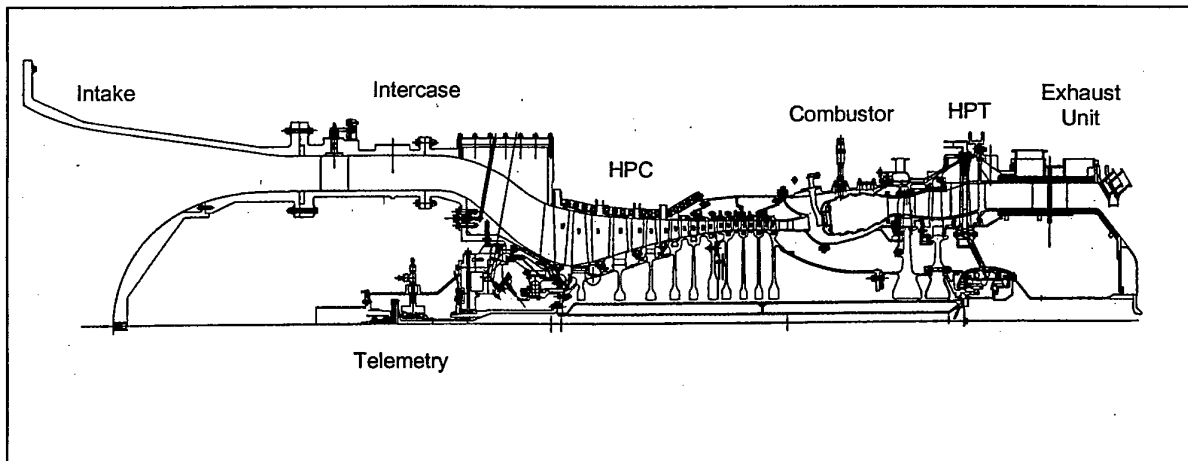
Figure 4: Cross-section of BR700 Core Engine Demonstrator
