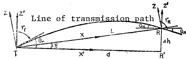
Figure 2. Plane Geometrical Path Relationships
