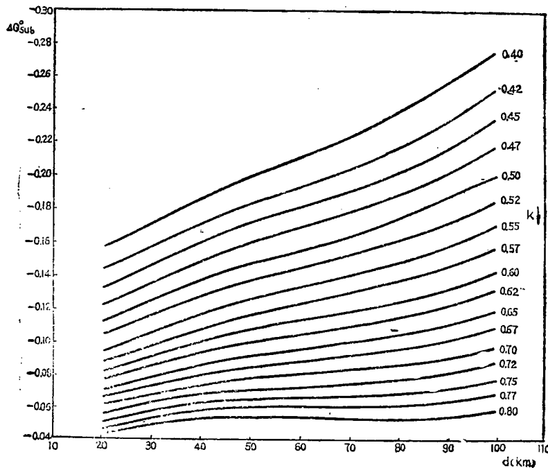
Figure 3. Graphs of the Relationship Between the Relative \Delta\theta_{sub} and d With the Point K Factor as Parameter
