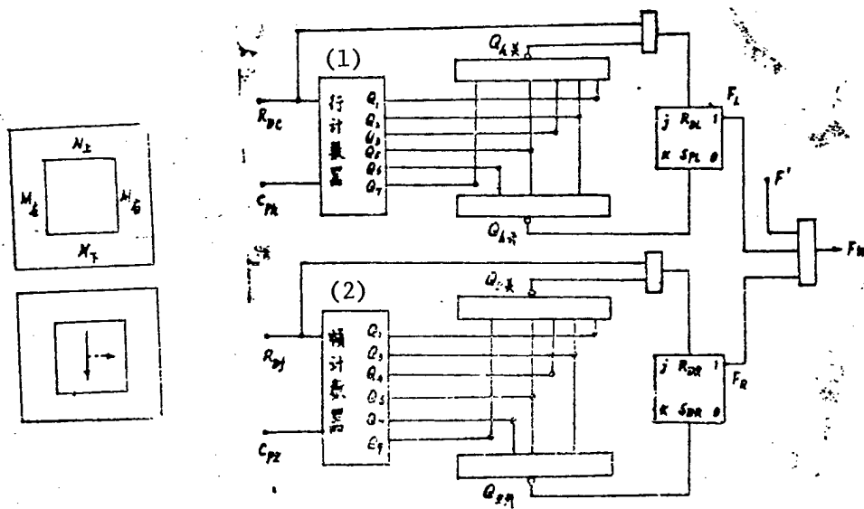
Figure 10. Sampling Window Forming Circuit
