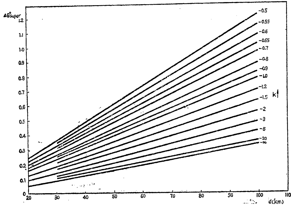
Figure 4. Graphs of the Relationship Between the Relative \Delta\theta_{\text{super}} and d With the Point K Factor as Parameter
