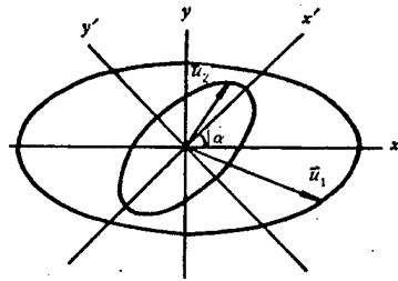
Figure 1. Tide Flow Ellipse
