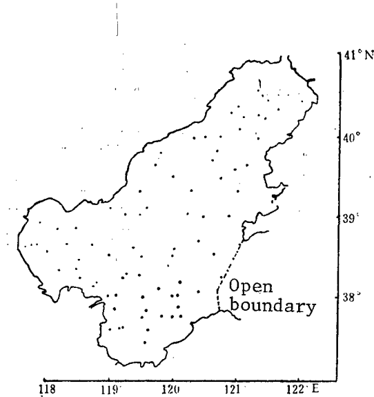
Figure 2. Bohai Sea Station Map
