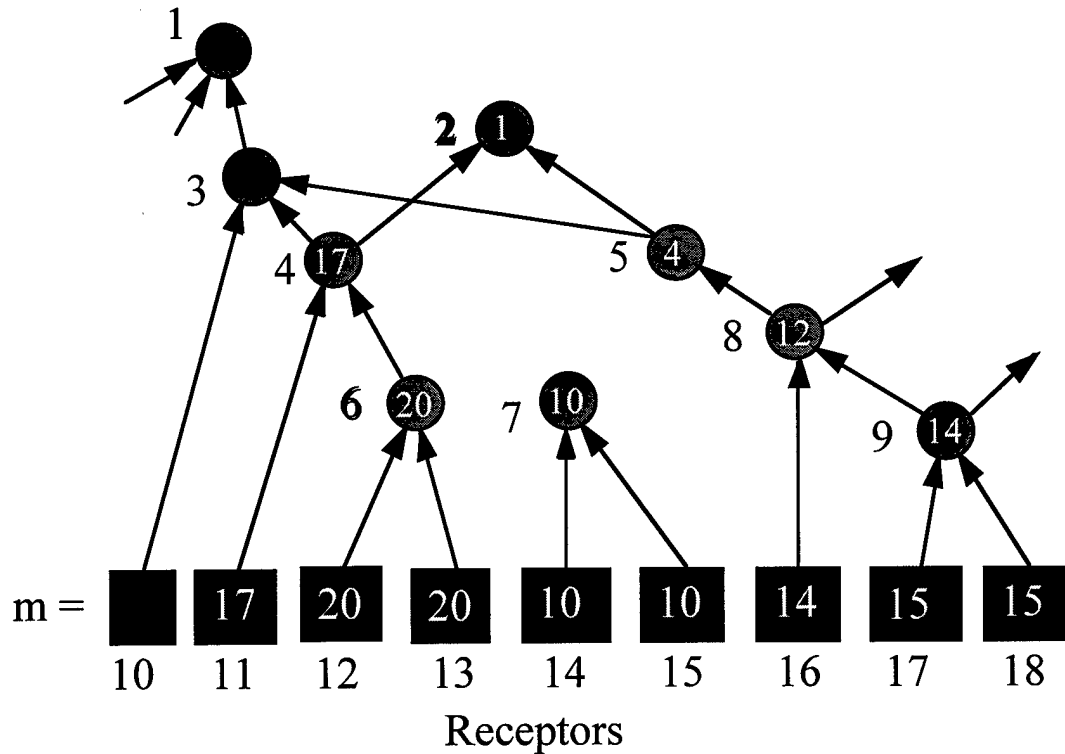
Figure 2. Determining Check Vertices in a Pyramidal Network
