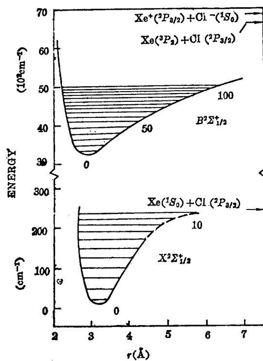
Figure 1. Potential curves of B 2 Σ 1/2 and X 2 Σ 1/2 of the XeCl excimer
