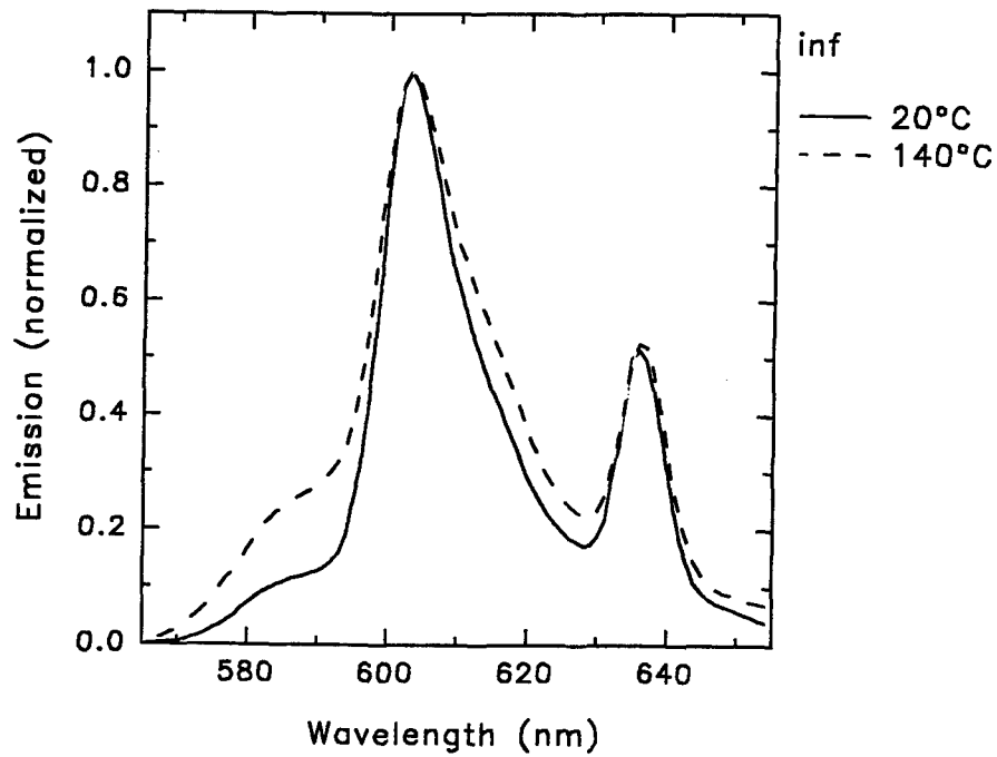
Figure 4. \text{Pr}^{3+} emission in fluoroaluminate (alf) and fluoroindate (inf) glasses: solid - at 20°C, dashed - at 140°C.
