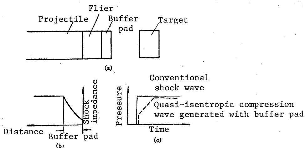
Figure 6. Generation of Quasi-Isentropic Compression With a Buffer Pad (a) Schematics of the device; (b) Shock impedance changes of the flier and buffer material; (c) Compression waveform at the interface
