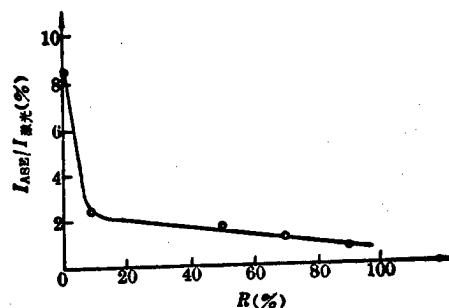
Fig. 6. Relationship of ASE background and output mirror reflectivity
