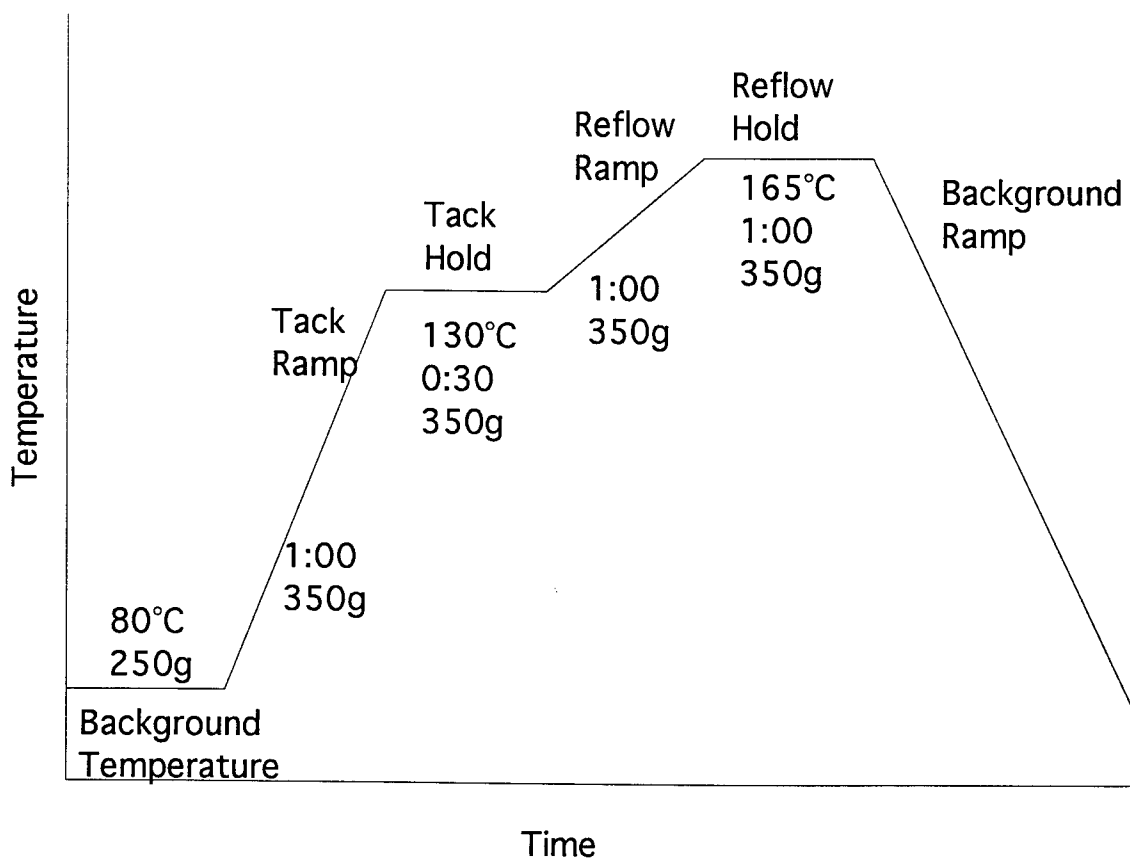
Figure 6. Bonding Parameters
