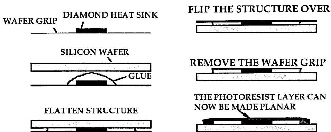
Figure 2. Encapsulation technique
