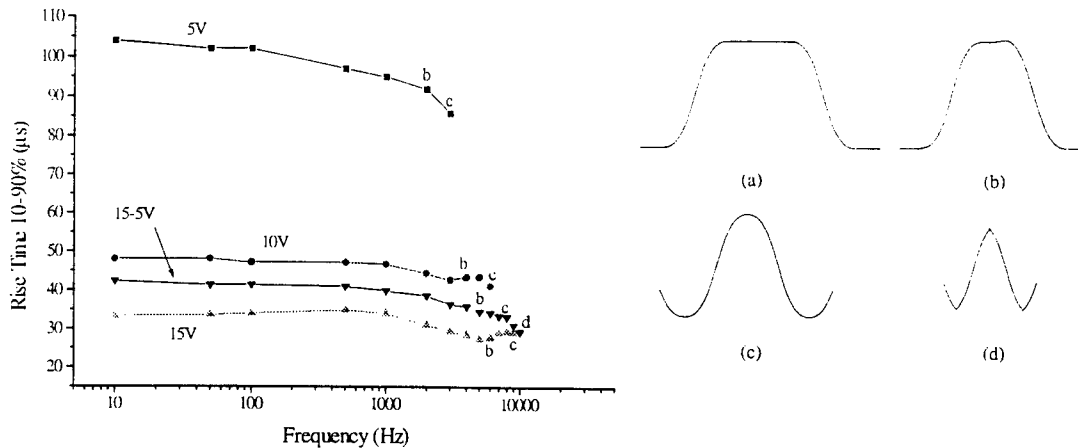
Figure 3: The 15-5V points represent the \pm 15-5 V waveform from the DR50 driver. The 5V, 10V and 15V points represent the \pm 5 , \pm 10 and \pm 15 V square wave points. As the frequency increases, the wave form of the optical output changes from a relatively square wave (a) to a triangular wave (d).
