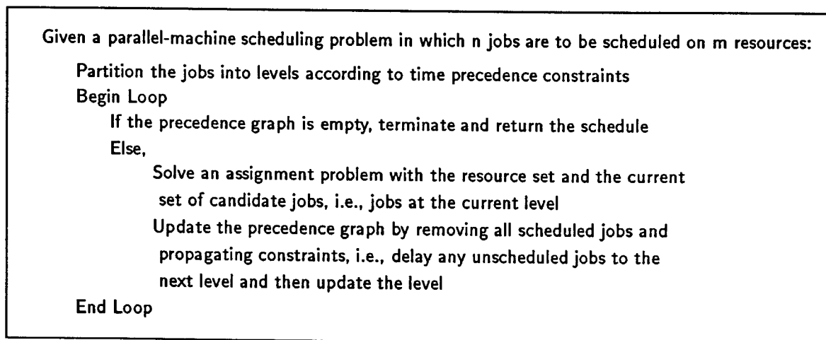
Figure 6: The Assignment Based Algorithm
