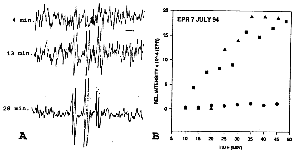
Figure 6. The EPR/spin trapping spectra over time (6A) and (6B) graph of 10 \mu L NaOH with 1 M ADN in .02 M PBN
