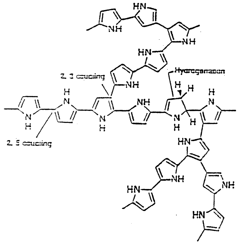
Proposed disordered structural model for polypyrrole
