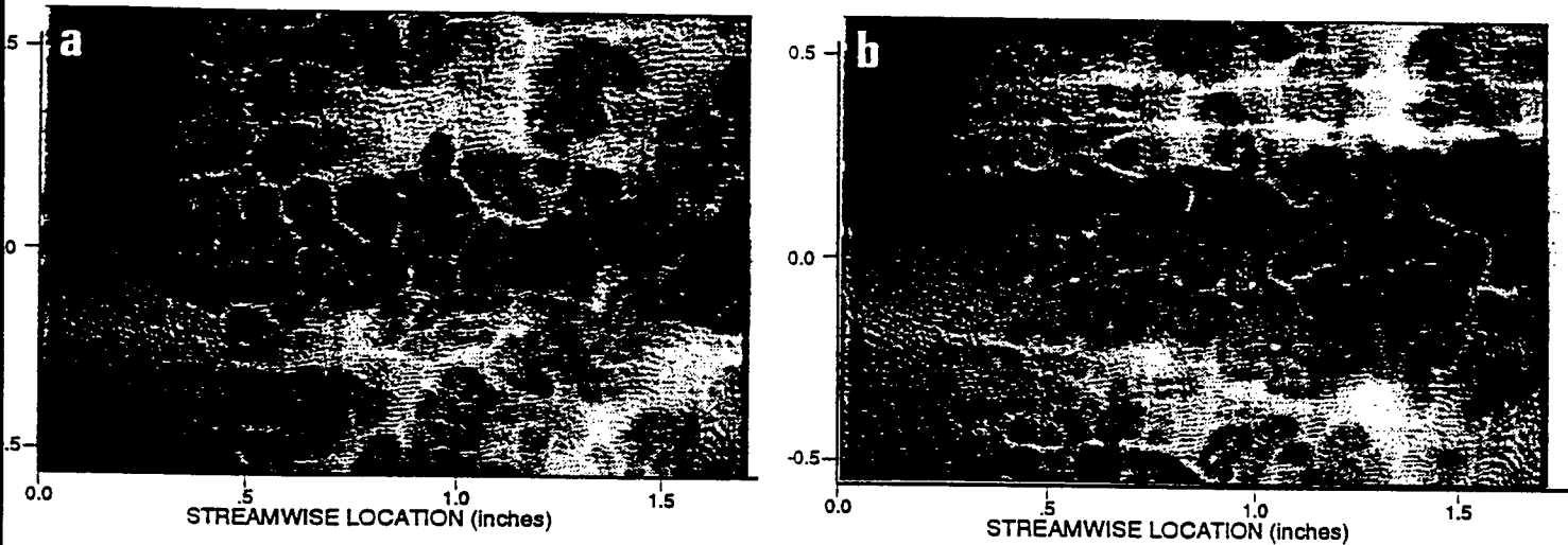
Figure 10 Face-on Mie scattering images a) pressure matched b) 4x pressure case
