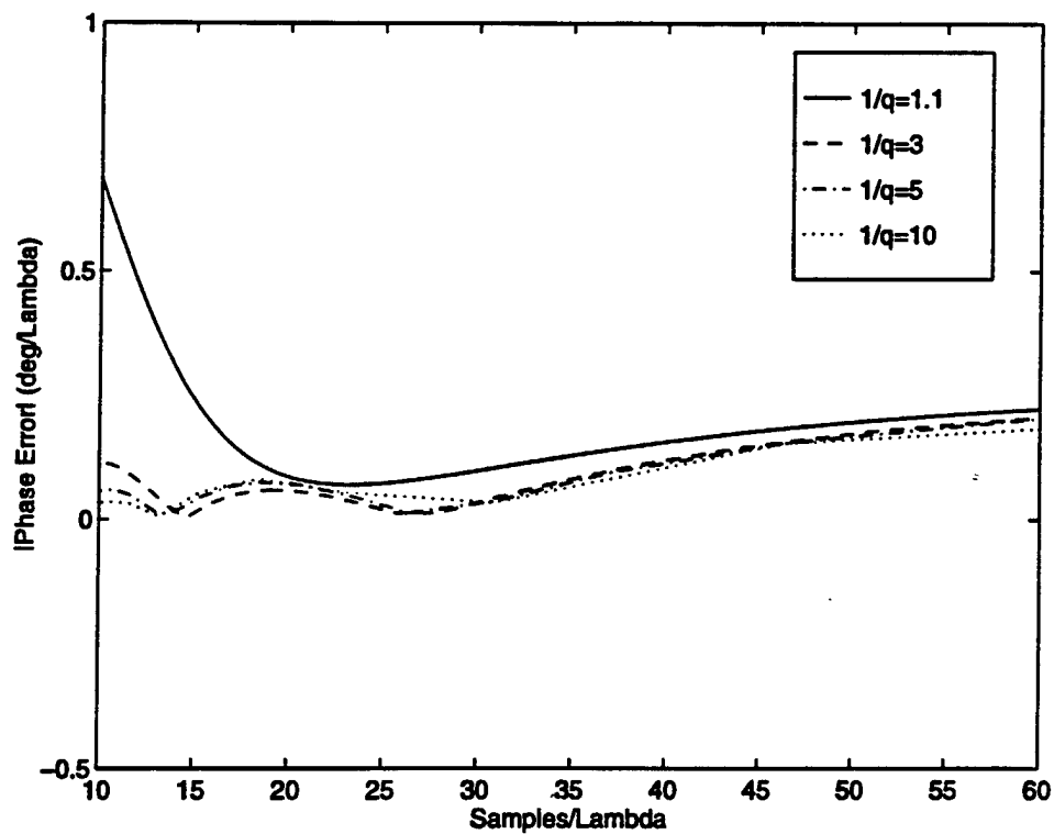
Figure 16: Effect of the Courant Number on the Dispersion Characteristics of W_0 - MRTD for n_a = n_b = n_c = 12 (Coarse Grid).
