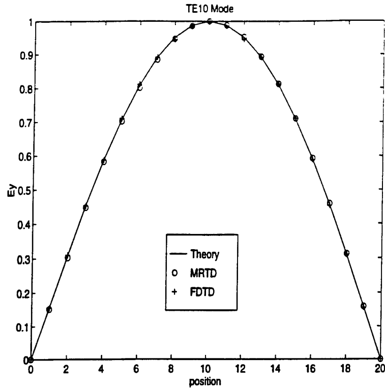
Figure 4.2: Shield TE_{10} E_y pattern.
