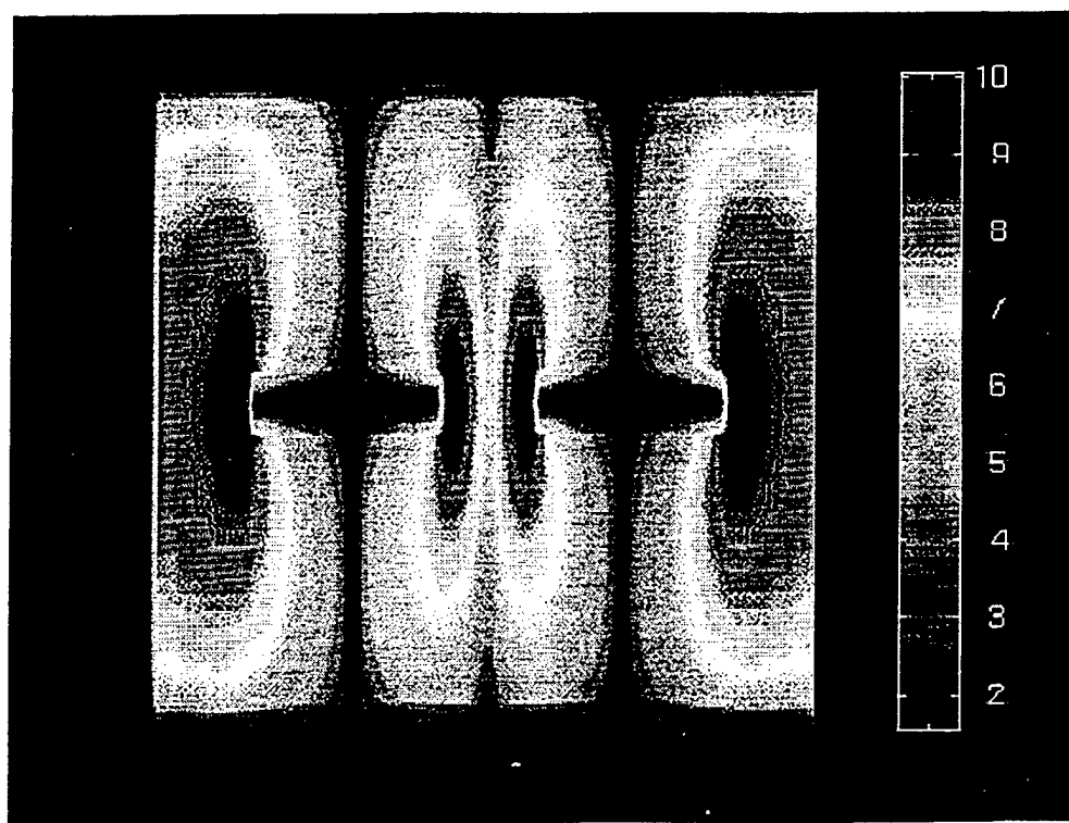
Figure 4.5: Tangential E-field Distribution (Shielded - Even Mode).
