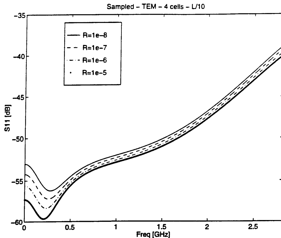
Figure 4.6: 4 PML cells - Non-split formulation - Dense Grid.
