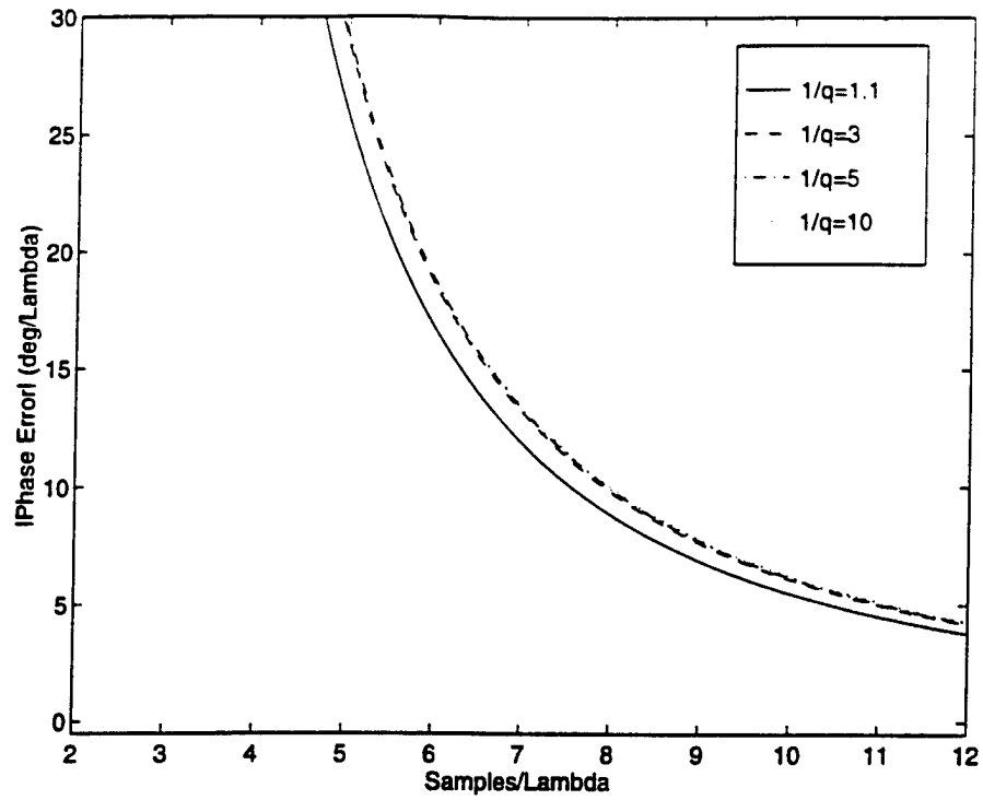
Figure 5.18: Effect of the Courant Number on the Dispersion Characteristics of FDTD (Coarse Grid).
