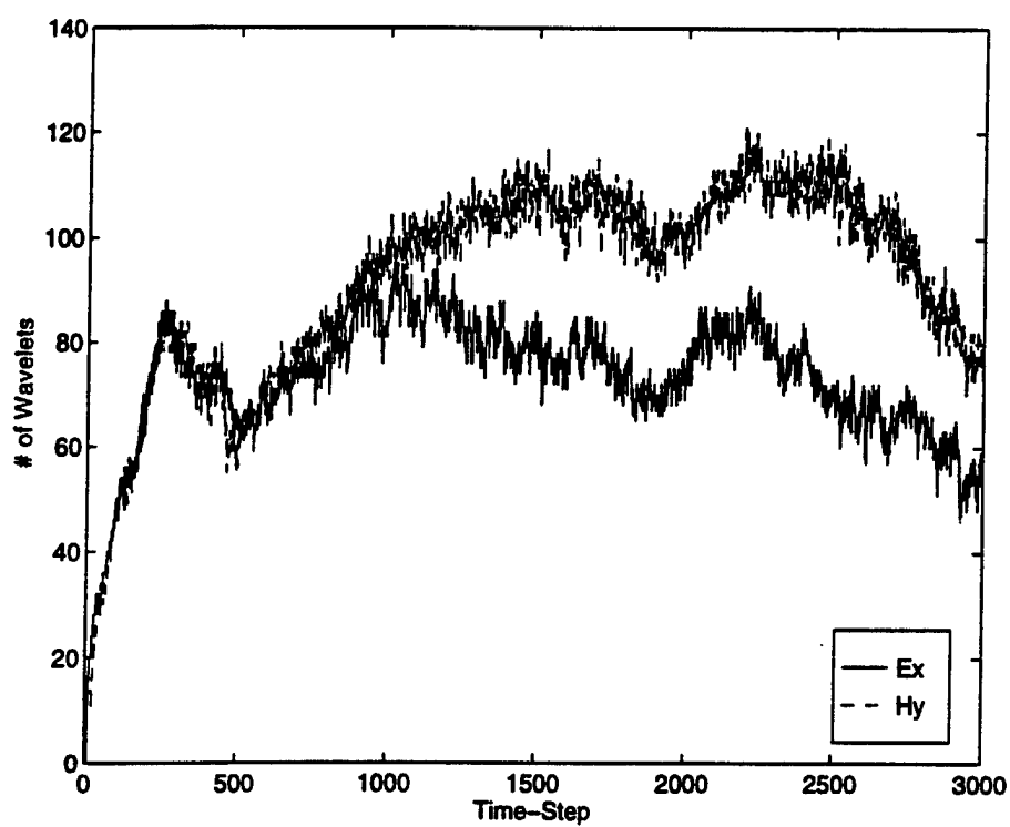
Figure 6.2: Normal E-field (Time-Domain).
