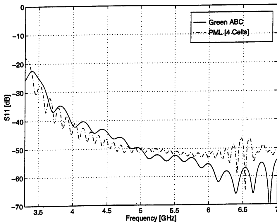
Figure 2.15: Comparison of Green's Function ABC and PML.
