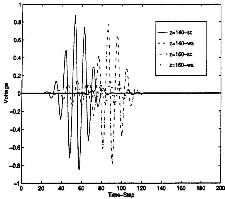
Figure 7: Voltage Coefficients.
