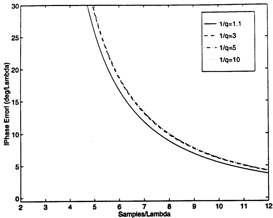
Figure 18: Effect of the Courant Number on the Dispersion Characteristics of FDTD (Coarse Grid).
