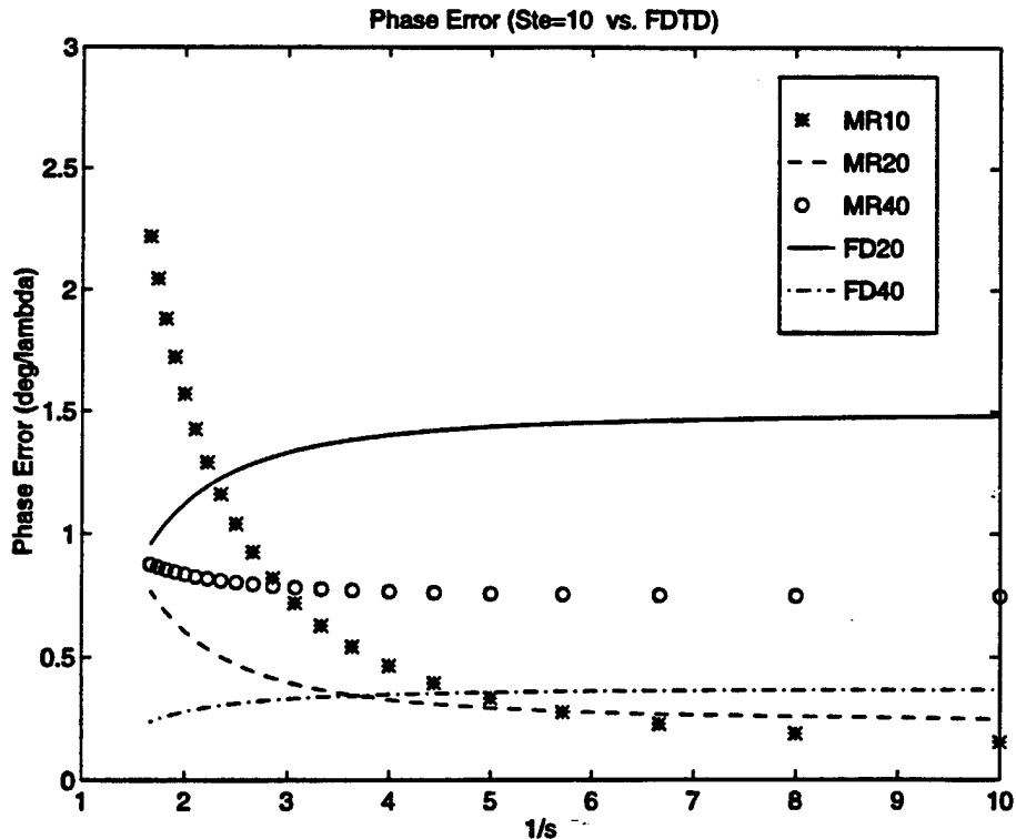
Figure 3: Dispersion Characteristics of S-MRTD for n_a=10 .
