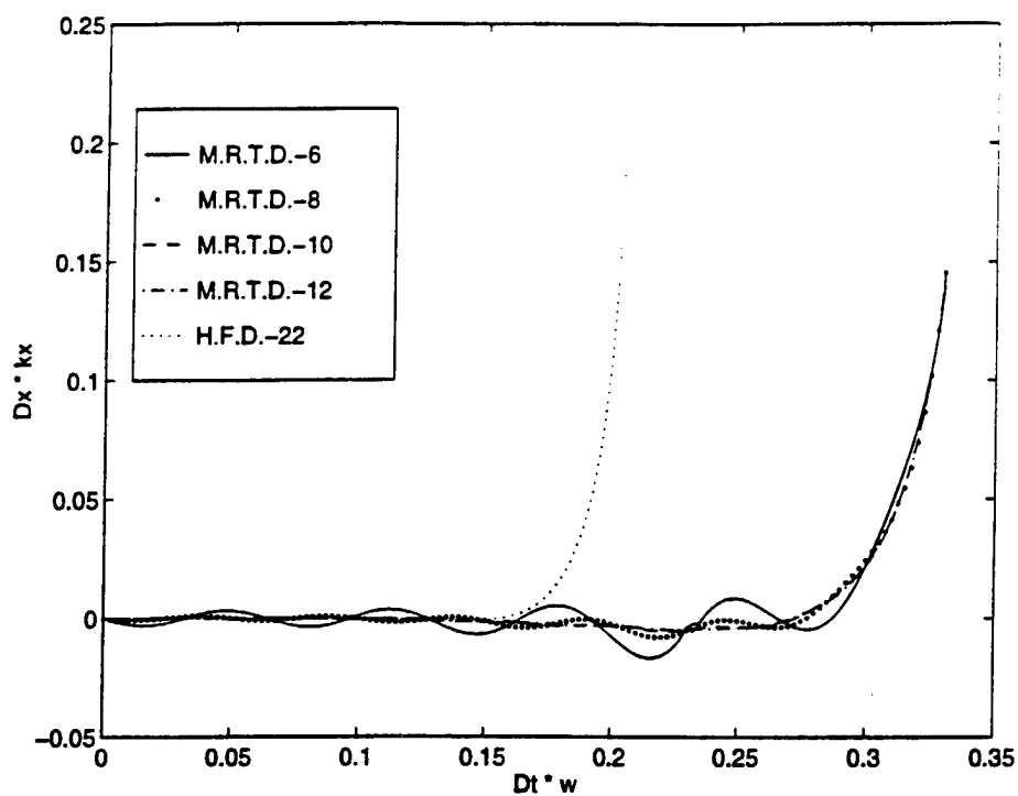
Figure 5.22: Comparison of the Oscillations of Wo-MRTD Scheme for Different Stencil Size.
