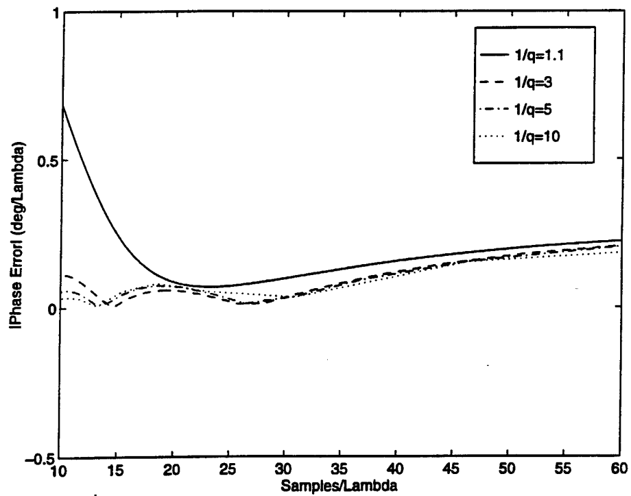
Figure 5.17: Effect of the Courant Number on the Dispersion Characteristics of W_0 - MRTD for n_a = n_b = n_c = 12 (Denser Grid).
