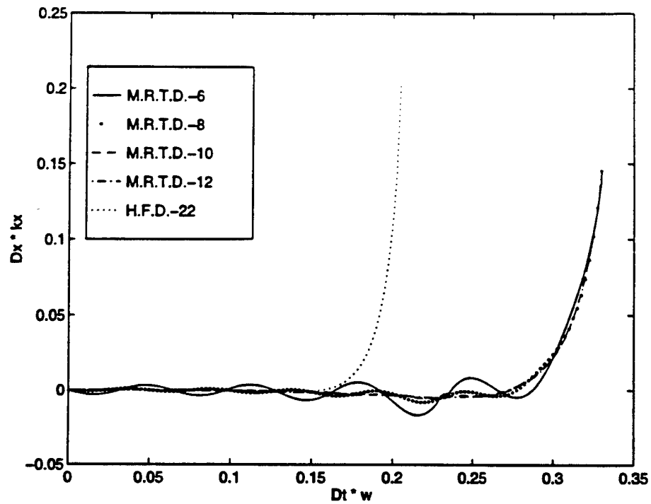
Figure 22: Comparison of the Oscillations of Wo-MRTD Scheme for Different Stencil Size.
