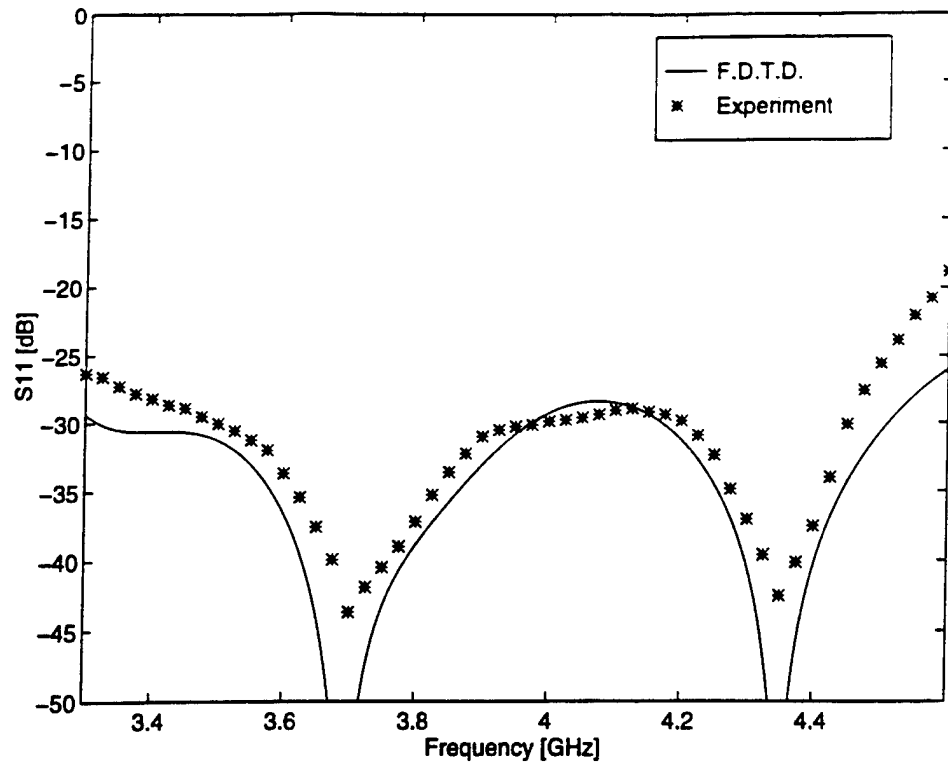
Figure 2.22: Experimental Validation for S_{11} .
