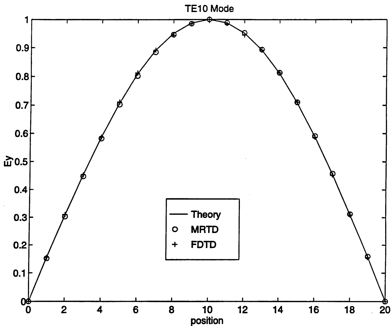
Figure 2: Shield TE 10 E_y pattern.
