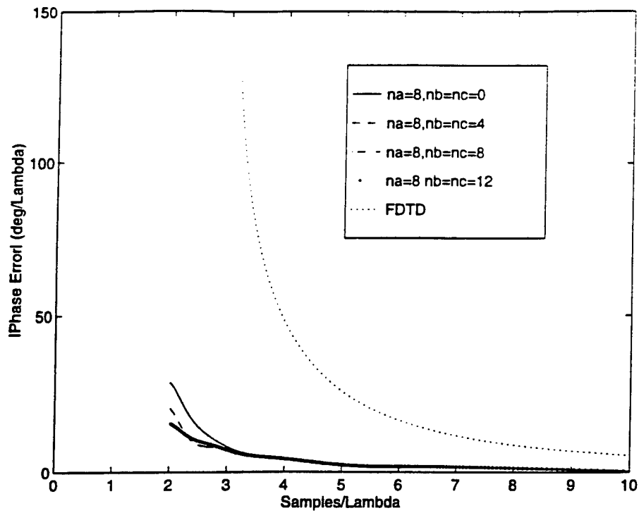
Figure 5.8: Wavelets Effect on the Dispersion Characteristics of MRTD for n_a=8 (Coarse Grid).
