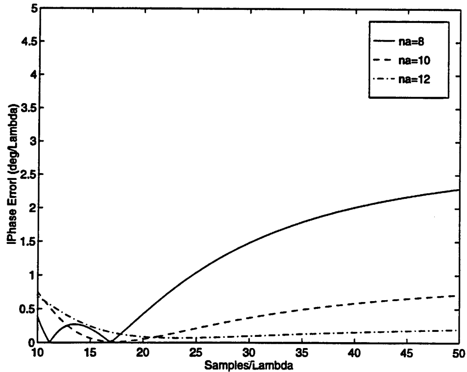
Figure 6: Stencil Effect on the Dispersion Characteristics of S-MRTD (Sparse Grid).
