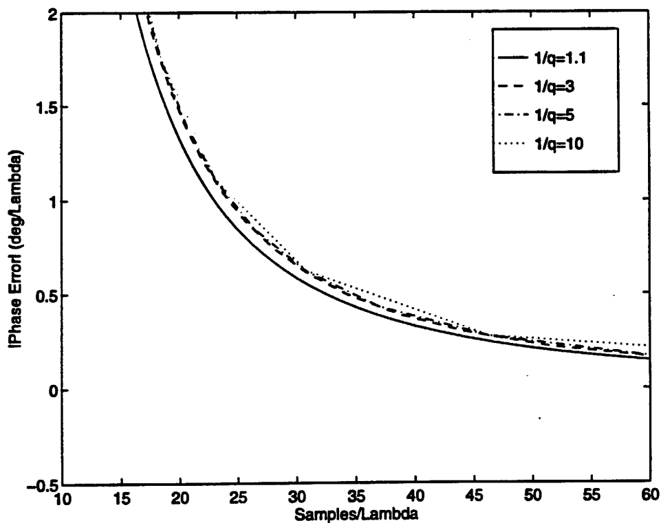
Figure 18: Effect of the Courant Number on the Dispersion Characteristics of FDTD (Coarse Grid).
