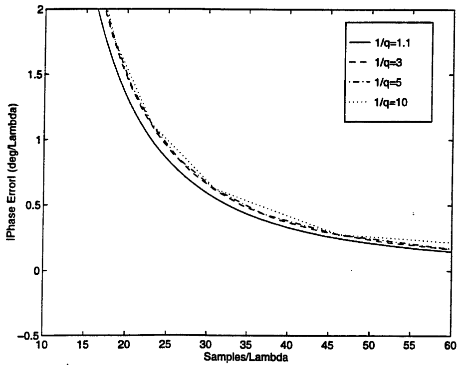
Figure 5.19: Effect of the Courant Number on the Dispersion Characteristics of FDTD (Denser Grid).
