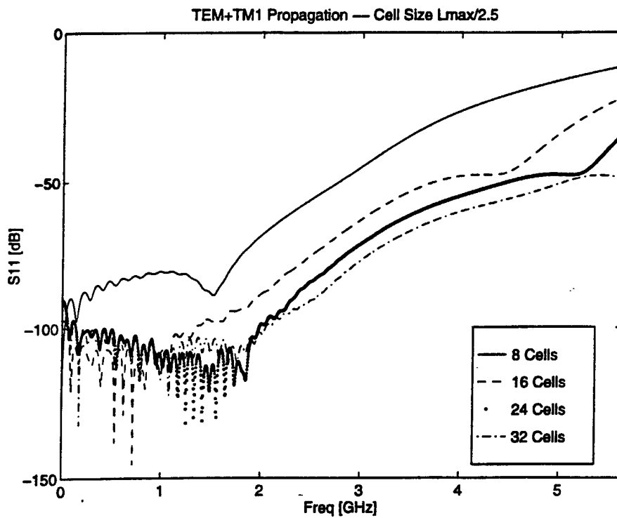
Figure 4.11: Multimodal Propagation - Coarse Grid.
