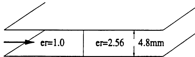
Figure 1: Dielectric-loaded Waveguide.
