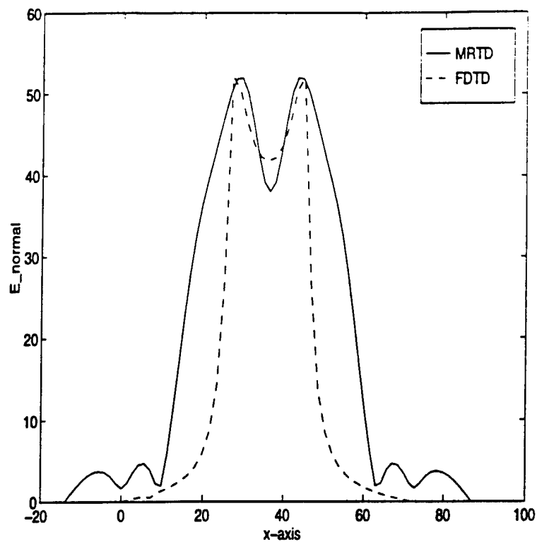
Figure 4.4: TEM E_y Pattern Comparison (8x8 Grid).
