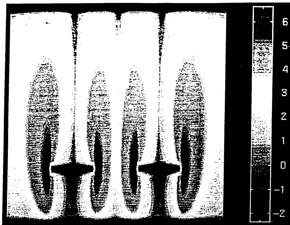
Figure 4.16: Tangential E-field Distribution (Open - Even Mode).
