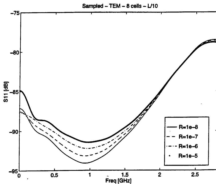
Figure 4.7: 8 PML cells - Non-split formulation - Dense Grid.
