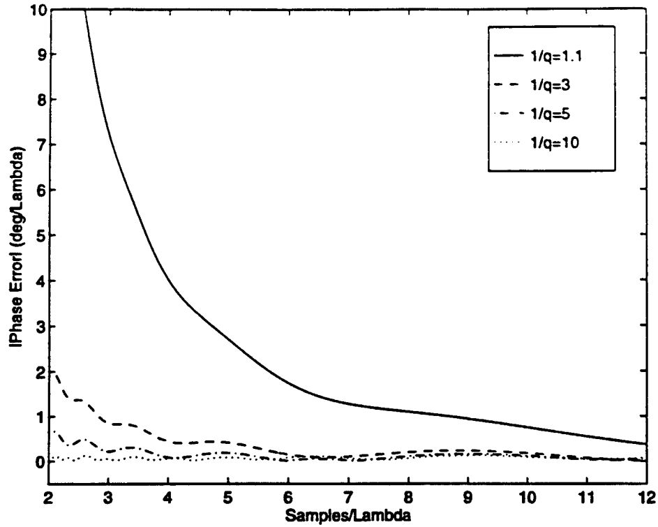
Figure 14: Effect of the Courant Number on the Dispersion Characteristics of W_0 - MRTD for n_a = n_b = n_c = 10 (Coarse Grid).
