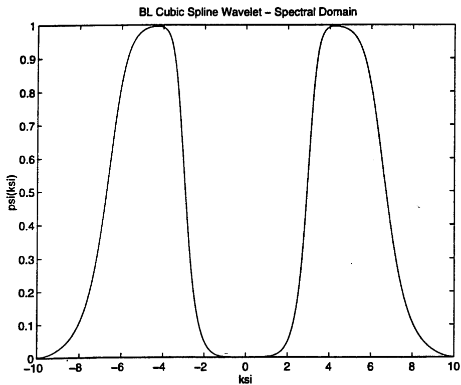
Figure 3.4: BL Cubic Spline Wavelet - Spectral Domain.
