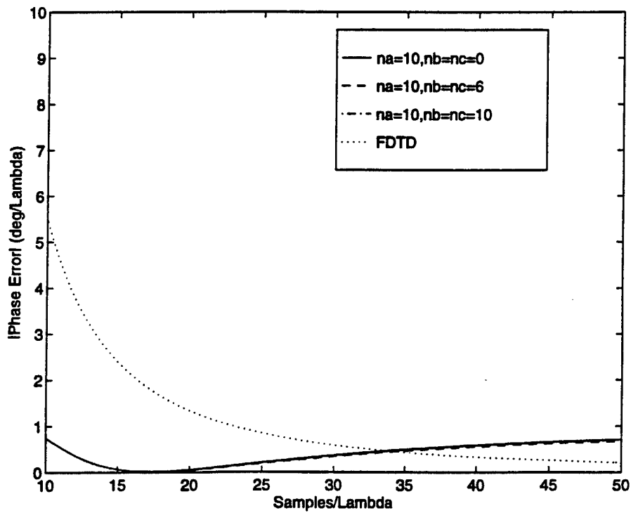
Figure 5.11: Wavelets Effect on the Dispersion Characteristics of MRTD for n_a=10 (Denser Grid).
