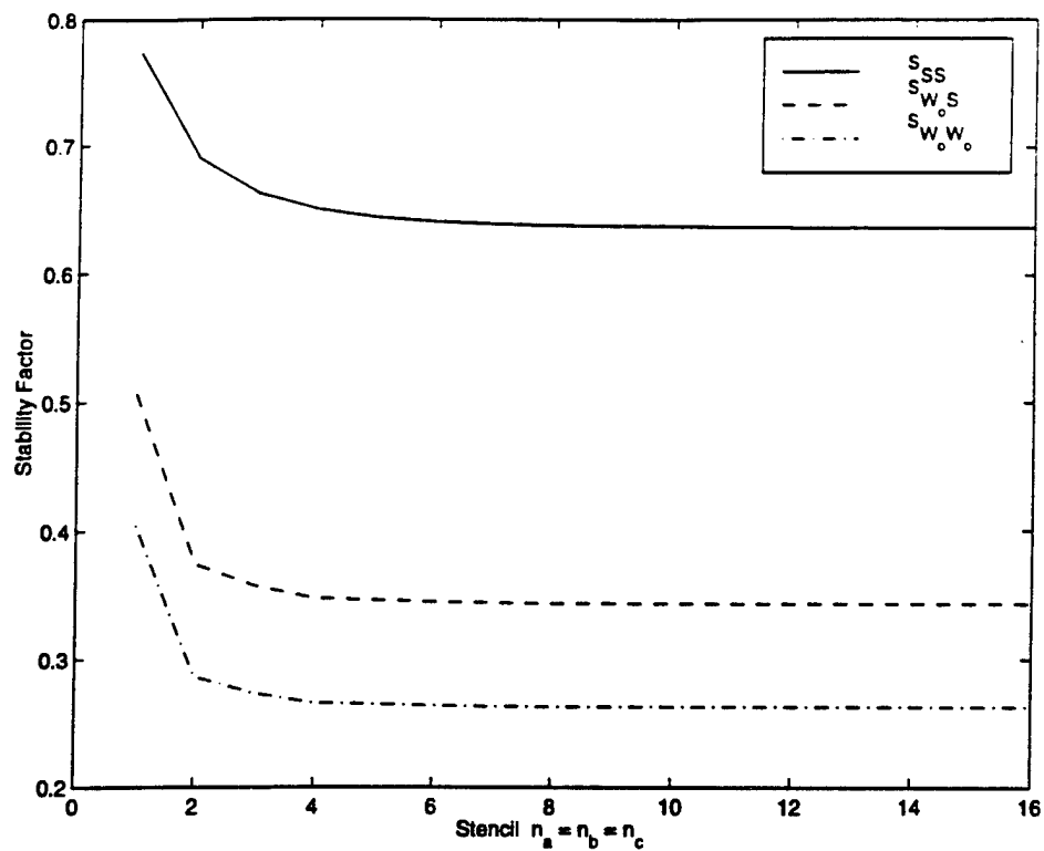
Figure 5.1: Stability Parameter s for MRTD.
