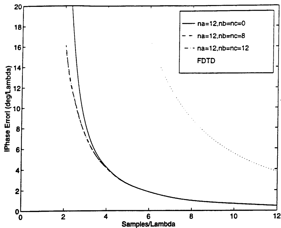
Figure 5.12: Wavelets Effect on the Dispersion Characteristics of MRTD for n_a=12 (Coarse Grid).
