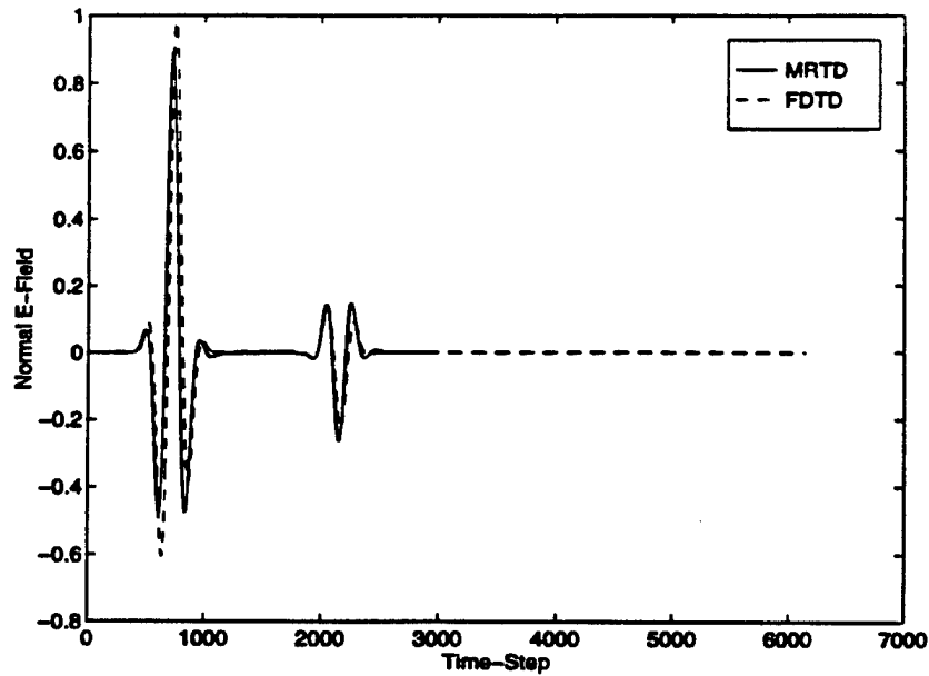
Figure 2: Normal E-field Time Evolution.
