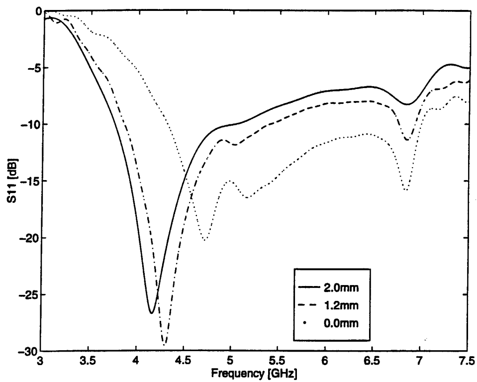
Figure 2.17: Reflection Coefficient for different Dielectric Thicknesses.
