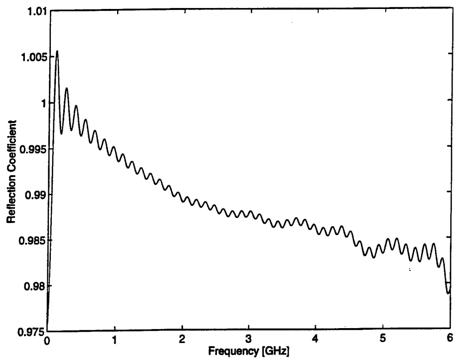
Figure 2.3: Reflection Coefficient of the Open.
