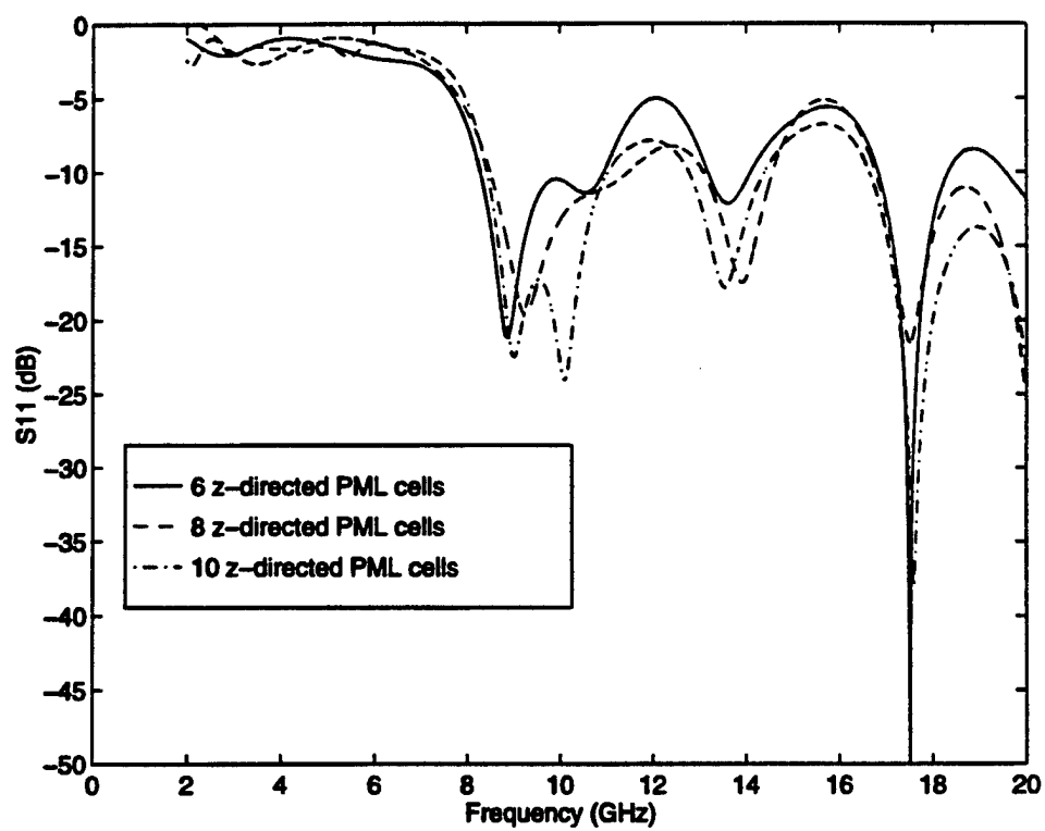
Figure 5: MRTD( 20 \times 20 \times 9 ) S_{11} plot for varying PML layers in the z-direction
