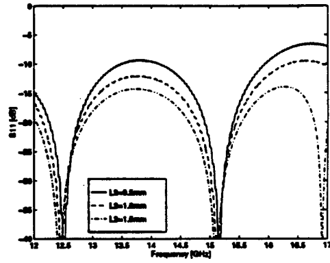
Figure 6: Parametric Variation of l_2 .
