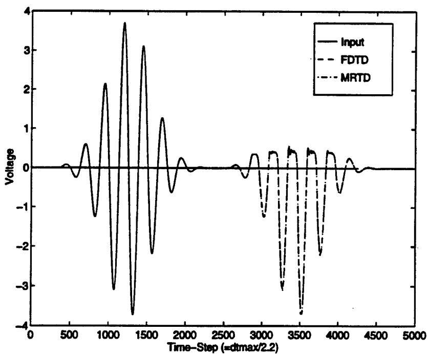
Figure 10: Comparison MRTD-FDTD.
