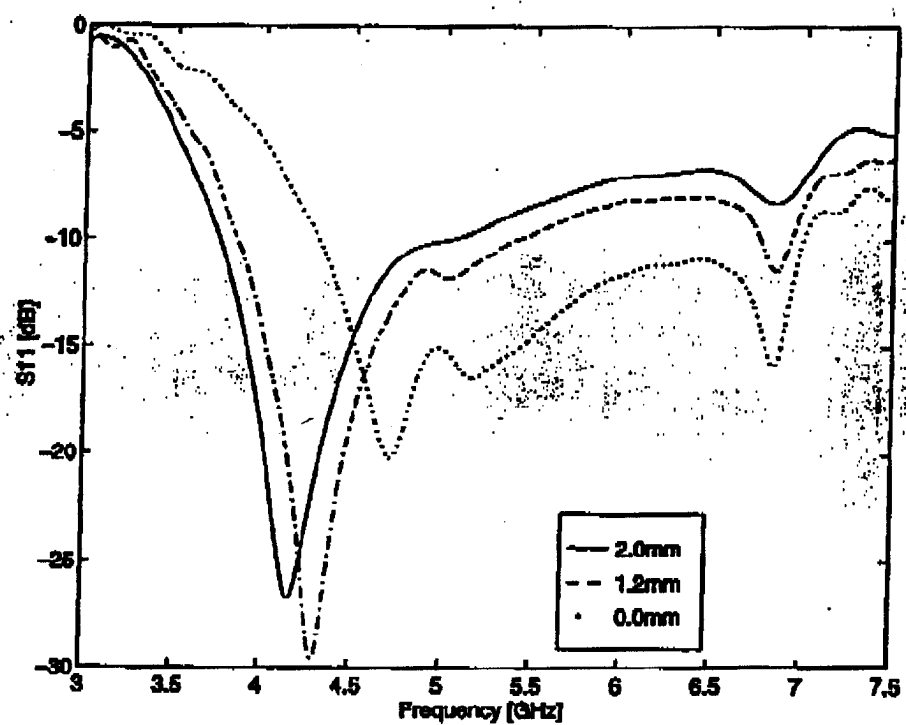
Figure 2.17: Reflection Coefficient for different Dielectric Thicknesses.
