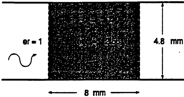
Figure 1: Dielectric-loaded Waveguide.
