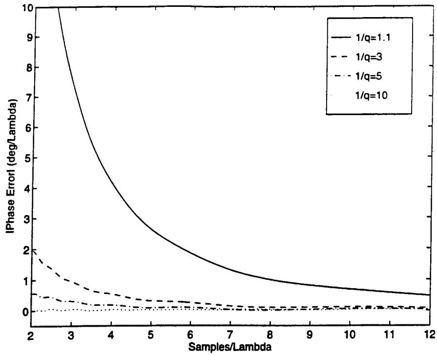
Figure 5.16: Effect of the Courant Number on the Dispersion Characteristics of W_0 - MRTD for n_a = n_b = n_c = 12 (Coarse Grid).
