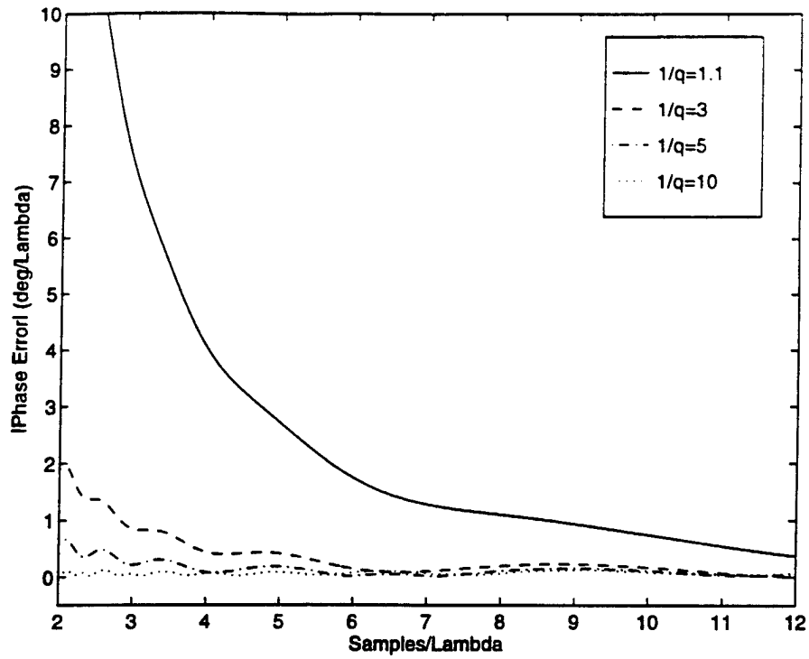
Figure 5.14: Effect of the Courant Number on the Dispersion Characteristics of W_0 - MRTD for n_a = n_b = n_c = 10 (Coarse Grid).
