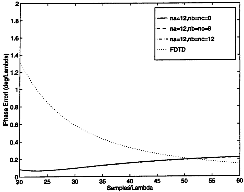
Figure 12: Wavelets Effect on the Dispersion Characteristics of MRTD for n_a=12 (Coarse Grid).
