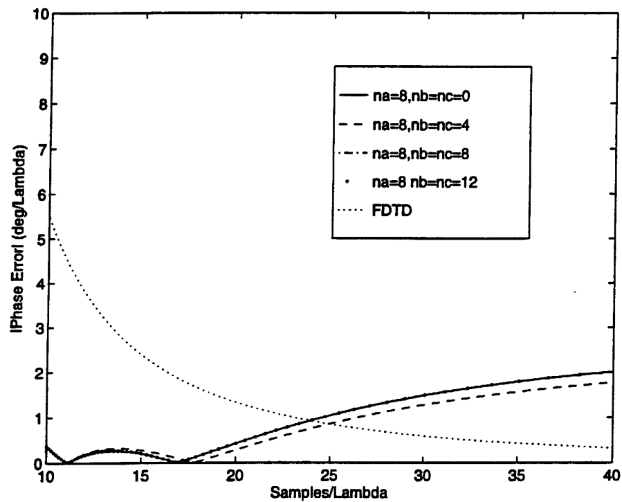
Figure 5.9: Wavelets Effect on the Dispersion Characteristics of MRTD for n_a=8 (Denser Grid).
