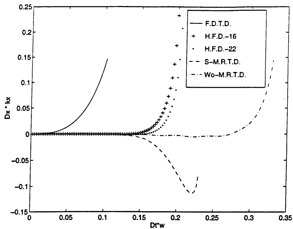
Figure 5.20: Comparison of the Dispersion Performance of S-MRTD and Wo-MRTD with Different Higher Order Yee's Schemes.
