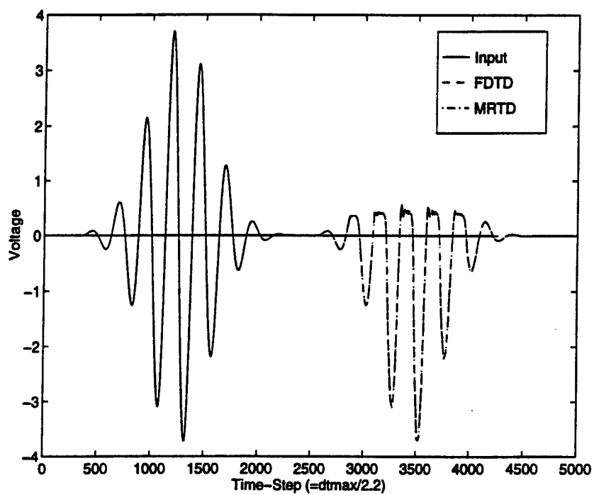
Figure 7.10: Comparison MRTD-FDTD.
