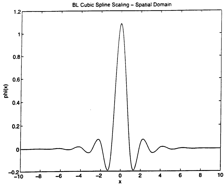
Figure 3.1: BL Cubic Spline Scaling - Spatial Domain.
