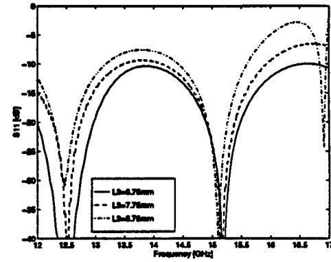
Figure 7: Parametric Variation of l_3 .
