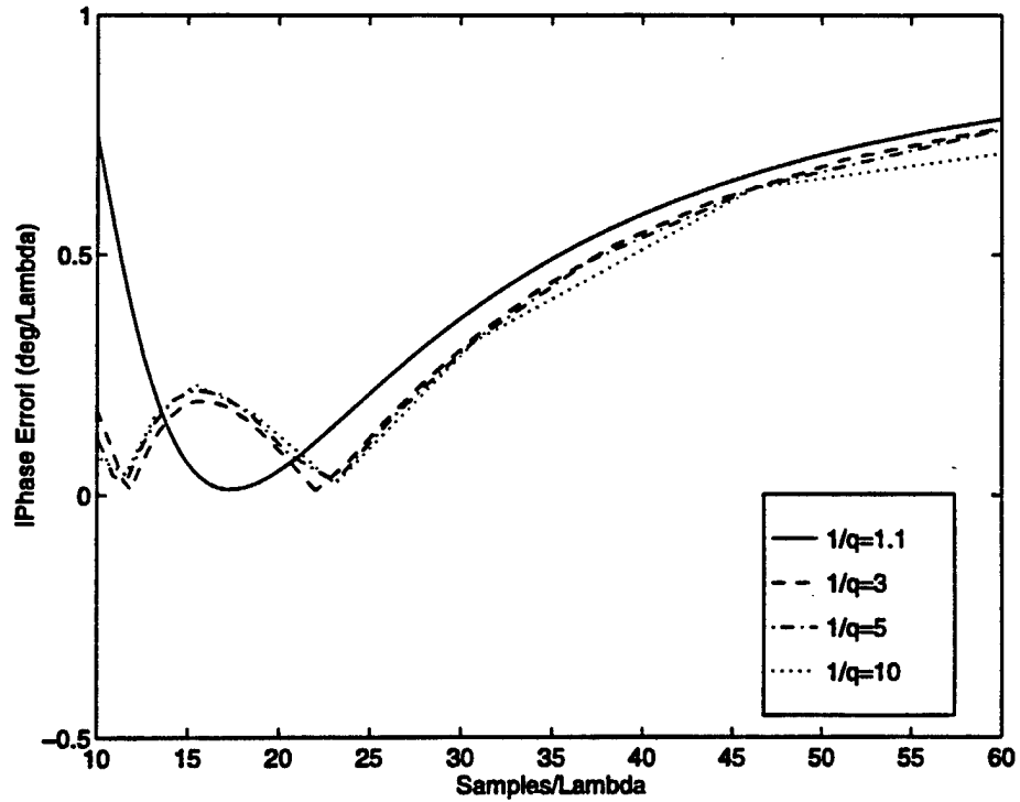
Figure 14: Effect of the Courant Number on the Dispersion Characteristics of W_0 - MRTD for n_a = n_b = n_c = 10 (Coarse Grid).
