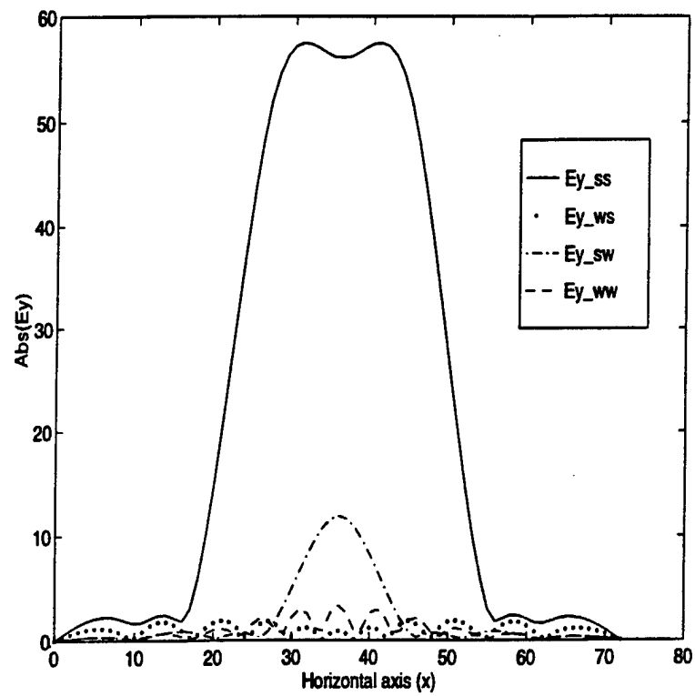
Figure 4.3: TEM E_y Pattern Components (8x8 Grid).
