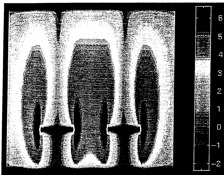
Figure 4.17: Tangential E-field Distribution (Open - Odd Mode).
