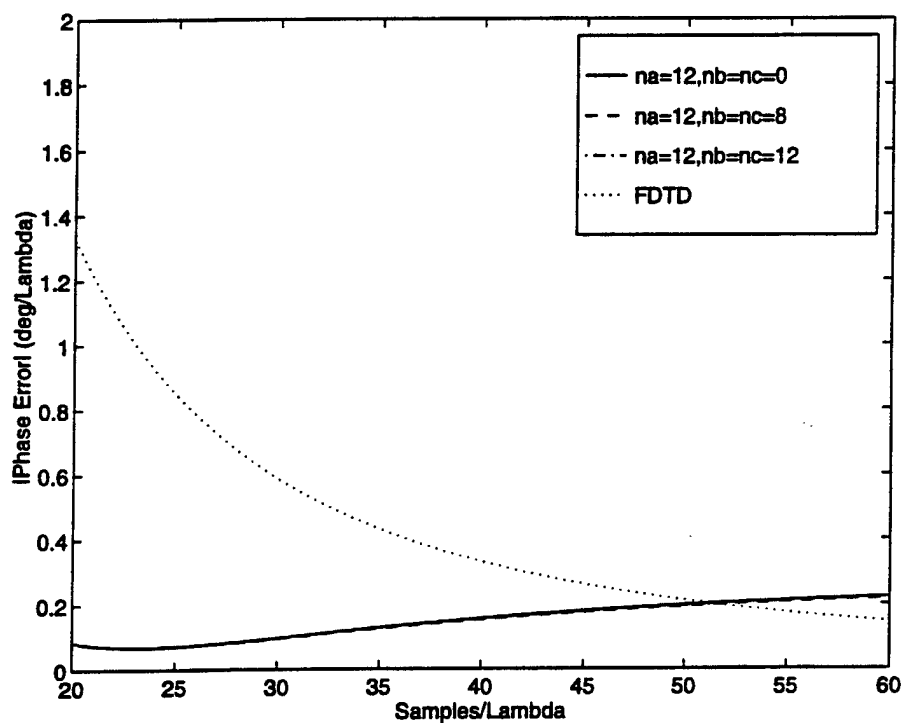
Figure 5.13: Wavelets Effect on the Dispersion Characteristics of MRTD for n_a=12 (Denser Grid).
