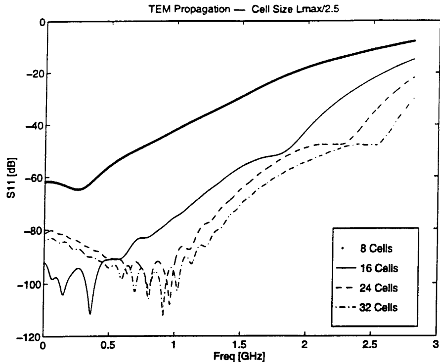
Figure 4.10: TEM Propagation - Coarse Grid.
