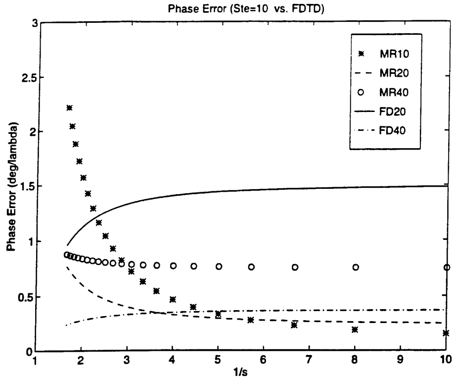
Figure 5.3: Dispersion Characteristics of S-MRTD for n_a=10 .
