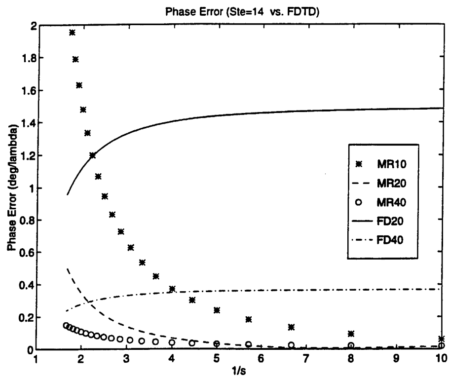
Figure 5.5: Dispersion Characteristics of S-MRTD for n_a=14 .
