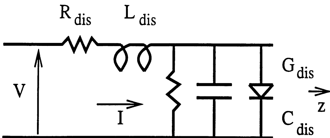
Figure 9: Rectifier Geometry.
