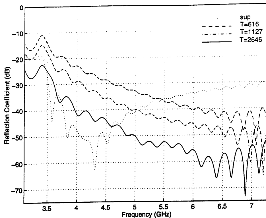
Figure 2.14: Reflection coefficient for the TE_{1,0}^z mode.
