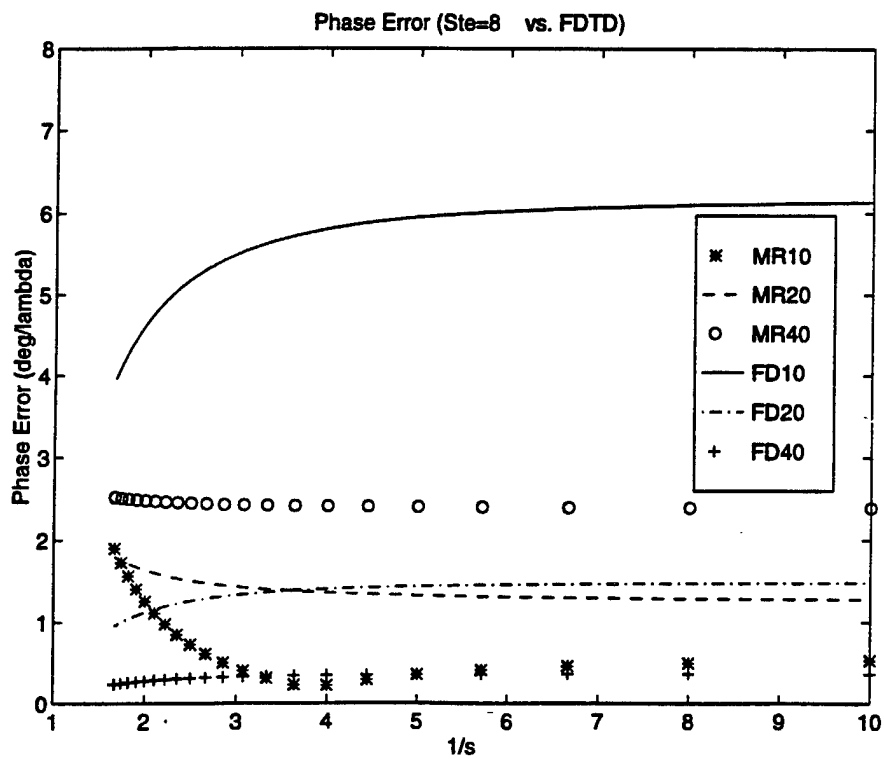
Figure 5.2: Dispersion Characteristics of S-MRTD for n_a=8 .
