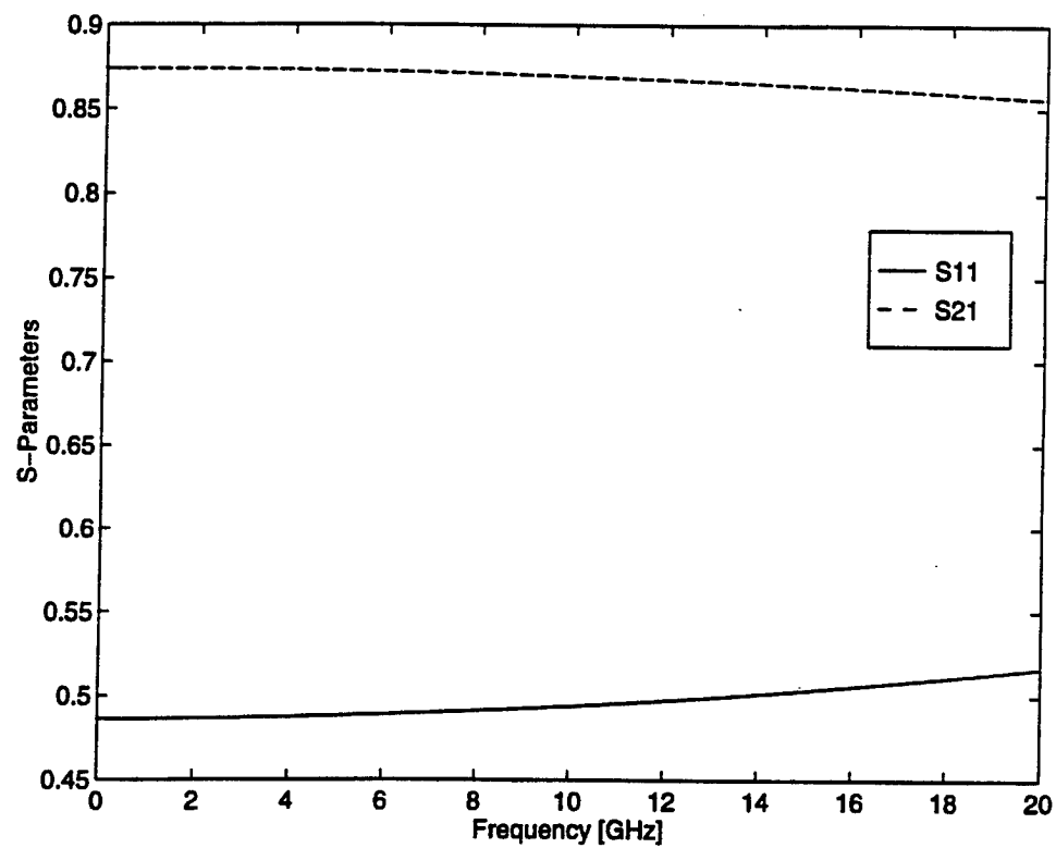
Figure 2.5: S-Parameters of the Viahole.
