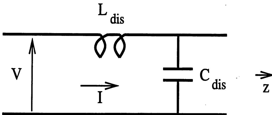
Figure 2: Ideal (Lossless) Transmission Line.
