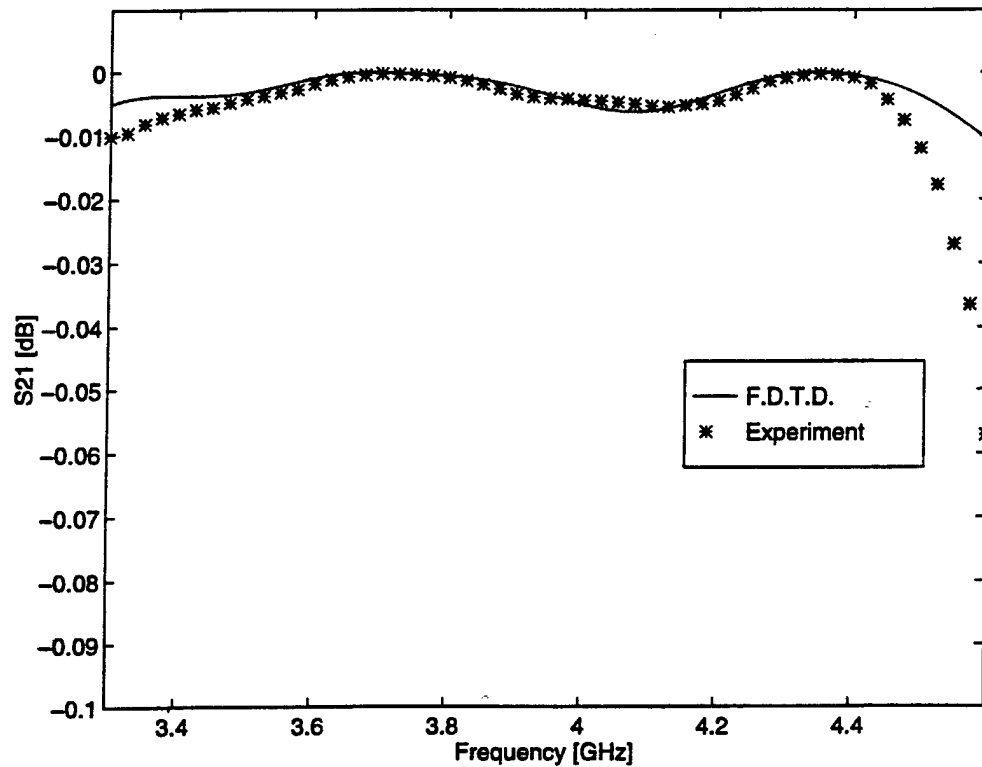
Figure 2.23: Experimental Validation for S_{21} .
