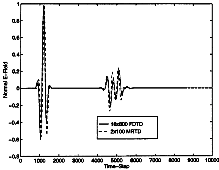
Figure 2: Normal E-field (Time-Domain).
