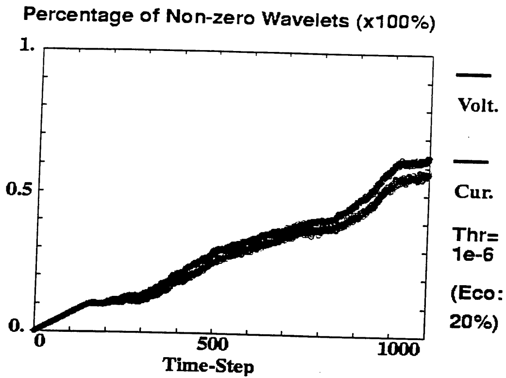
Figure 7.5: Fraction of Wavelets above Threshold.
