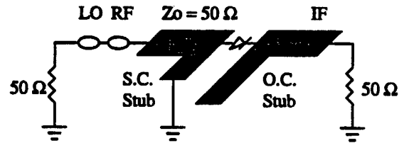
Figure 5: Mixer Geometry.
