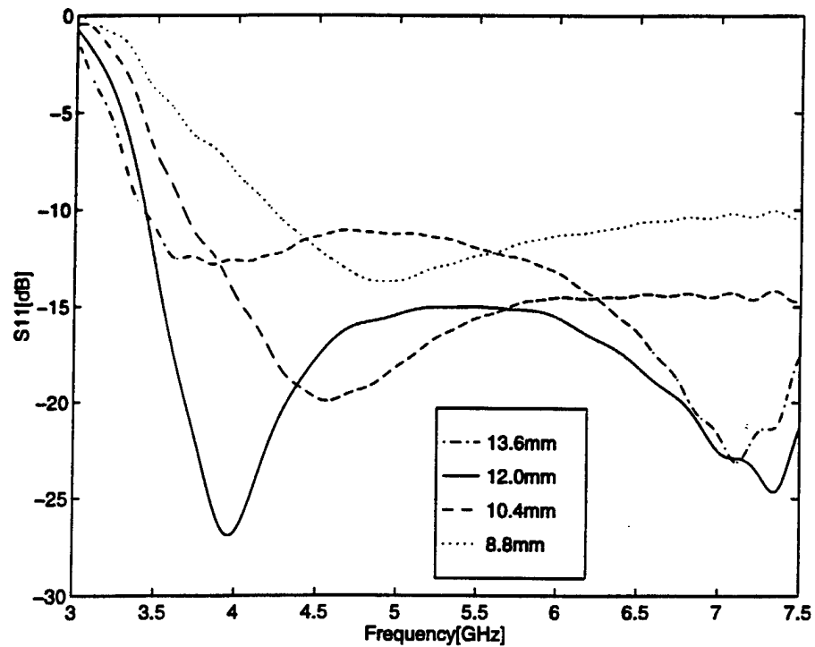
Figure 2.20: Reflection Coefficient for different Patch Widths.
