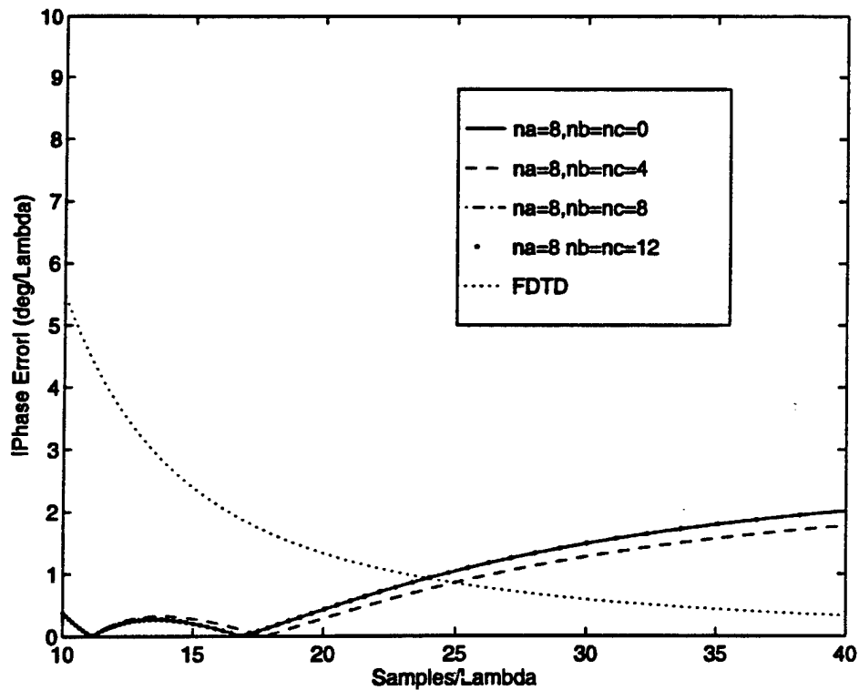
Figure 8: Wavelets Effect on the Dispersion Characteristics of MRTD for n_a=8 (Coarse Grid).
