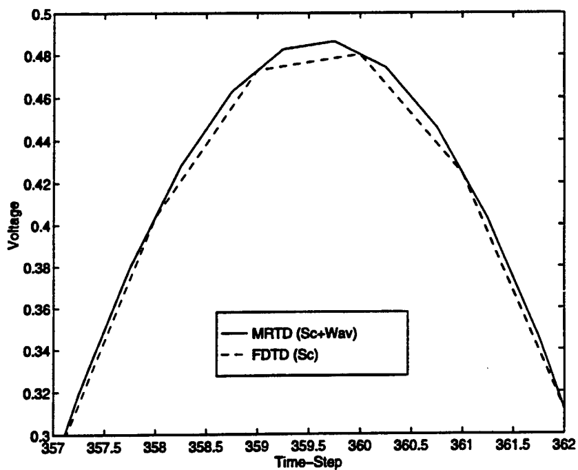
Figure 4: Comparison MRTD-FDTD.
