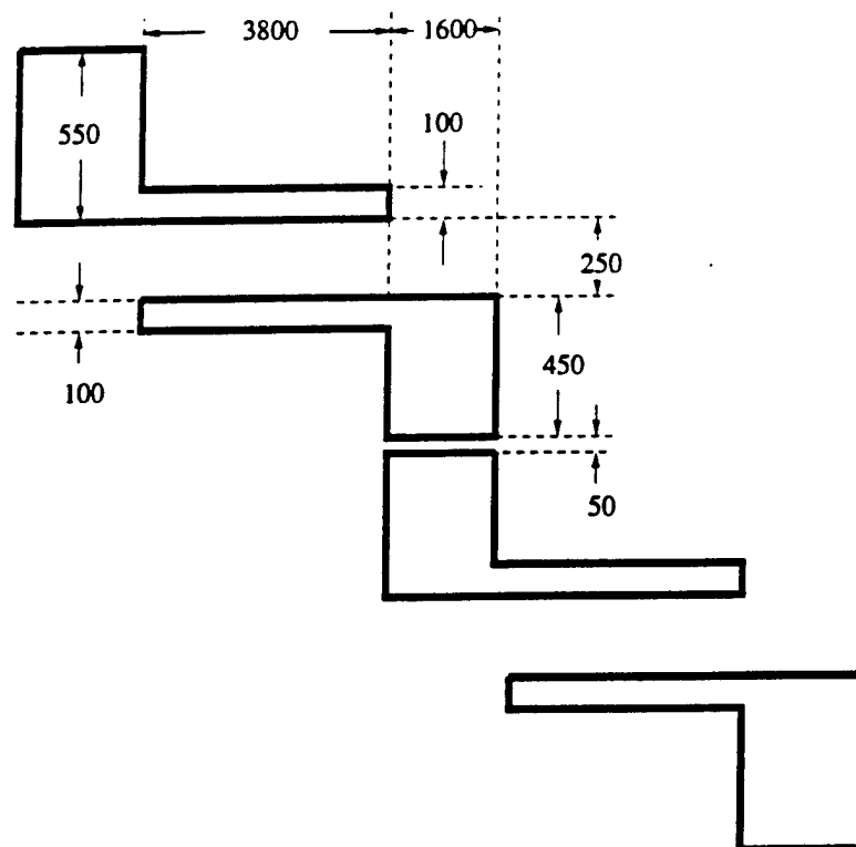
Figure 2.8: Coupled Line Filter Geometry.
