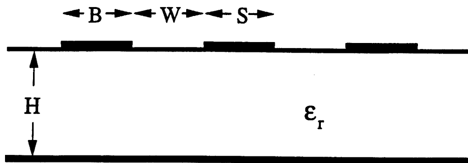
Figure 2.10: Coplanar waveguide with finite width ground planes (F.G.C.).
