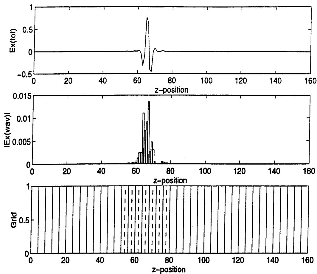
Figure 6.4: Adaptive Grid Demonstration ( t=1000 steps).
