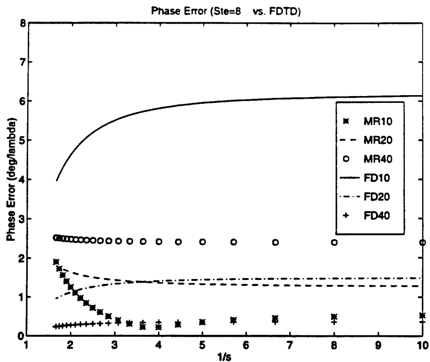
Figure 2: Dispersion Characteristics of S-MRTD for n_a=8 .
