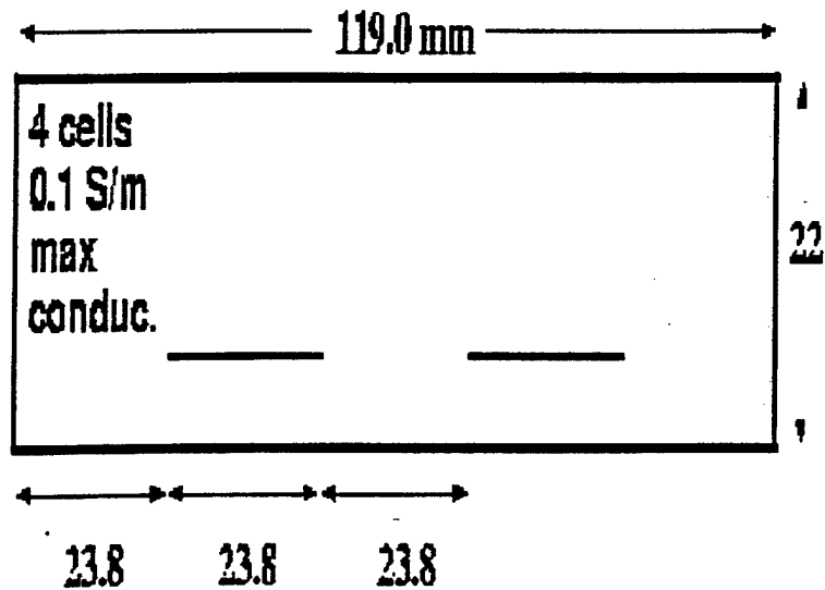
Figure 4.15: Open Coupled Stripline Geometry.
