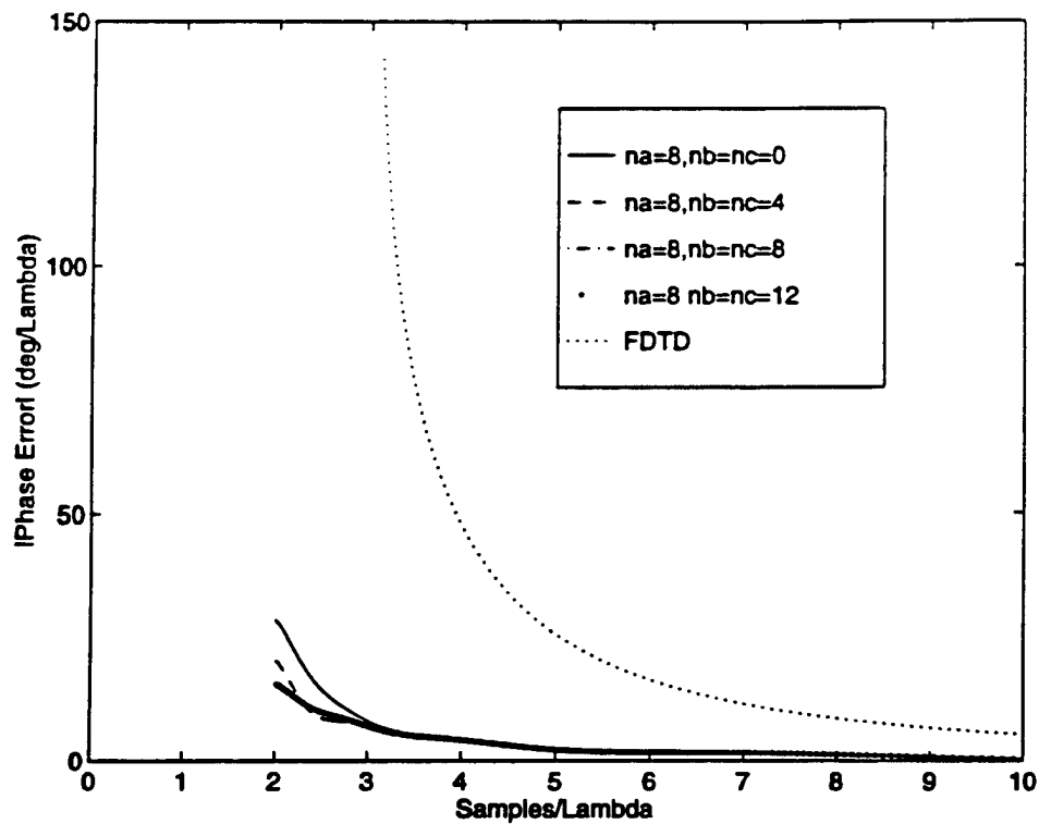
Figure 8: Wavelets Effect on the Dispersion Characteristics of MRTD for n_a=8 (Coarse Grid).
