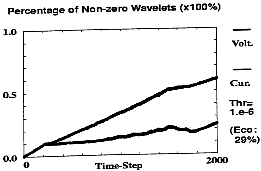
Figure 7.8: Fraction of Wavelets above Threshold.
