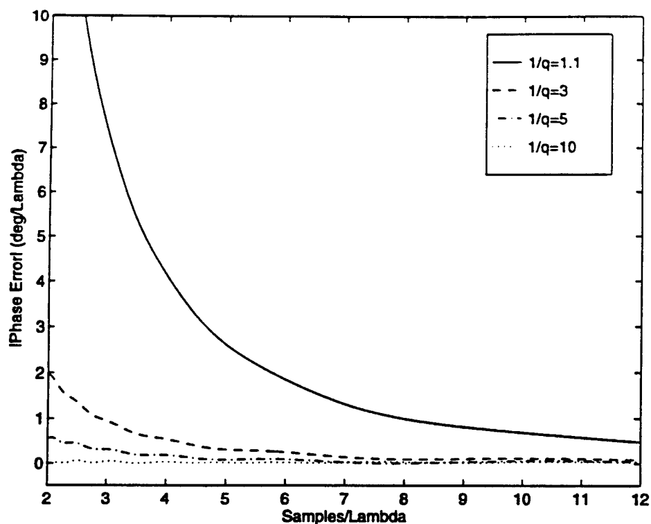
Figure 16: Effect of the Courant Number on the Dispersion Characteristics of W_0 - MRTD for n_a = n_b = n_c = 12 (Coarse Grid).
