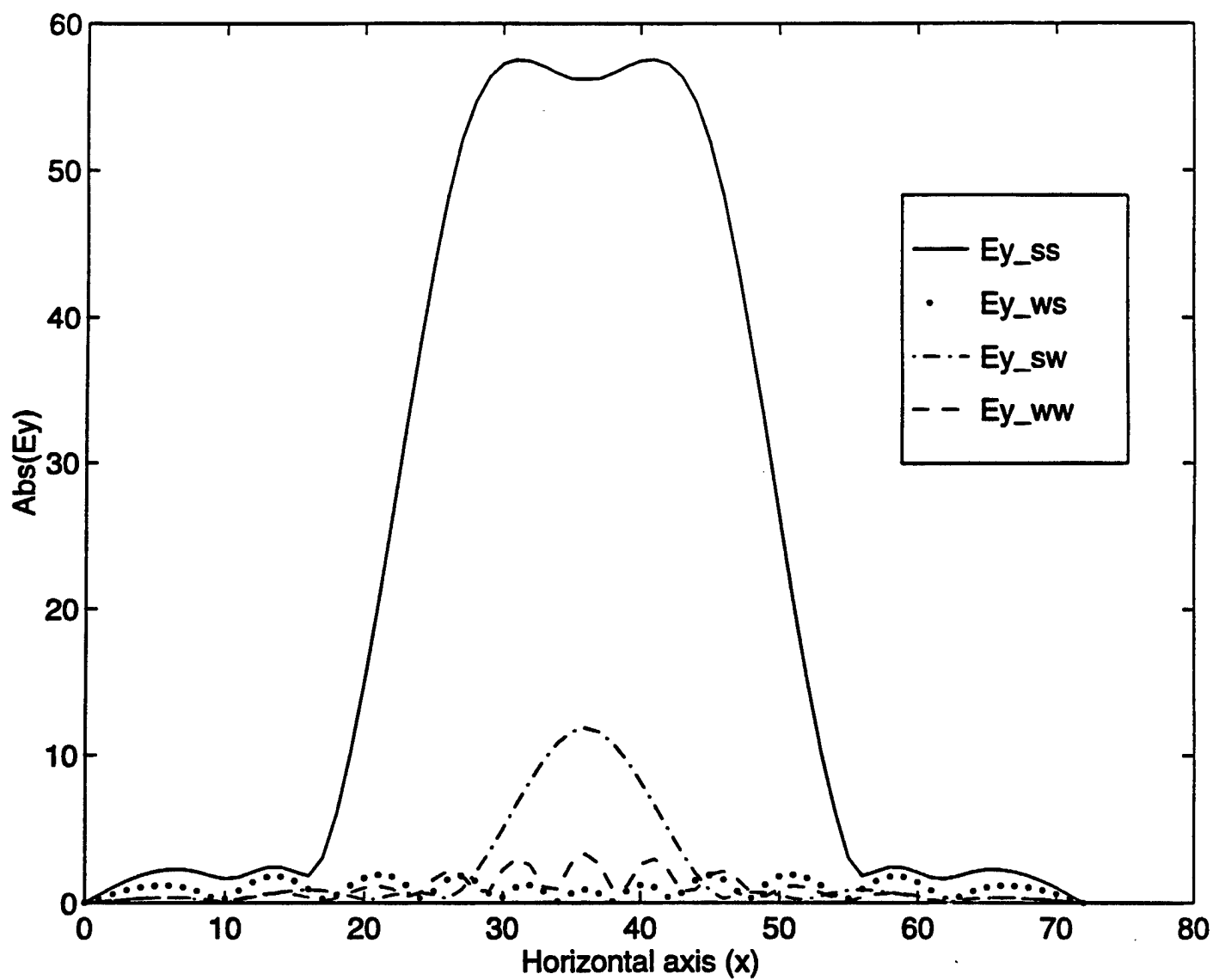
Figure 3: TEM E_y Pattern Components (8x8 Grid).
