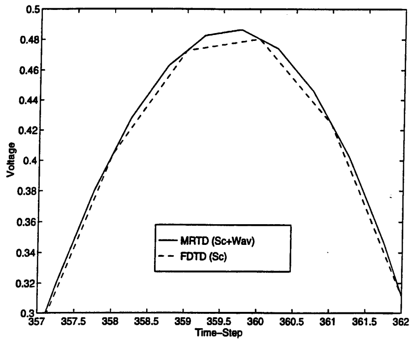
Figure 7.4: Comparison MRTD-FDTD.
