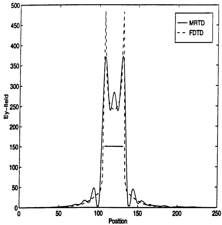
Figure 4.14: Open Single Stripline - E_y TEM Distribution.
