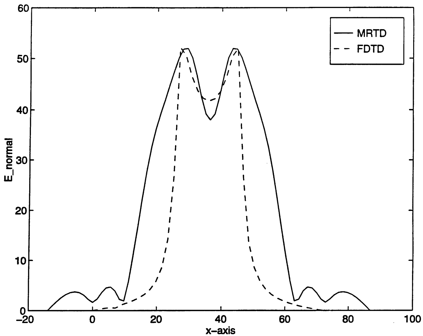
Figure 4: TEM E_y Pattern Comparison (8x8 Grid).
