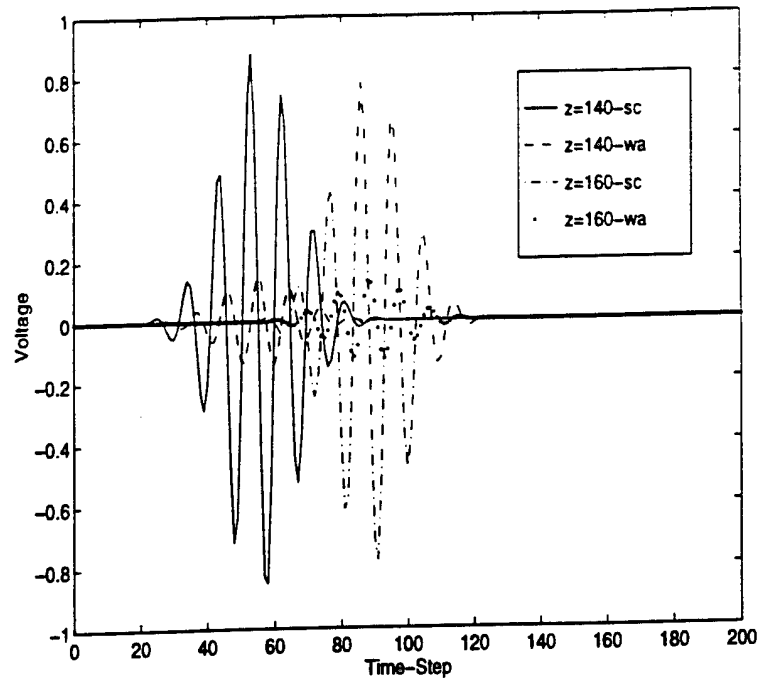
Figure 7.7: Voltage Coefficients.
