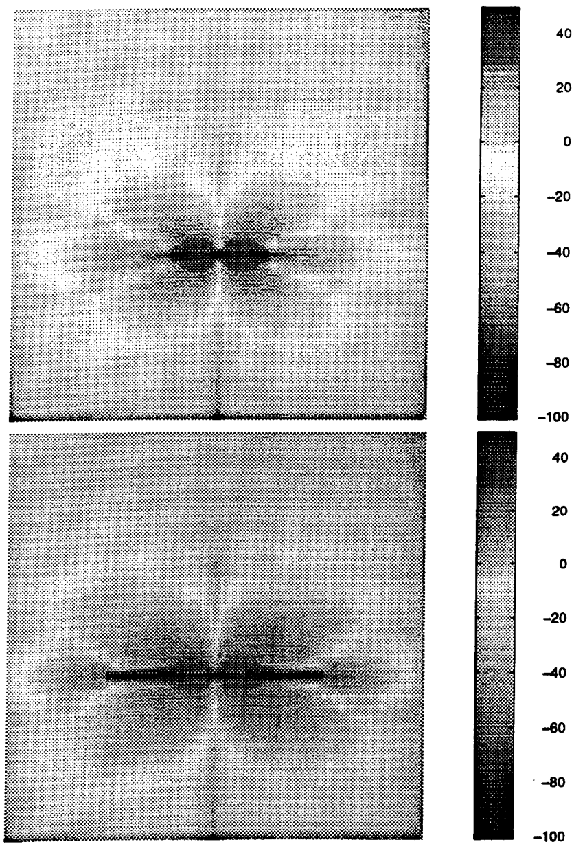
Figure 2.11: Normal H-Distribution (Log) for B=25 \mu\text{m} (up), 100 \mu\text{m} (bottom).
