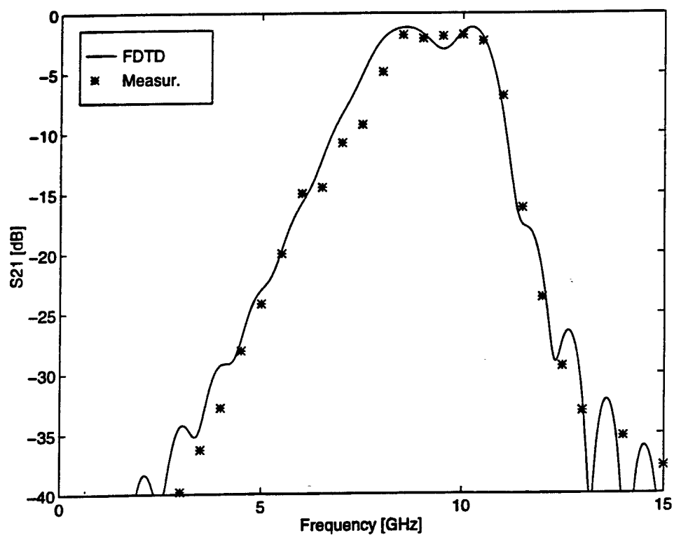
Figure 2.9: Coupled Line Filter S_{21} .
