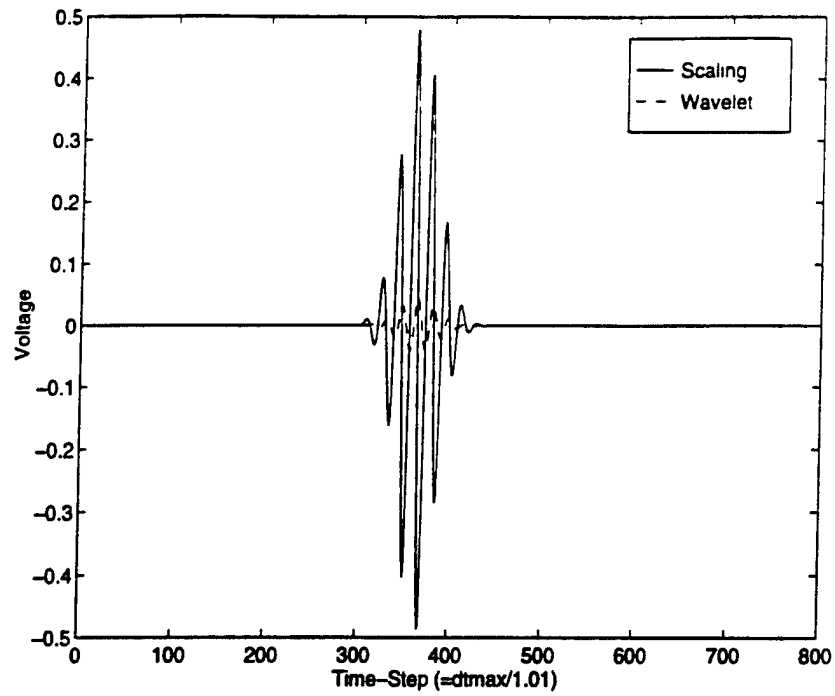
Figure 7.3: Voltage Coefficients.
