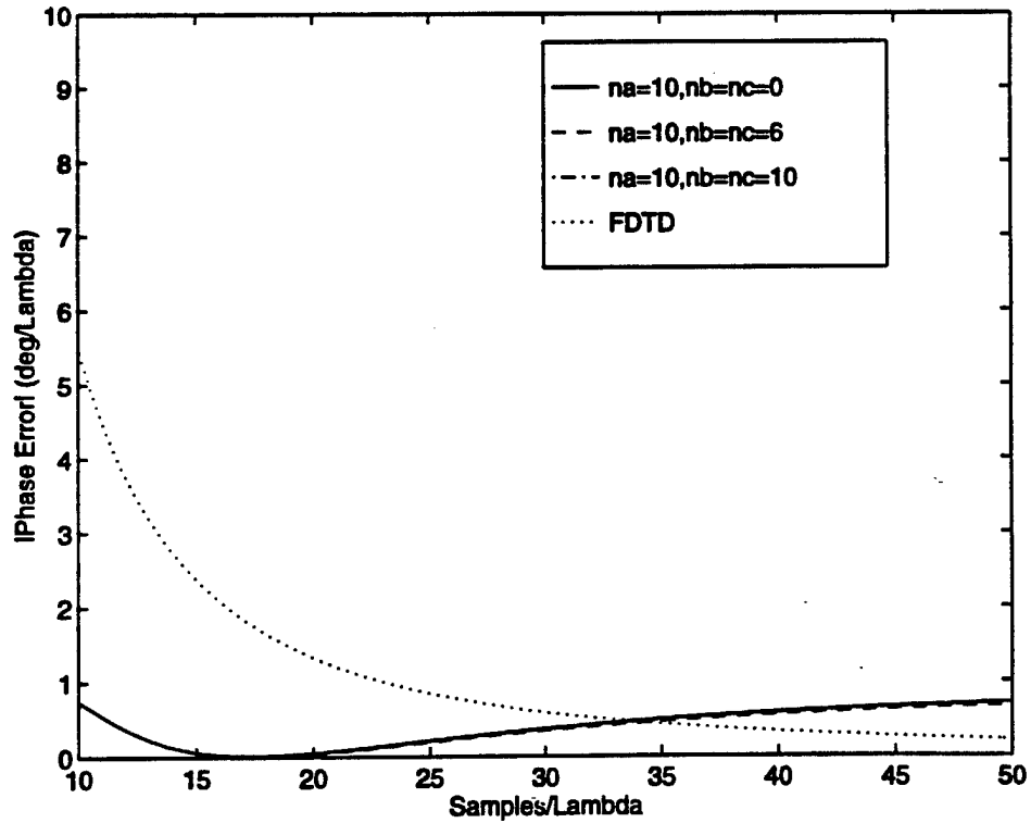
Figure 10: Wavelets Effect on the Dispersion Characteristics of MRTD for n_a=10 (Coarse Grid).
