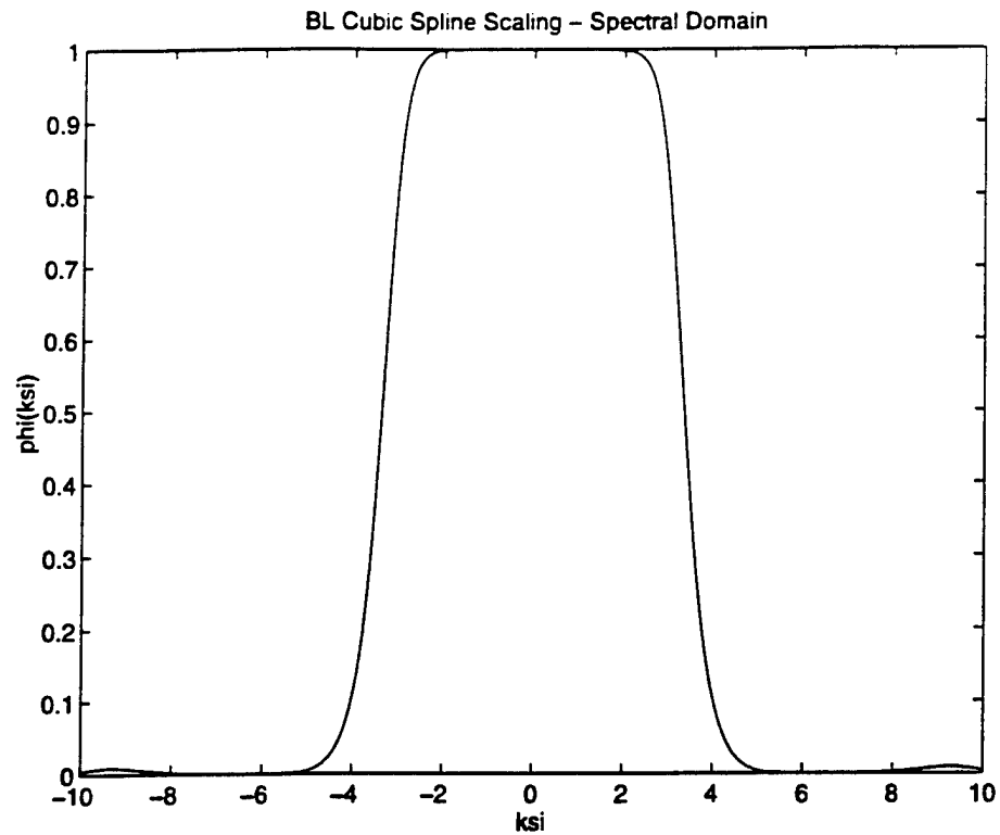
Figure 3.3: BL Cubic Spline Scaling - Spectral Domain.
