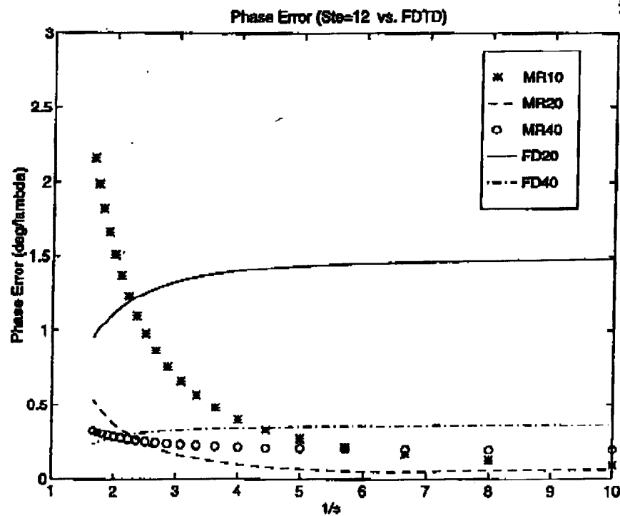
Figure 5.4: Dispersion Characteristics of S-MRTD for n_a=12 .
