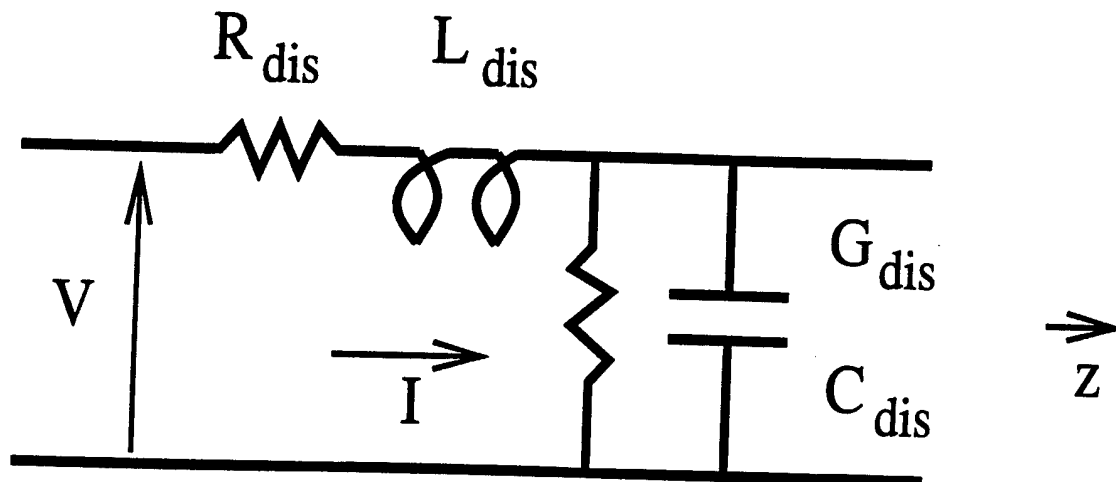
Figure 7.6: Lossy Transmission Line.
