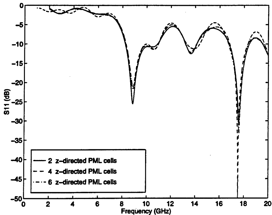
Figure 3: S_{11} comparison plots for a patch antenna
