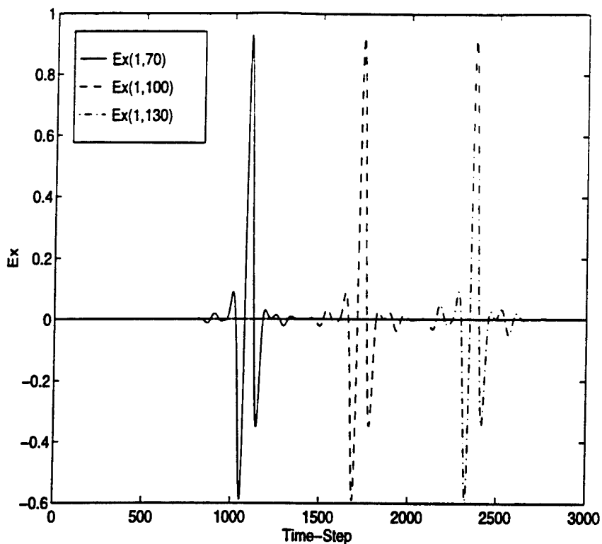
Figure 6.2: Normal E-field (Time-Domain).
