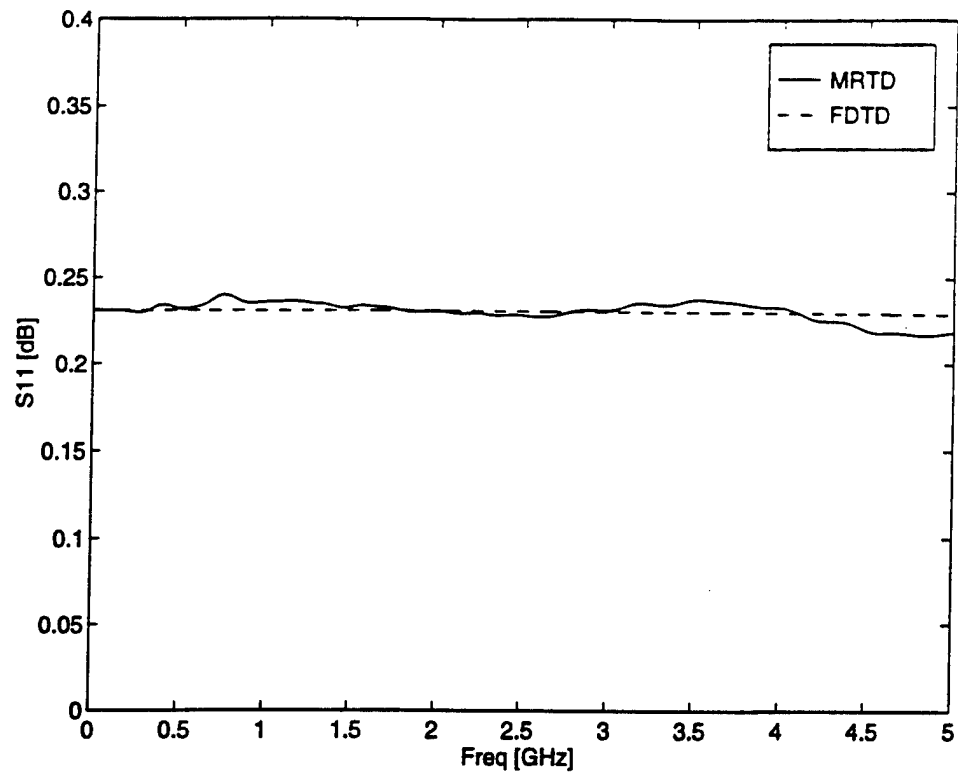
Figure 6.6: S-Parameters of the Waveguide.
