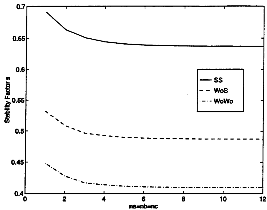
Figure 1: Stability Parameter s for MRTD.
