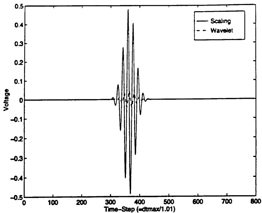
Figure 3: Voltage Coefficients.
