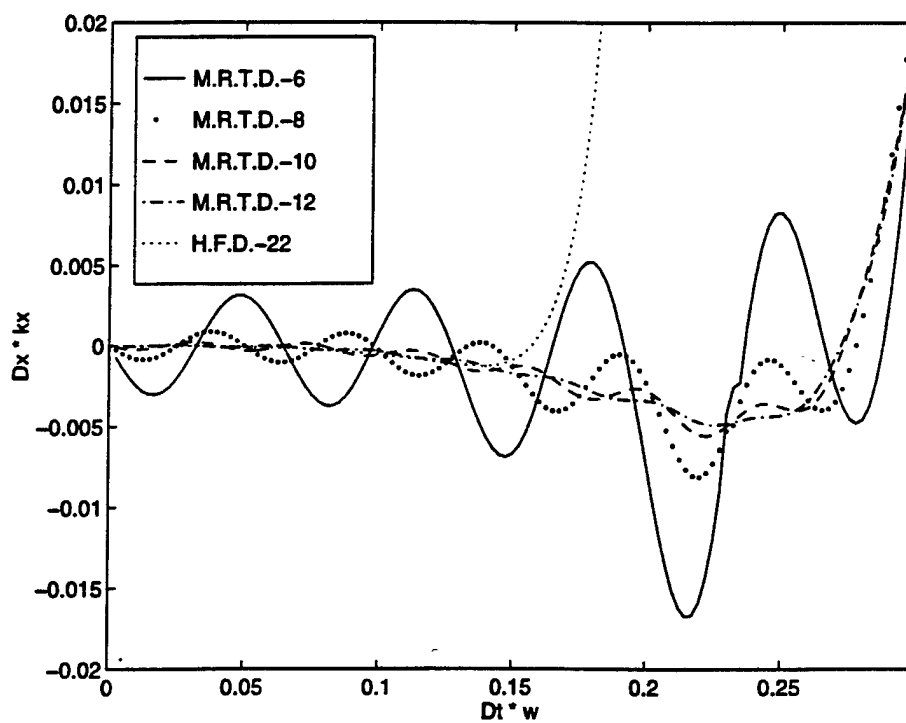
Figure 5.23: Details of Fig.(5.22).
