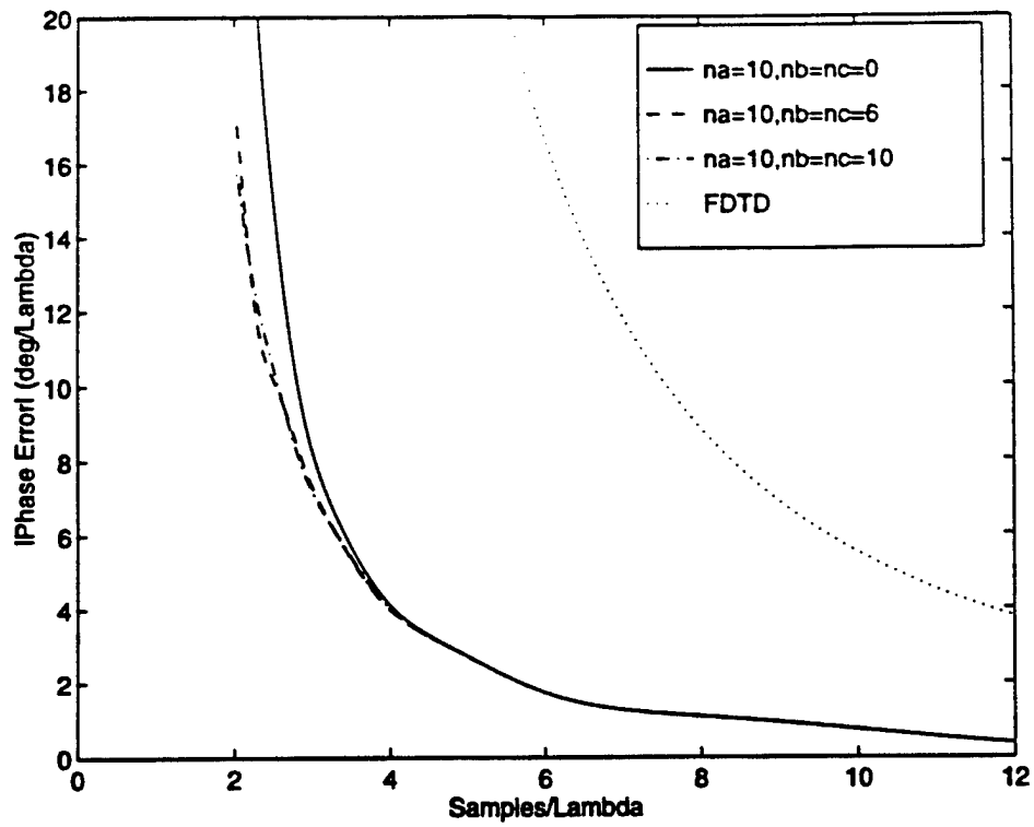
Figure 10: Wavelets Effect on the Dispersion Characteristics of MRTD for n_a=10 (Coarse Grid).
