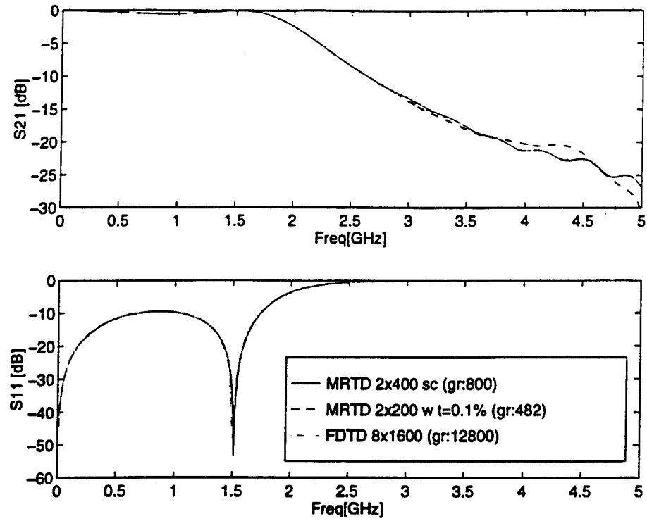
Figure 6.10: S-Parameters of the Filter.
