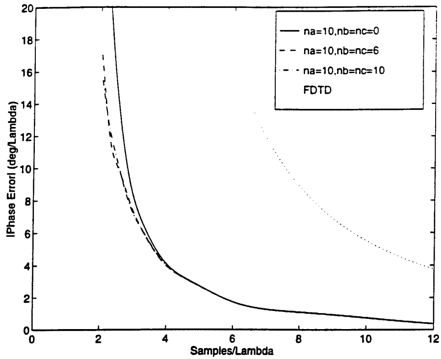
Figure 5.10: Wavelets Effect on the Dispersion Characteristics of MRTD for n_a=10 (Coarse Grid).
