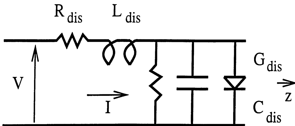
Figure 7.9: Rectifier Geometry.
