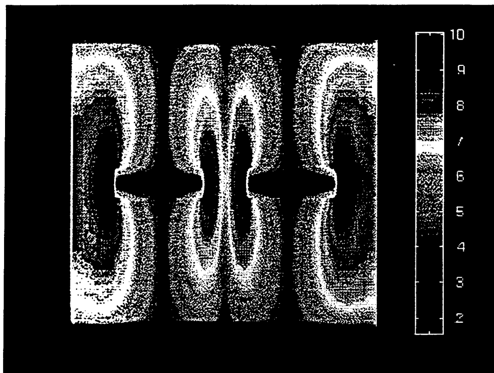
Figure 5: Tangential E-field Distribution (Shielded - Even Mode).
