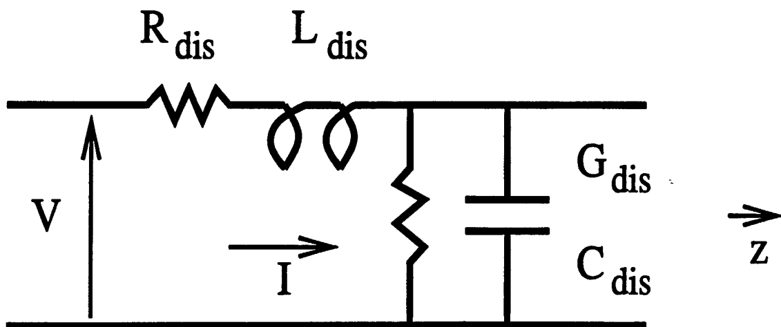
Figure 6: Lossy Transmission Line.
