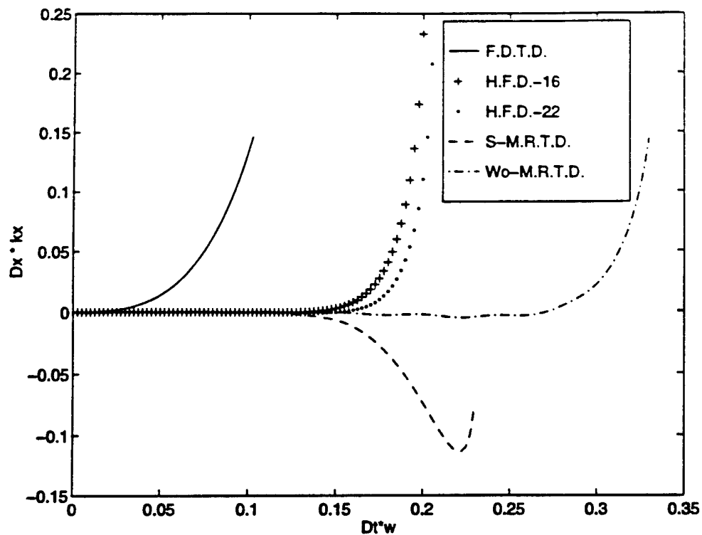
Figure 20: Comparison of the Dispersion Performance of S-MRTD and Wo-MRTD with Different Higher Order Yee's Schemes.
