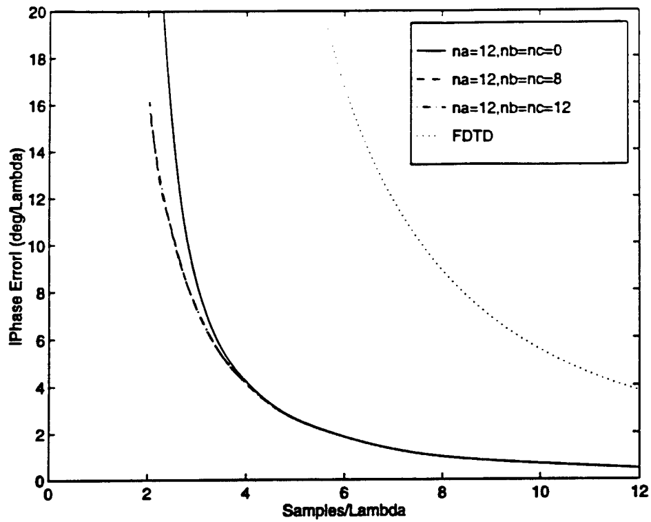
Figure 12: Wavelets Effect on the Dispersion Characteristics of MRTD for n_a=12 (Coarse Grid).
