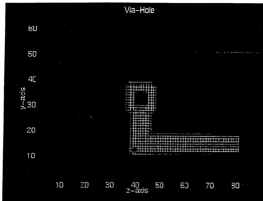
Figure 2.7: E-Distribution across Bottom Viahole.
