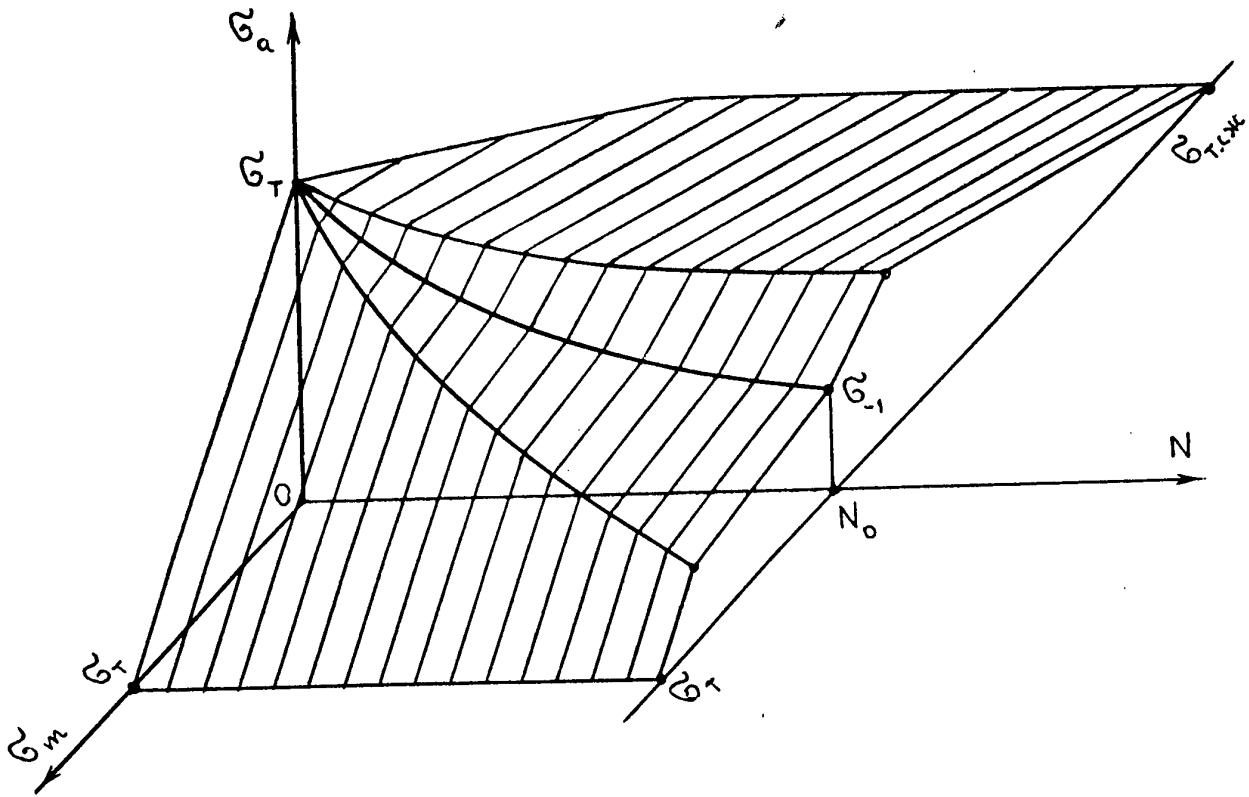
Fig.1 Fatigue surface.
