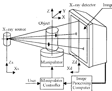
Figure 1. A single-head cone-beam X-ray system.
