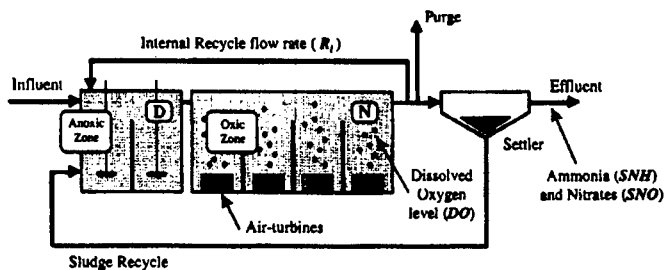
Fig. 1. Wastewater Treatment Plant
