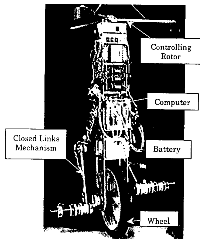
Fig. 1. Photo of extension-cableless unicycle robot.
