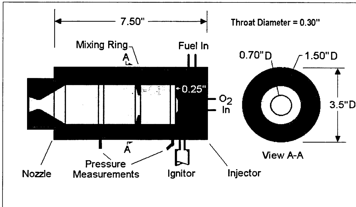
Figure 3.3 - Rocket Motor Overall Geometry
