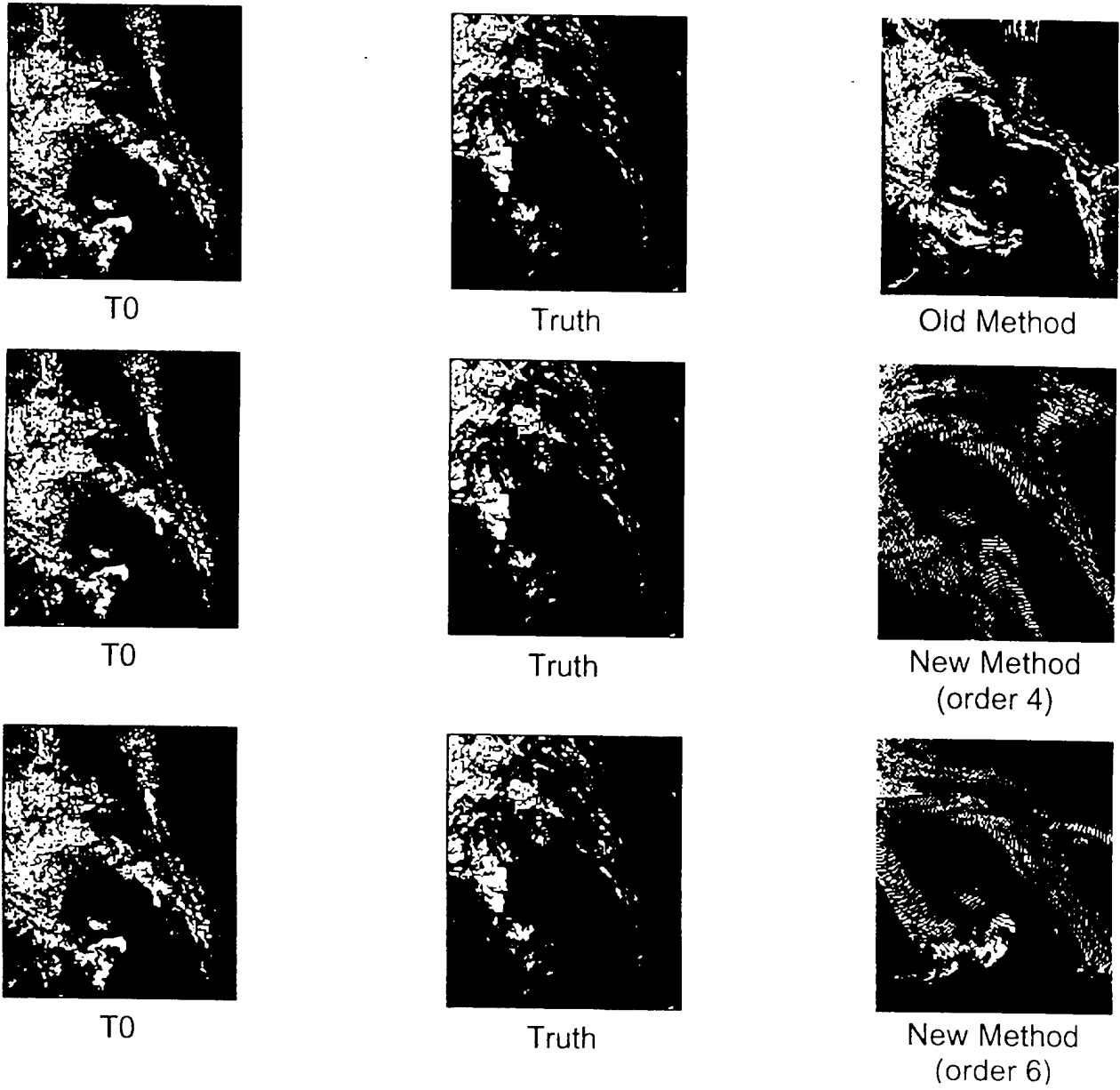
Figure 3-3. Cloud advection results.
