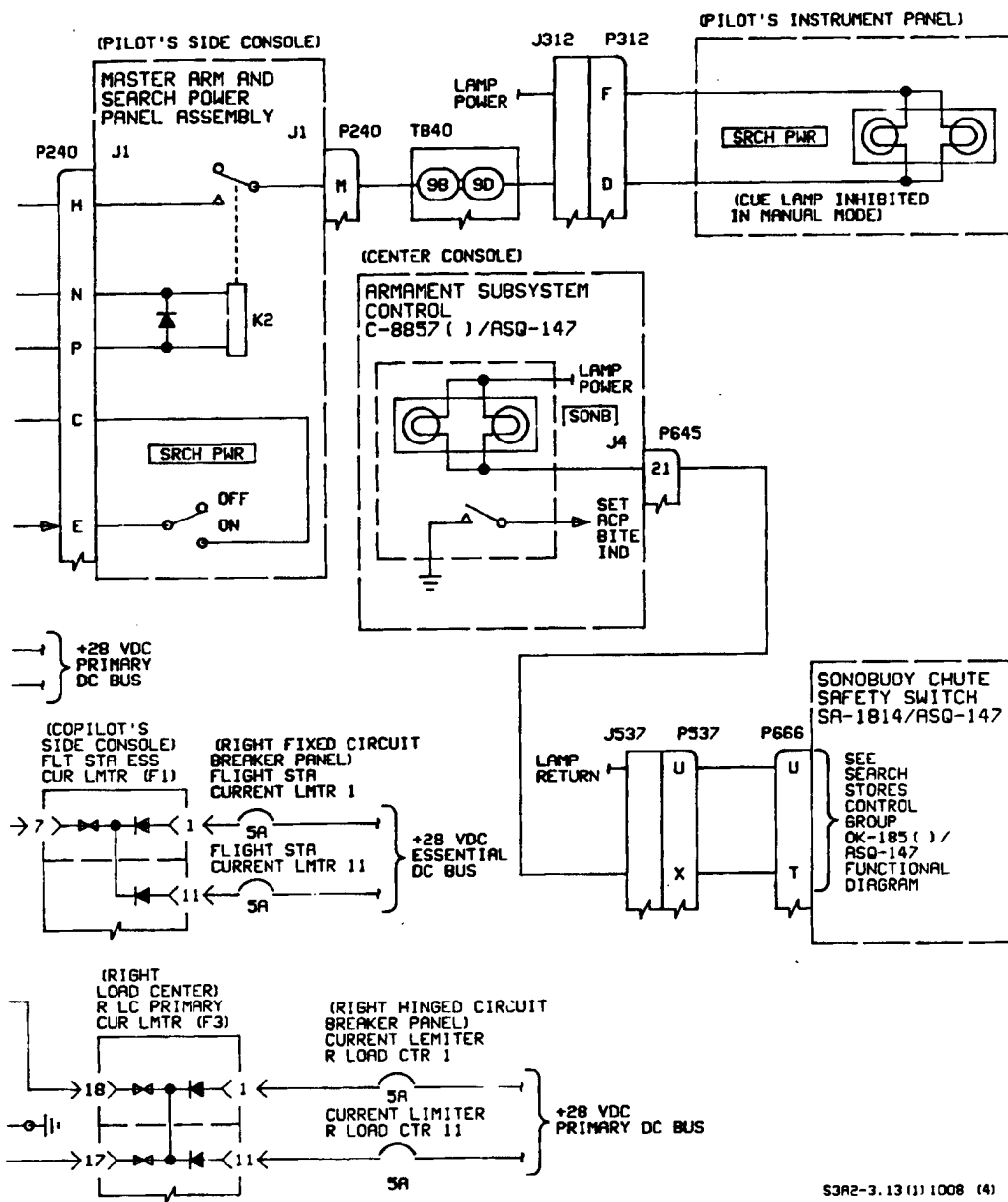
Figure 12. Search Stores Control Group OK-185( )/ASQ-147 Power Distribution Diagram (Sheet 4)
