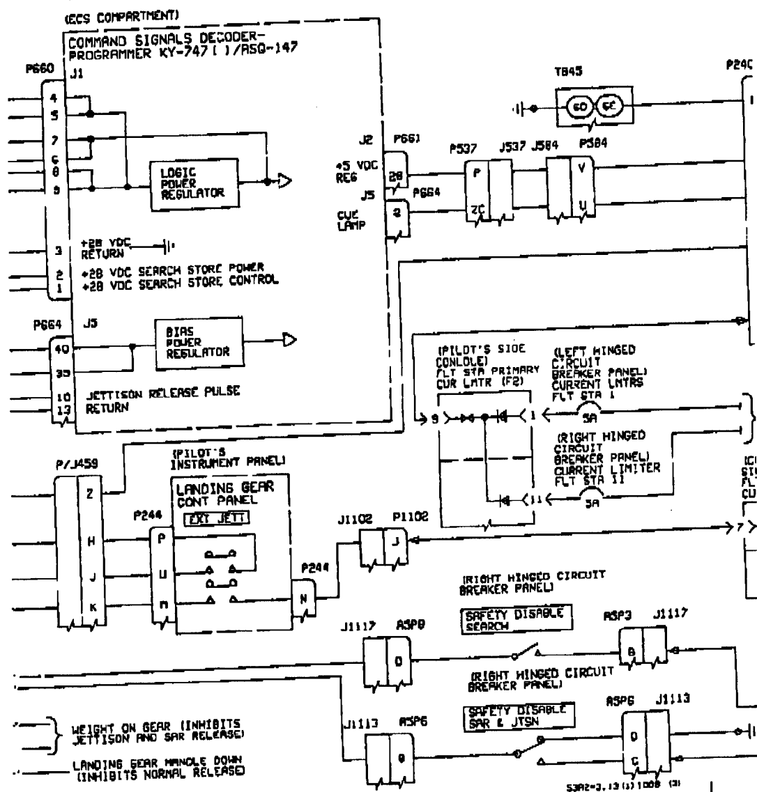
Figure 12. Search Stores Control Group OK-185( )/ASQ-147 Power Distribution Diagram (Sheet 3)
