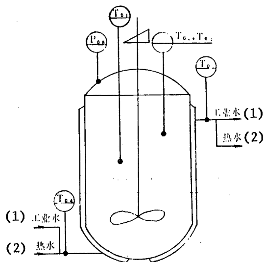
Figure 1. Checking Points of Polymerization Reactor
