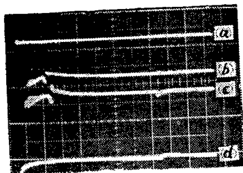
Figure 4. Nonresonant Multiple Photon Photo-Ionization Signals (a) 0.53\text{ }\mu\text{m} ; (b) 1.06\text{ }\mu\text{m} ; (c) 1.06\text{ }\mu\text{m} , 0.53\text{ }\mu\text{m} ; (d) delay monitor ( 1.06\text{ }\mu\text{m} and 0.53\text{ }\mu\text{m} represent the incident laser wavelength). The scale of (a), (b), and (c) is 10 mV/div, (d) is 20 mV/div
