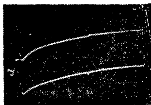
Figure 5. Sign Change of Photo-Ionization Signal Pulse When Action Zone Approaches Two Collector Plates (With 1.2 V DC collector potential)
