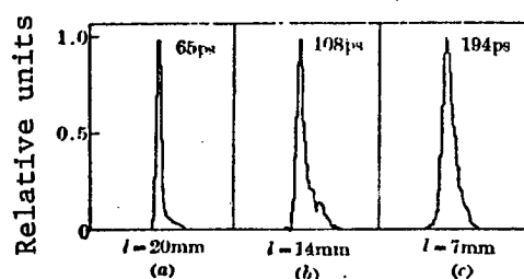
Figure 3. Effect of Traveling Wave Amplification Distance on Pulse Width
