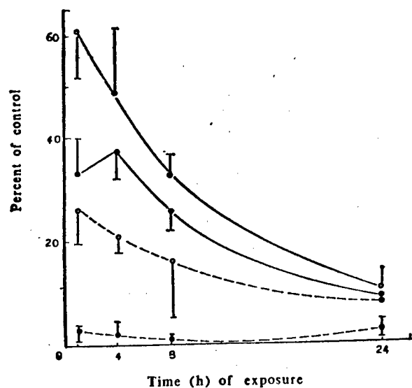
Figure 1. Survival of KB Cells After Continuous Treatment With HCPT Determined by Colony Formation Method
