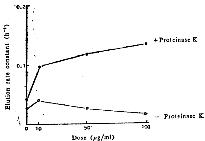
Figure 3. Relationship Between the Elution Rate and HCPT Dose
