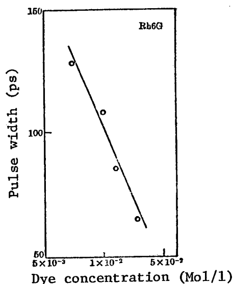
Figure 4. Influence of Dye Concentration on Pulse Width
