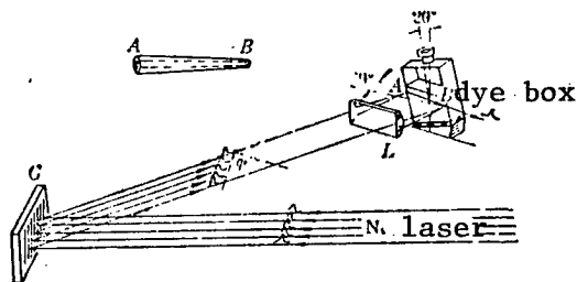
Figure 1. Experimental Apparatus
