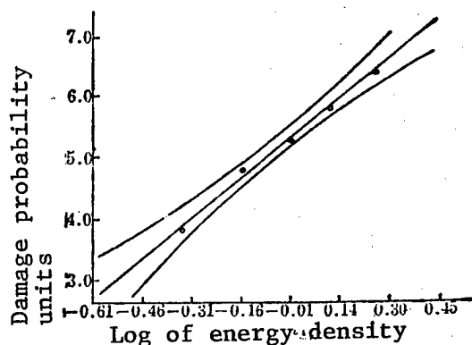
Figure 2. Relationship Between Probability Units of Damage to Rabbit Corneas Irradiated by XeCl Excimer Laser and the Log of the Dose
