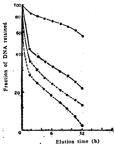
Figure 2. Elution Kinetics of DNA From KB Cells Prelabeled With [ ^{14}\text{C} ] Thymidine and Treated With Proteinase K Incubated With Various Concentrations of HCPT for 1 Hour.
