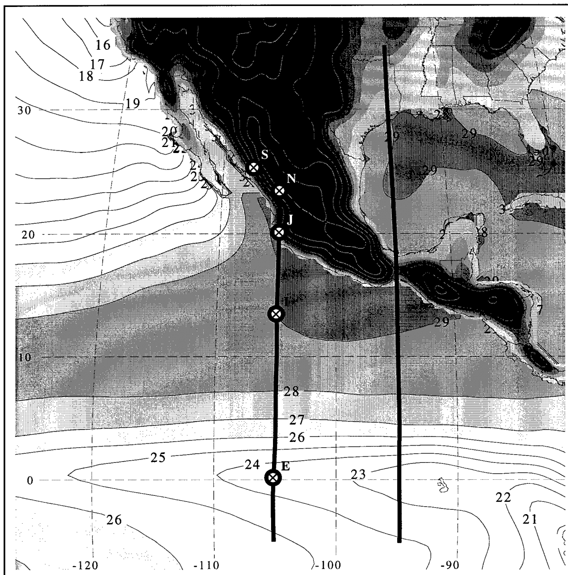
Figure 3.6. MM5 model terrain, locations of vertical cross sections (solid lines), locations of parcel trajectory ending locations (crosses), and mean SST in °C for JJA 1990-1997. Terrain contour intervals are 1000 m. SST contour intervals are 1 °C. SST is shaded above 26 °C.
