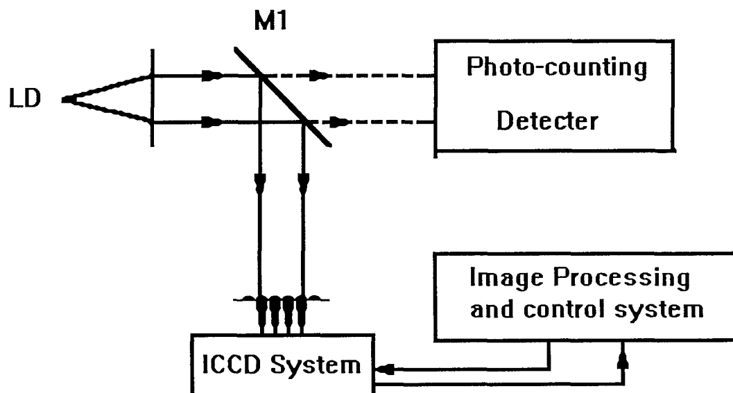
Fig.1. Schematic of the configuration in the test.
