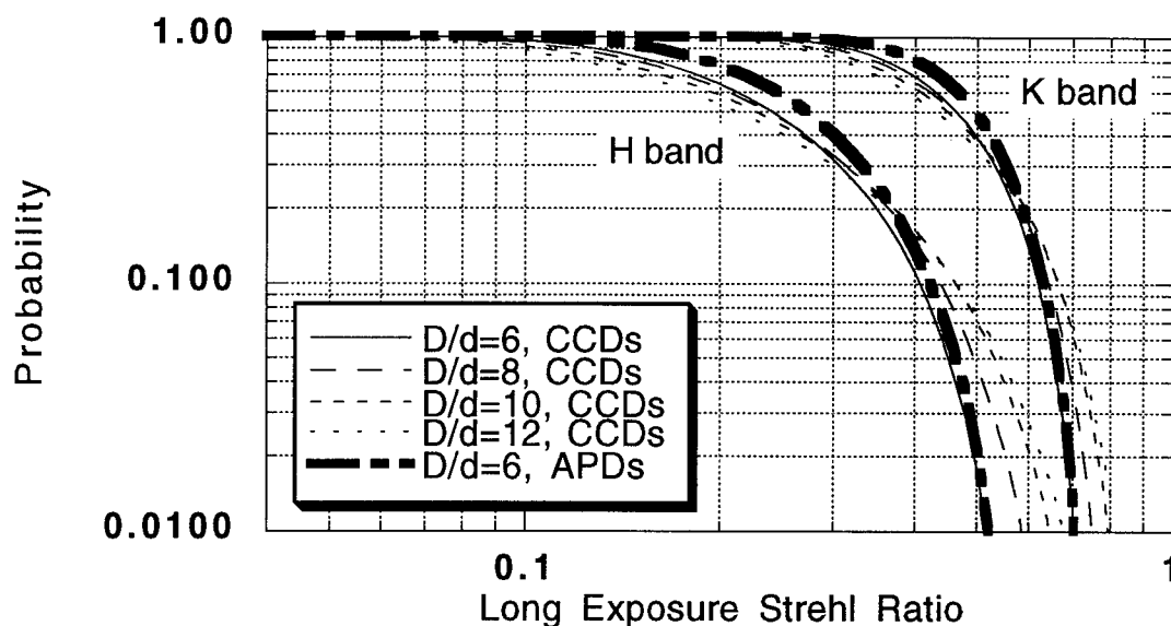
Figure 1: Sky coverage probabilities vs detector technology and order of correction ( D/d )
