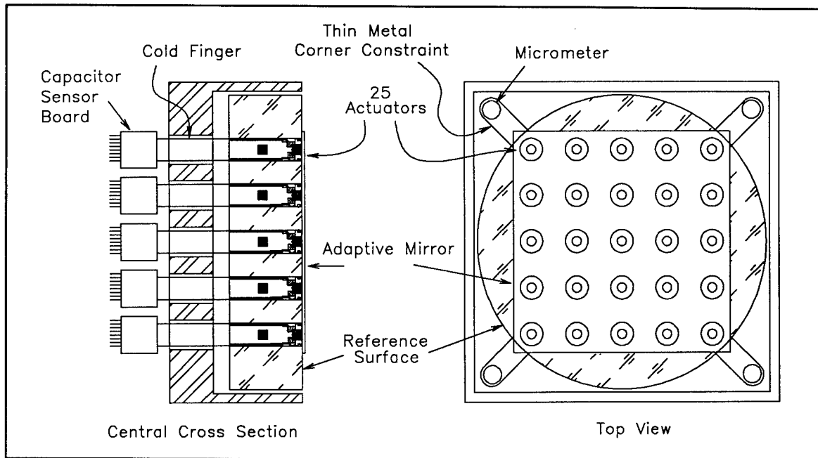
Figure 3. 25-element Prototype
