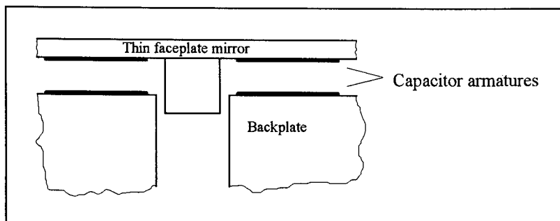
Fig. 1 - Sensing capacitator scheme
