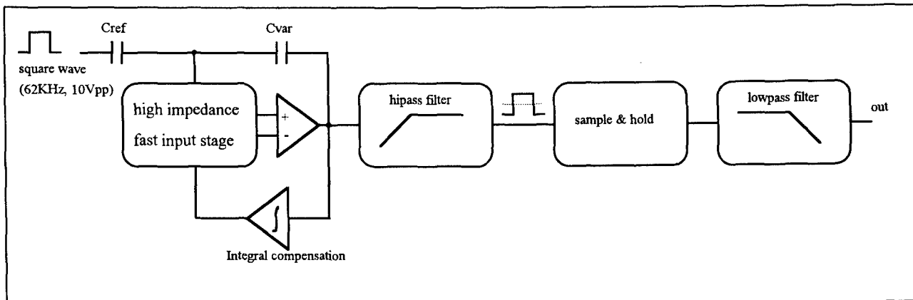
Fig. 3 - Conceptual scheme of the electronic circuit
