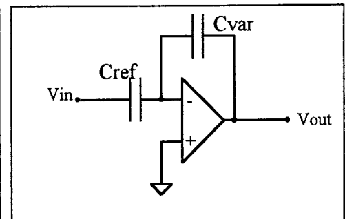
Fig. 2 - Working principle
