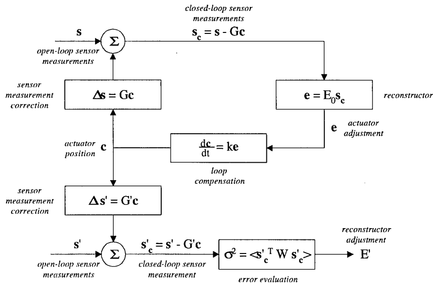
Figure 1. Adaptive optics system control loop diagram.
