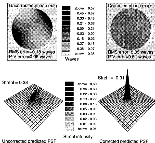
Fig. 2. Correction of static wavefront aberrations using the LC-SLM. The top two plots are uncorrected and corrected greyscale phase maps as measured by the interferometer. The bottom two plots show the expected PSFs obtained by Fourier transforming the phase maps.
