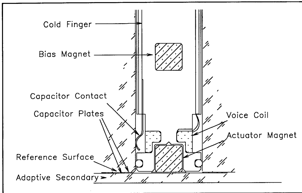
Figure 2. Actuator Assembly
