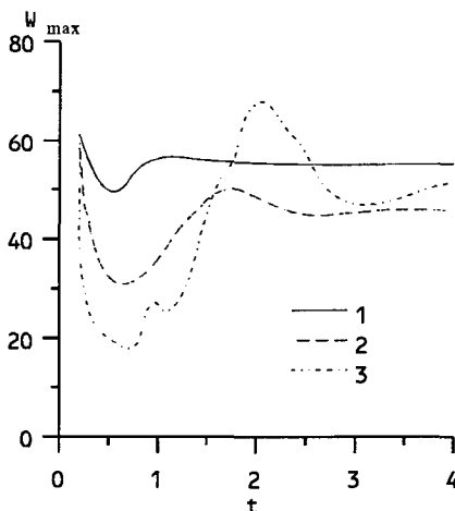
Fig. 3. Dynamics of peak intensity W_{\max}(t) in the AOS focus with the Hartmann sensor. 1— W_0 = 16 ; 2— W_0 = 32 ; 3— W_0 = 64 .
