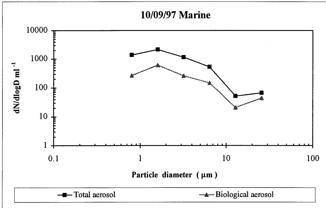
Figure 2 (e) Total and biological aerosol size distribution. \text{dN}/\text{dlogD} per ml vs. diameter ( \mu\text{m} )
