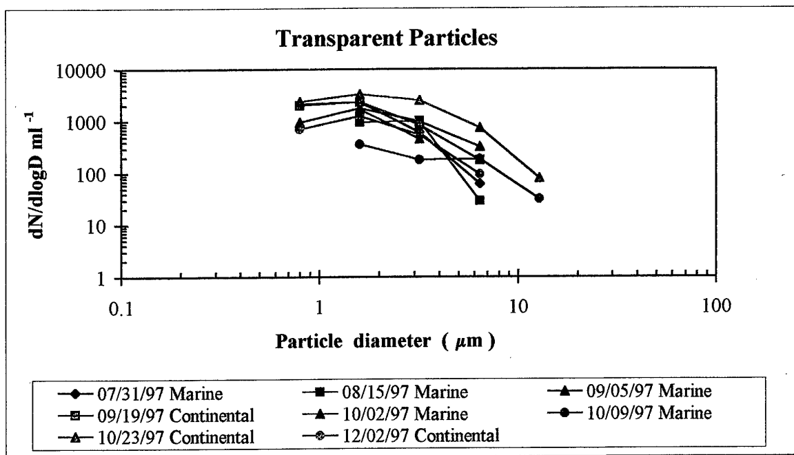
Figure 2 (d) Transparent particle size distribution. dN/dlogD per ml vs. diameter (μm)
