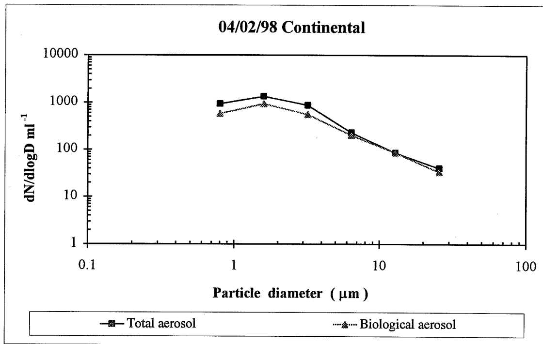
Figure 3 (b) Total and biological aerosol size distribution. \text{dN}/\text{dlogD} per ml vs. diameter ( \mu\text{m} )
