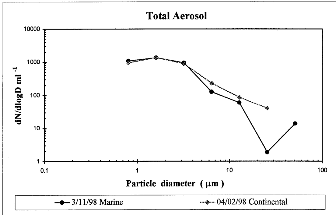
Figure 3 (c) Total aerosol size distribution. dN/d\log D per ml vs. diameter ( \mu m )
