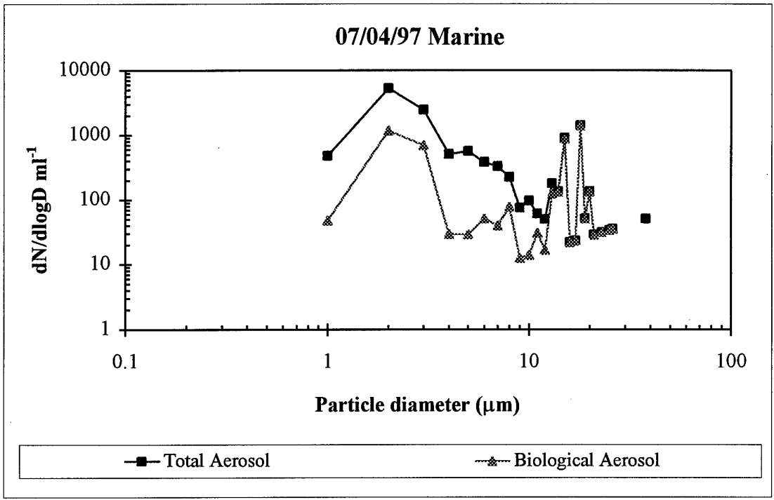
Figure 1 (a) Total and biological aerosol size distribution. dN/dlogD per ml vs. diameter (μm)
