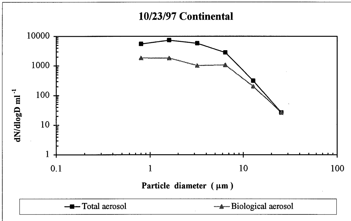
Figure 2 (f) Total and biological aerosol size distribution. \text{dN}/\text{dlogD} per ml vs. diameter ( \mu\text{m} )
