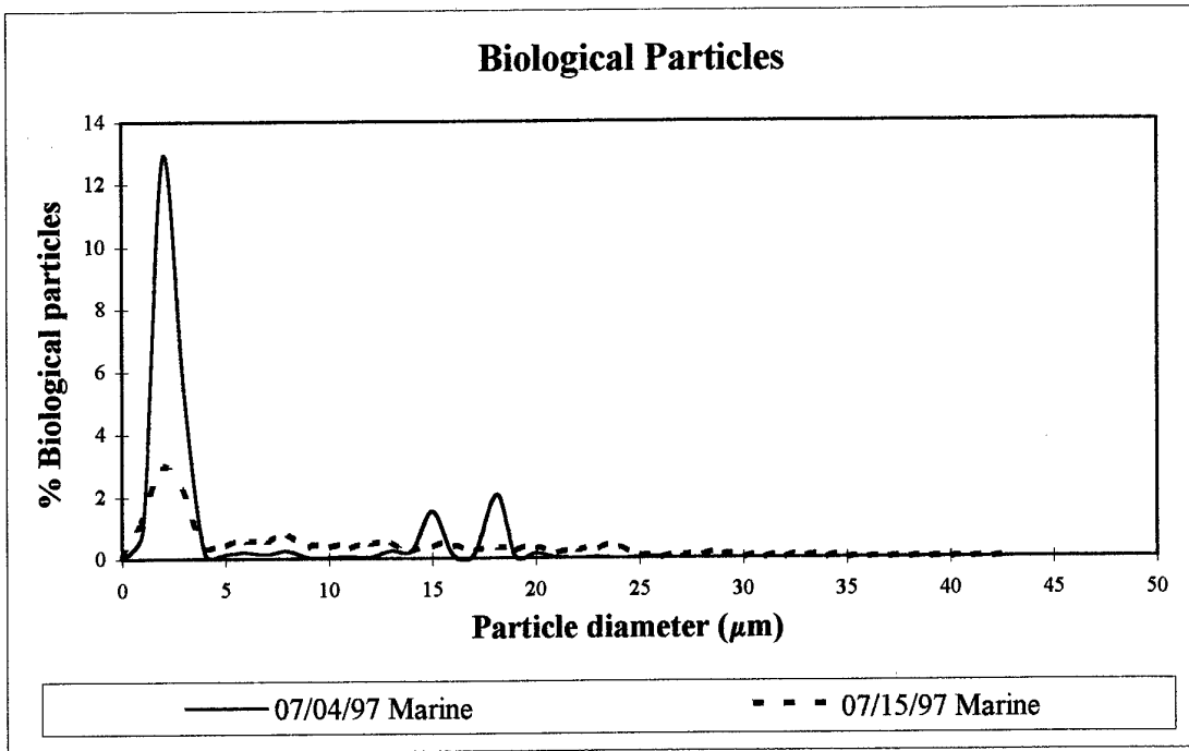
Figure 1 (e) Percentage (%) of biological particles to total aerosol particles vs. diameter ( \mu\text{m} )
