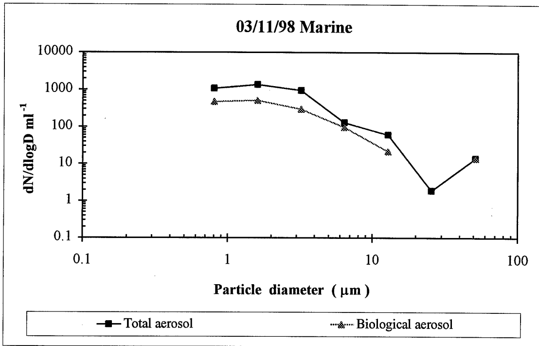
Figure 3 (a) Total and biological aerosol size distribution. \text{dN}/\text{dlogD} per ml vs. diameter ( \mu\text{m} )
