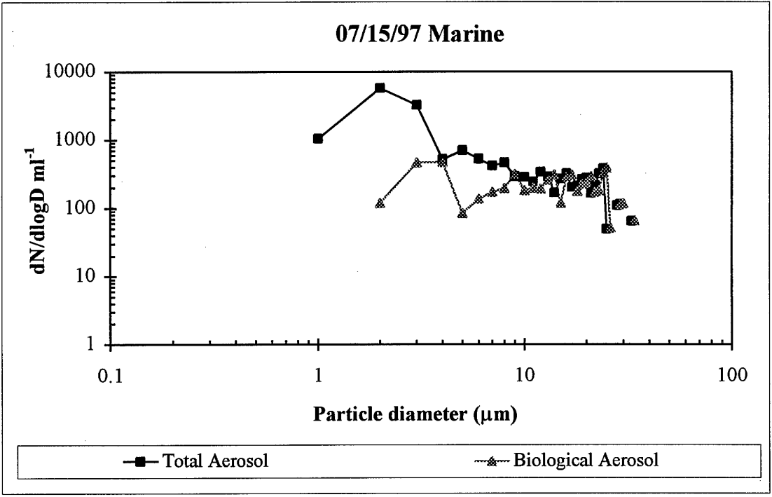
Figure 1 (b) Total and biological aerosol size distribution. dN/dlogD per ml vs. diameter (μm)
