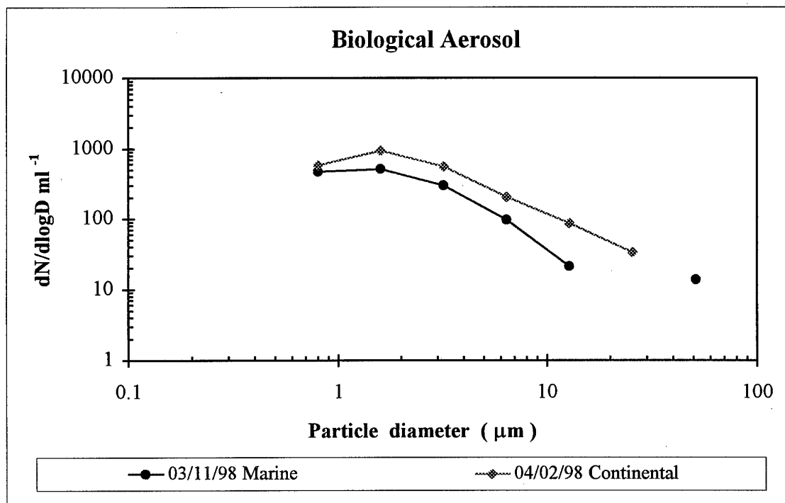
Figure 3 (d) Biological aerosol size distribution. dN/d\log D per ml vs. diameter ( \mu m )
