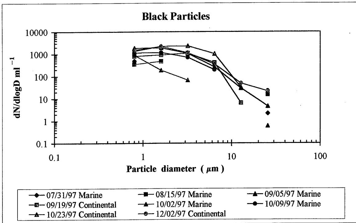
Figure 2 (c) Black particle size distribution. dN/dlogD per ml vs. diameter (μm)
