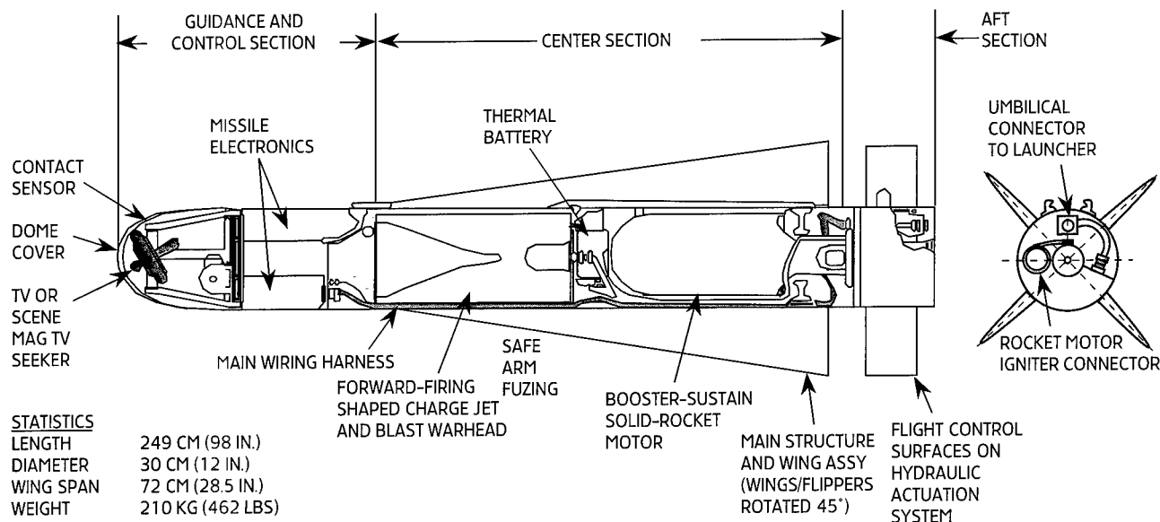
FIGURE 3. Electronic Component Arrangement
