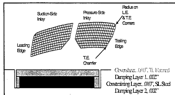
FIGURE 40. ACCS 1 Blisk
