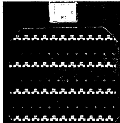
FIGURE 20. An Array of PdCr Thin-Film Strain Gage Batch Fabricated on a Ceramic Substrate
