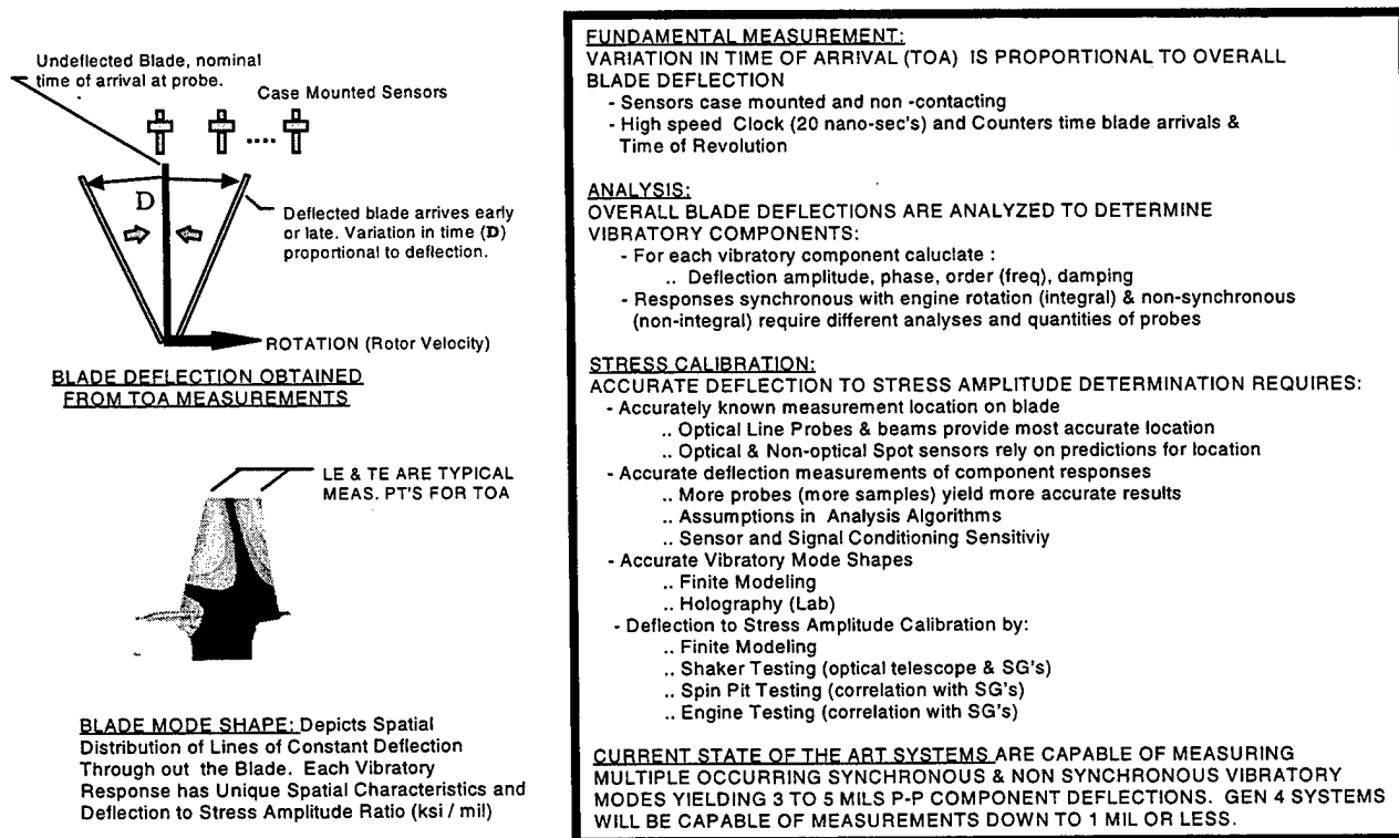
FIGURE 15. Rotating Blade Dynamic Stress Determination by NSMS
