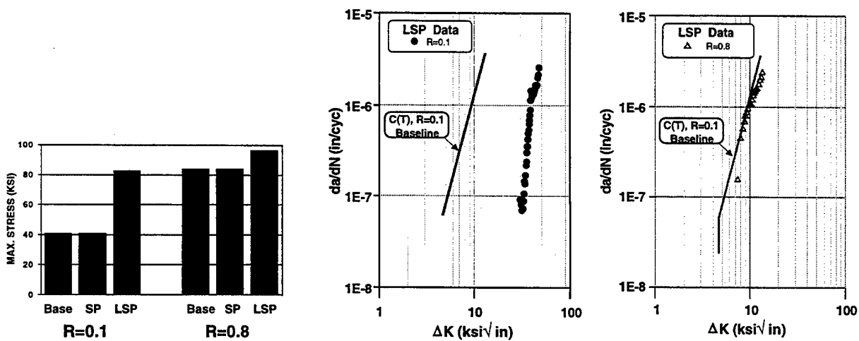
FIGURE 10. Notched Fatigue and Fatigue Crack Growth Behavior of LSP'd Ti-6Al-4V
