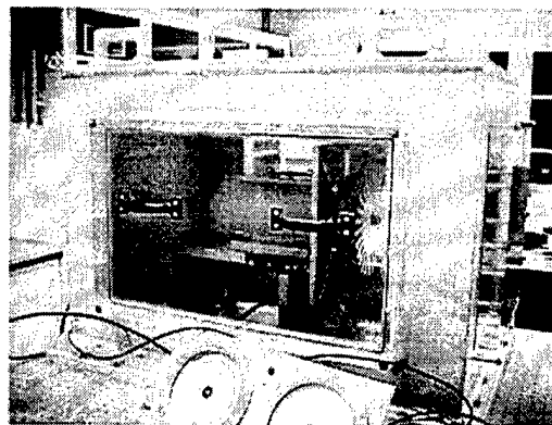
FIGURE 48. AFRL Vacuum Chamber
