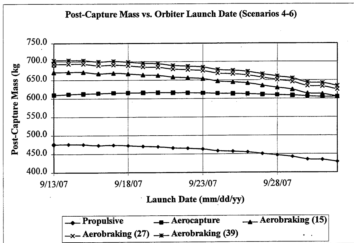
Figure 6.15: Scenarios 4,5,6 – Orbiter Post-Capture Mass
