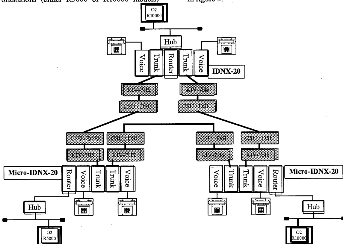
Figure 5. 3 node RTI test configuration with communications devices
