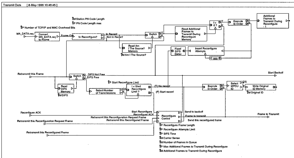
Figure 3-9 Transmit Data
