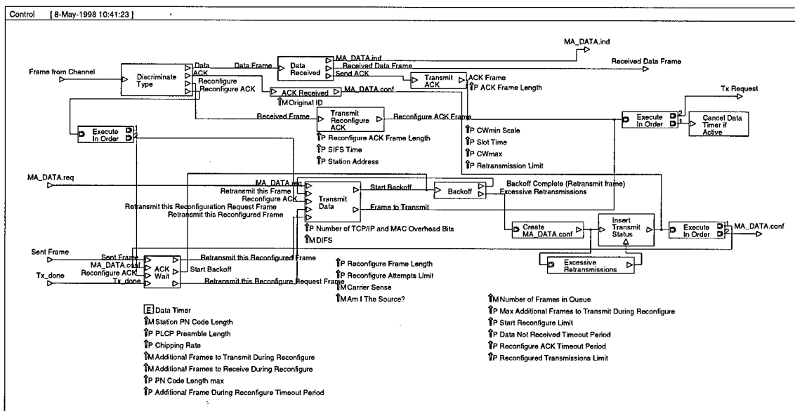
Figure 3-8 The Control Module
