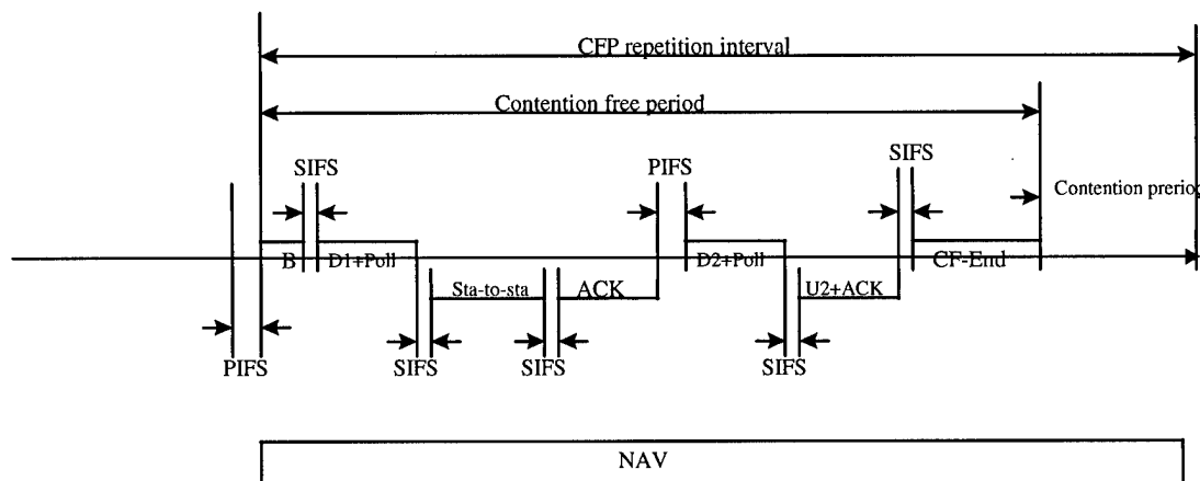
Figure 2-9 Station to Station Transmission
