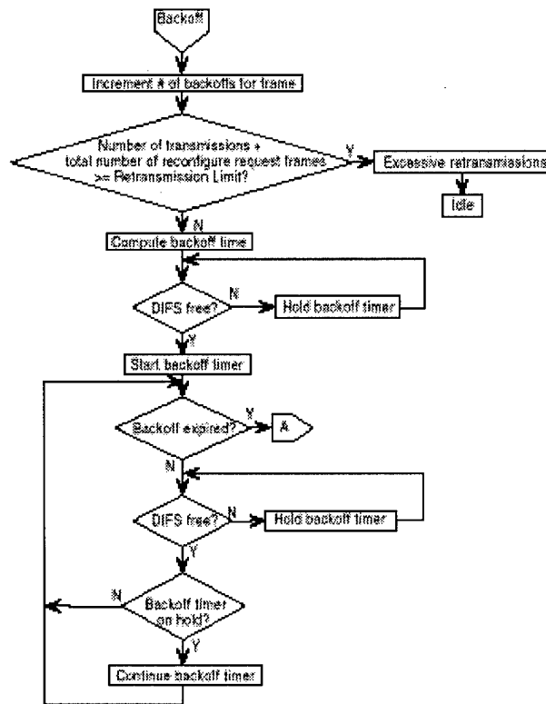
Figure 3-4 Backoff [Mul97]
