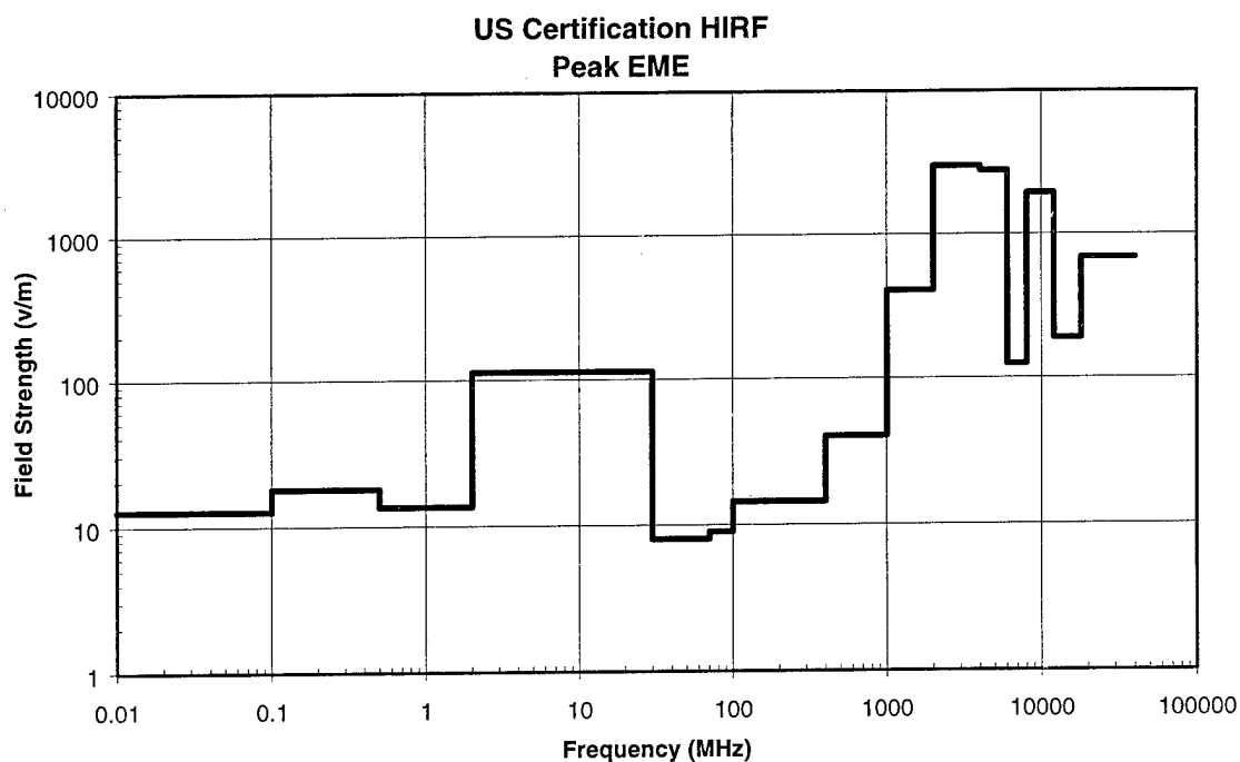
FIGURE 13 PEAK U.S. CERTIFICATION ENVIRONMENT
