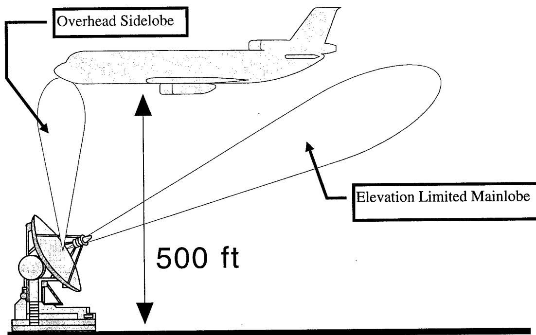
FIGURE 6 ILLUSTRATION OF OVERHEAD ILLUMINATION
