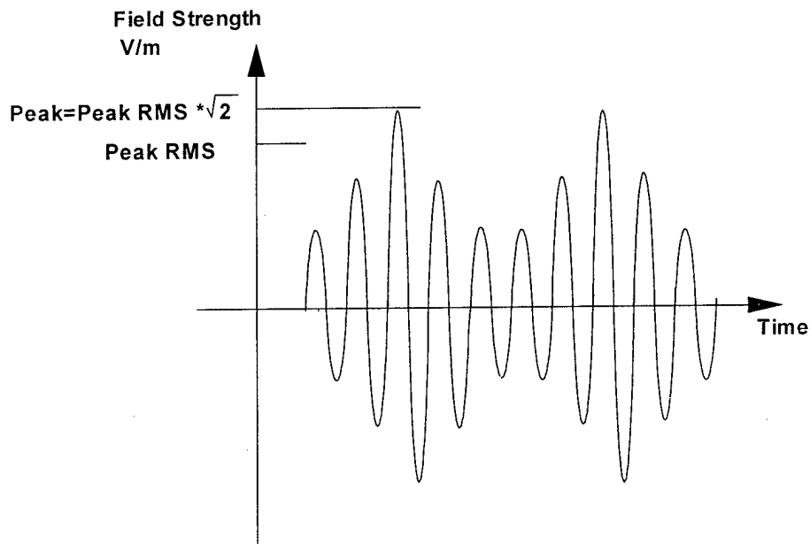
Figure B-1 AMPLITUDE MODULATED SIGNAL
