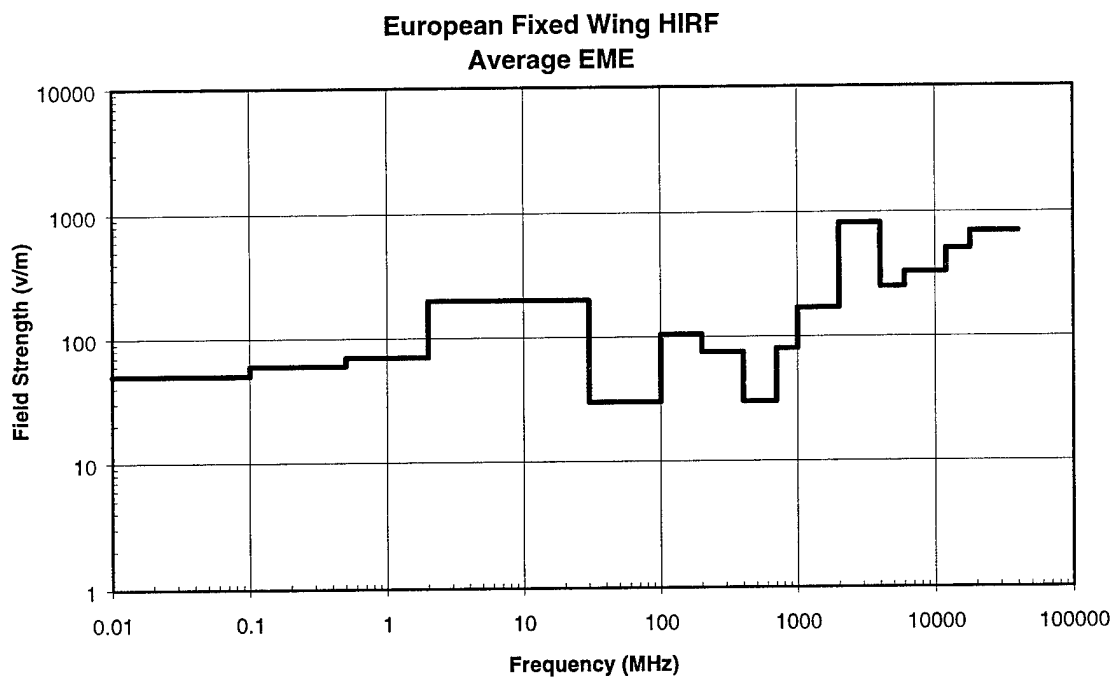
FIGURE 20 AVERAGE EUROPEAN FIXED WING SEVERE ENVIRONMENT
