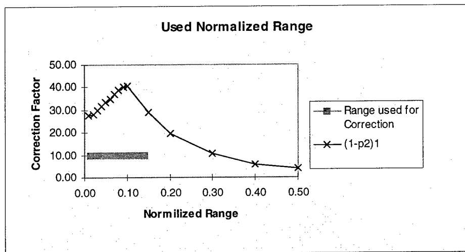
FIGURE 7 EXAMPLE OF NEAR-FIELD CORRECTION FACTOR
