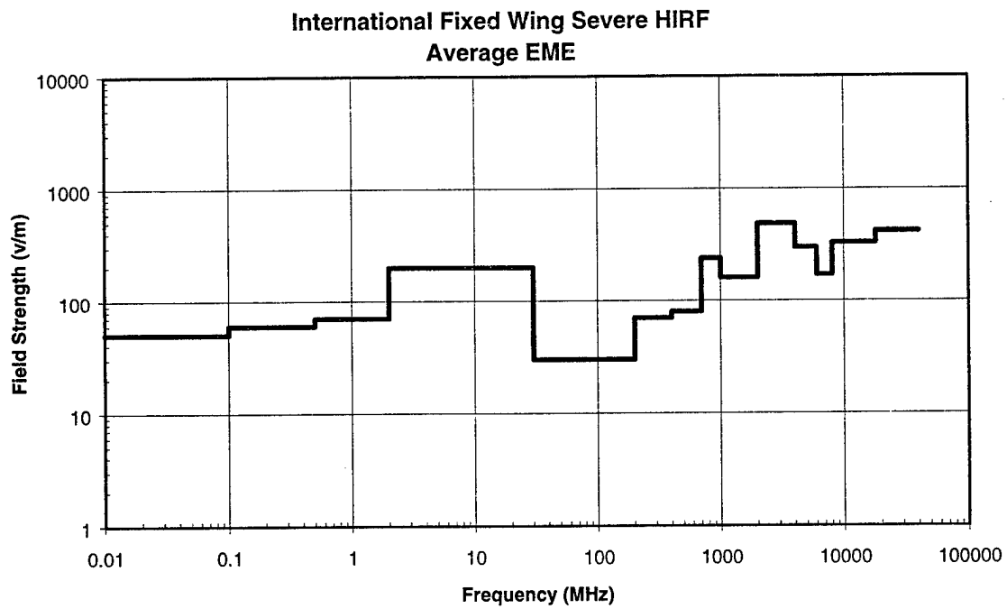
FIGURE 28 AVERAGE INTERNATIONAL FIXED WING SEVERE ENVIRONMENT
