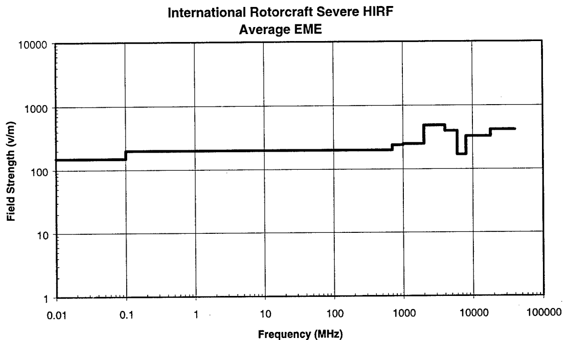
FIGURE 26 AVERAGE INTERNATIONAL ROTORCRAFT SEVERE ENVIRONMENT
