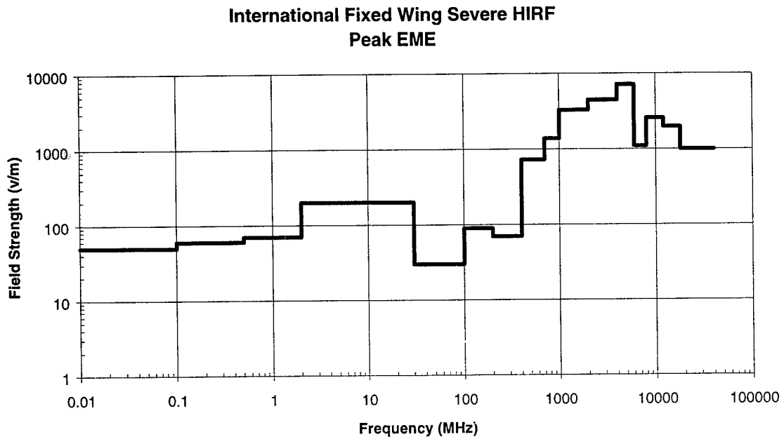
FIGURE 27 PEAK INTERNATIONAL FIXED WING SEVERE ENVIRONMENT
