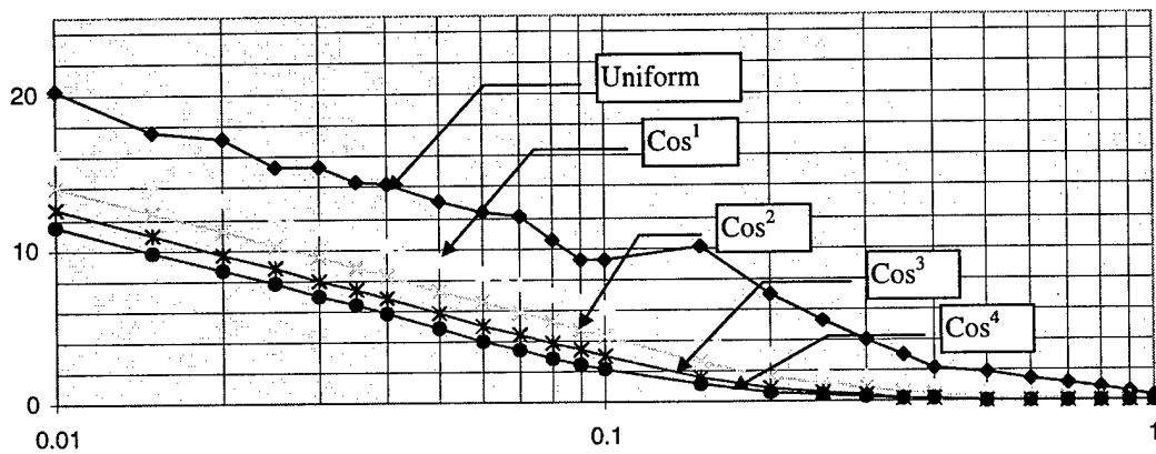
FIGURE 3 NEAR-FIELD CORRECTION FACTORS FOR RECTANGULAR APERTURE
