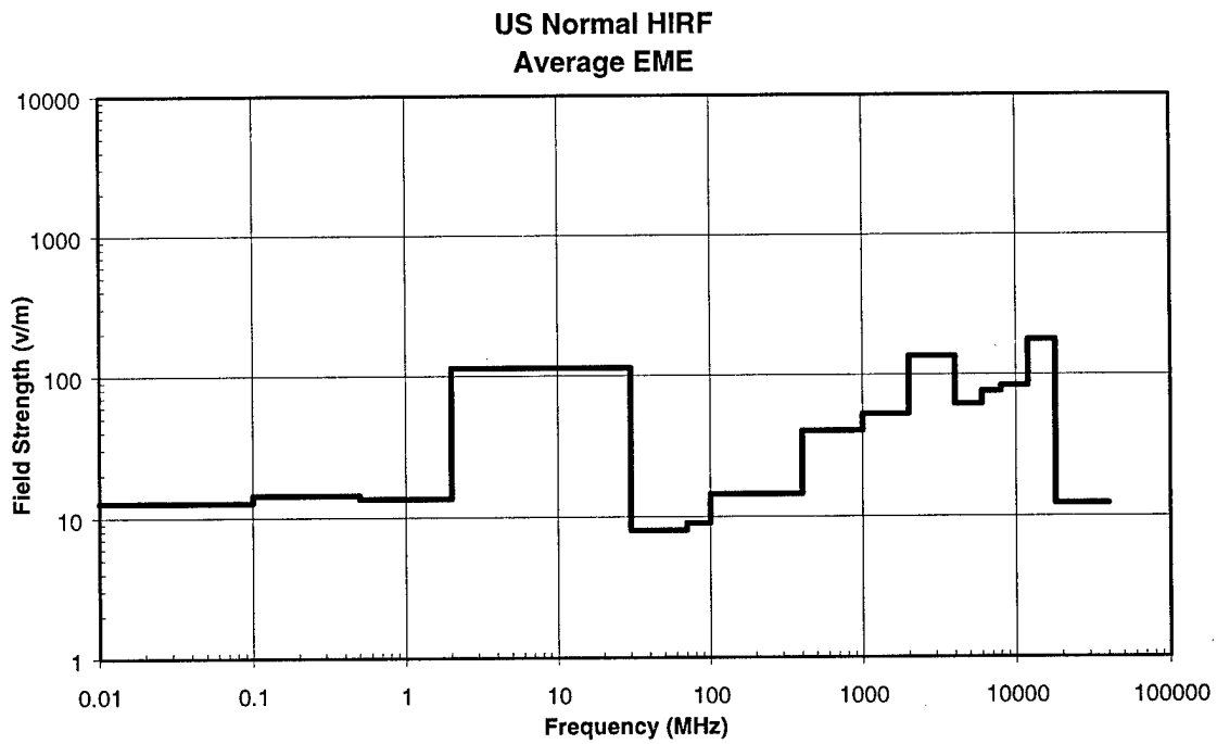
FIGURE 16 AVERAGE U.S. NORMAL ENVIRONMENT
