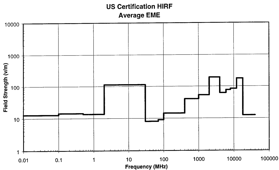
FIGURE 14 AVERAGE U.S. CERTIFICATION ENVIRONMENT
