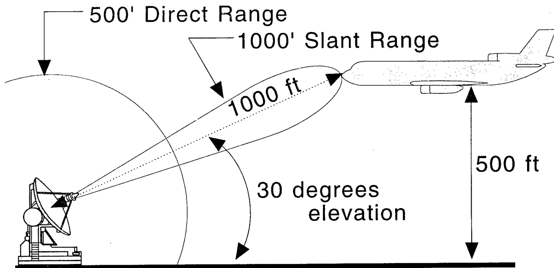
FIGURE 5 ILLUSTRATION OF SLANT ILLUMINATION
