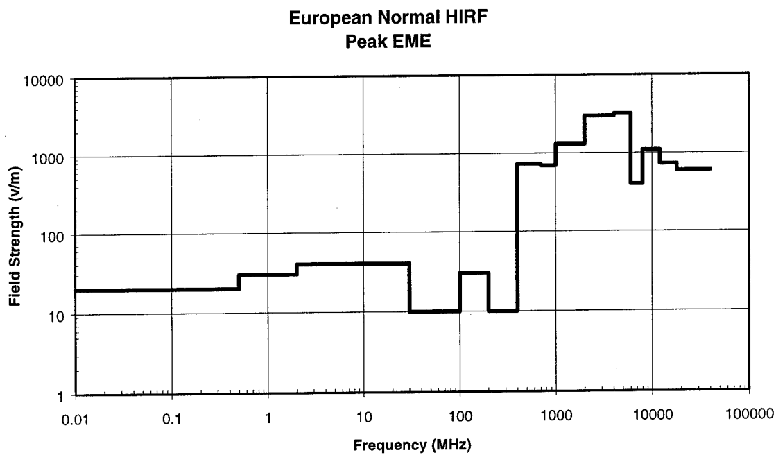
FIGURE 23 PEAK EUROPEAN NORMAL ENVIRONMENT
