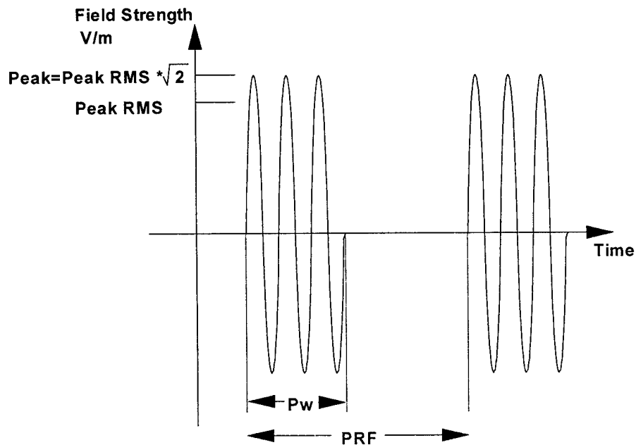
Figure B-2 PULSE MODULATED OR GATED SIGNAL
