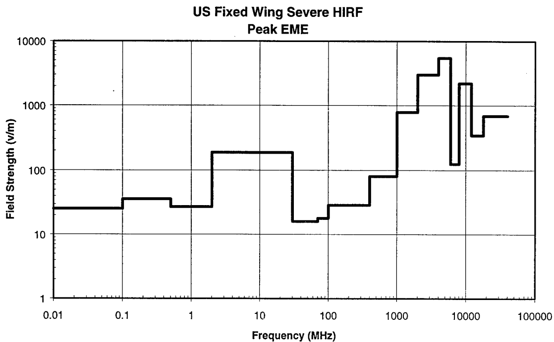
FIGURE 11 PEAK U.S. FIXED WING SEVERE ENVIRONMENT
