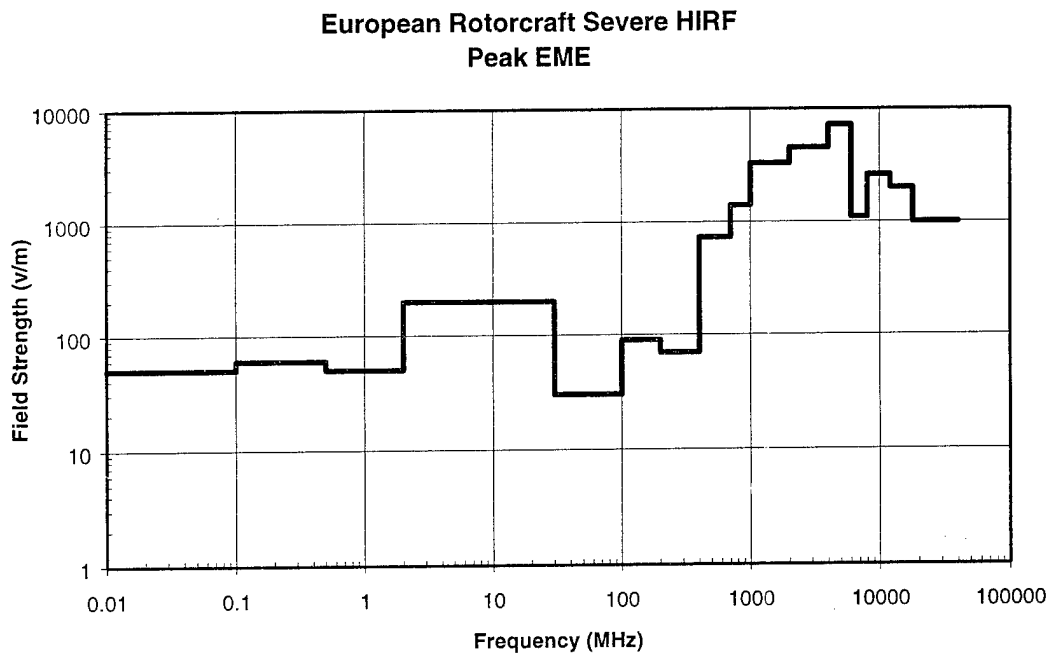
FIGURE 17 PEAK EUROPEAN ROTORCRAFT SEVERE ENVIRONMENT
