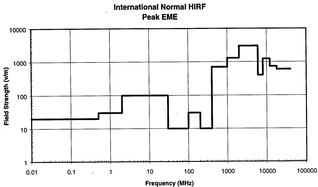
FIGURE 31 PEAK INTERNATIONAL NORMAL ENVIRONMENT
