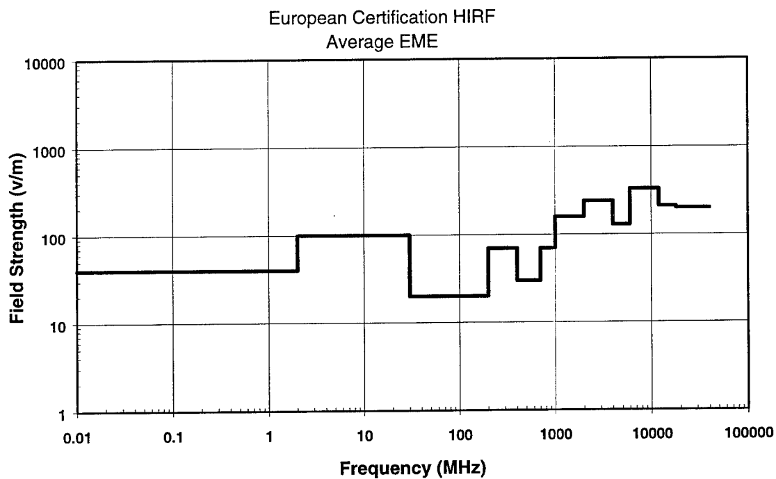
FIGURE 22 AVERAGE EUROPEAN CERTIFICATION ENVIRONMENT
