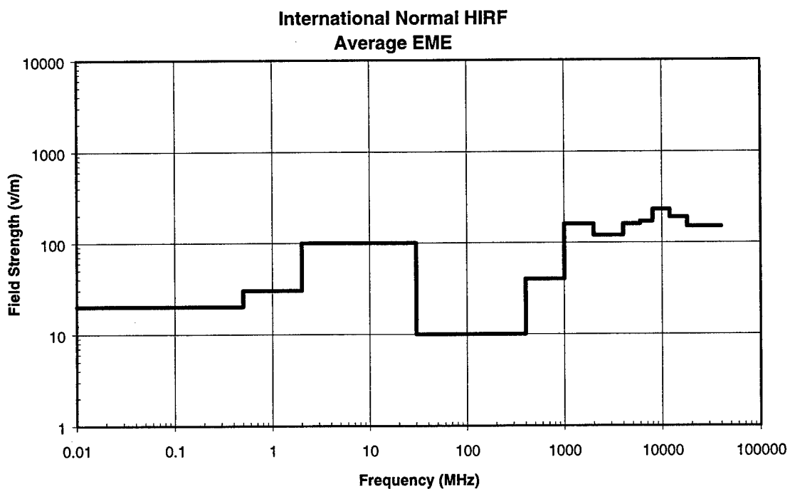
FIGURE 32 AVERAGE INTERNATIONAL NORMAL ENVIRONMENT
