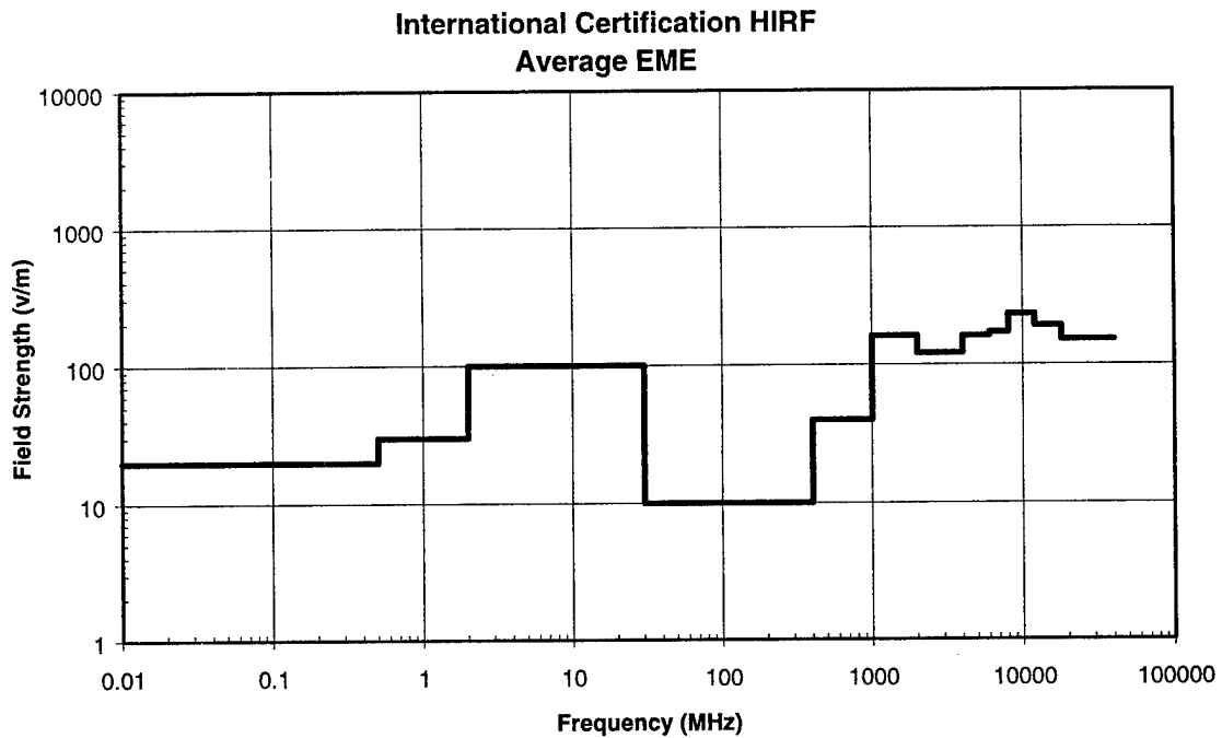
FIGURE 30 AVERAGE INTERNATIONAL CERTIFICATION ENVIRONMENT
