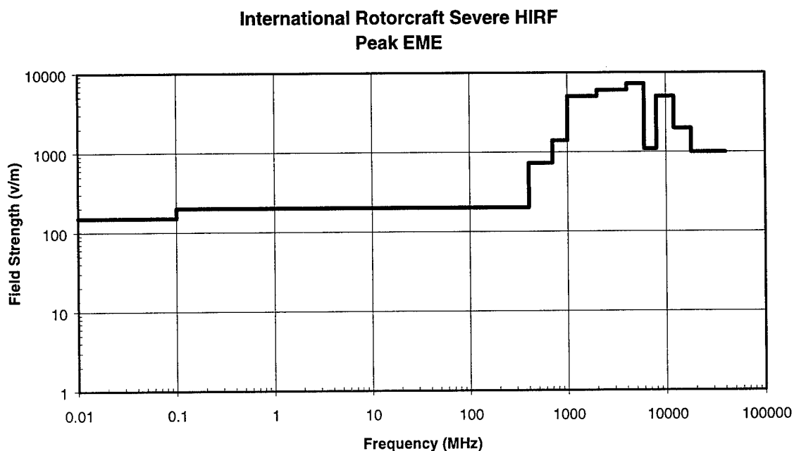
FIGURE 25 PEAK INTERNATIONAL ROTORCRAFT SEVERE ENVIRONMENT
