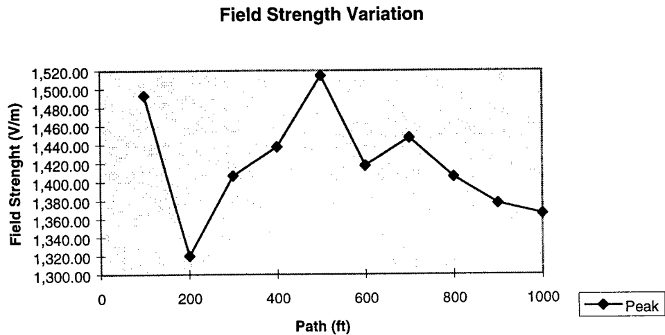
FIGURE 8 EXAMPLE OF NEAR-FIELD STRENGTH
