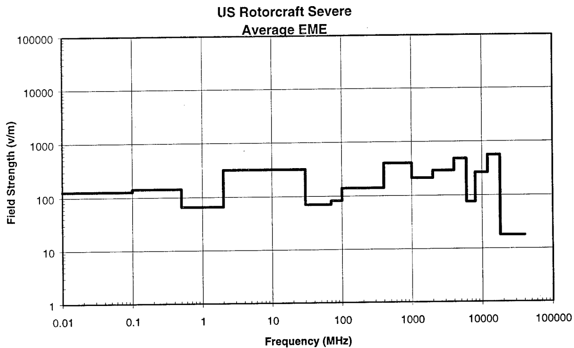
FIGURE 10 AVERAGE U.S. ROTORCRAFT SEVERE ENVIRONMENT
