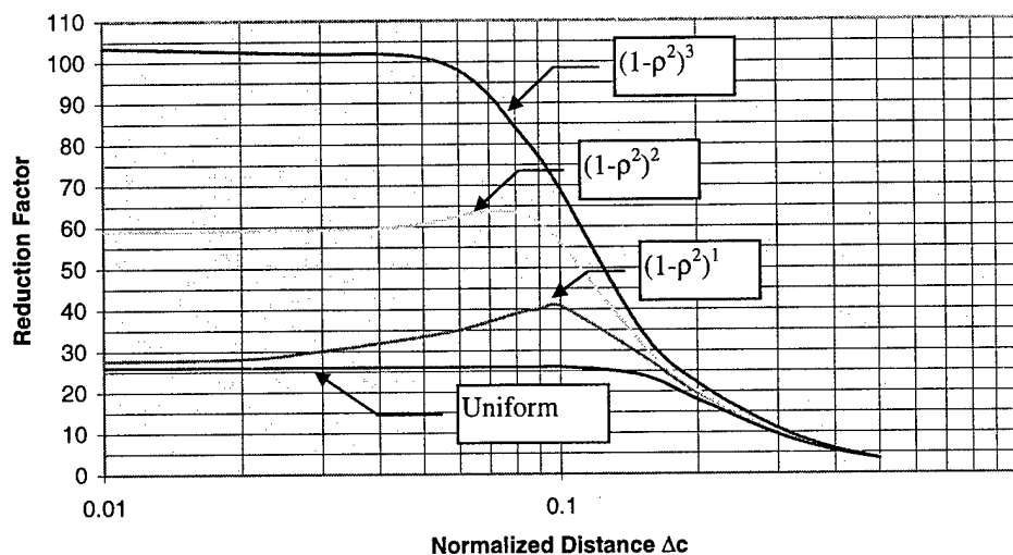
FIGURE 4 NEAR-FIELD CORRECTION FACTORS FOR CIRCULAR APERTURES
