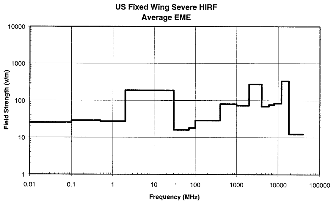
FIGURE 12 AVERAGE U.S. FIXED WING SEVERE ENVIRONMENT
