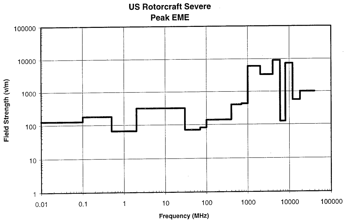
FIGURE 9 PEAK U.S. ROTORCRAFT SEVERE ENVIRONMENT
