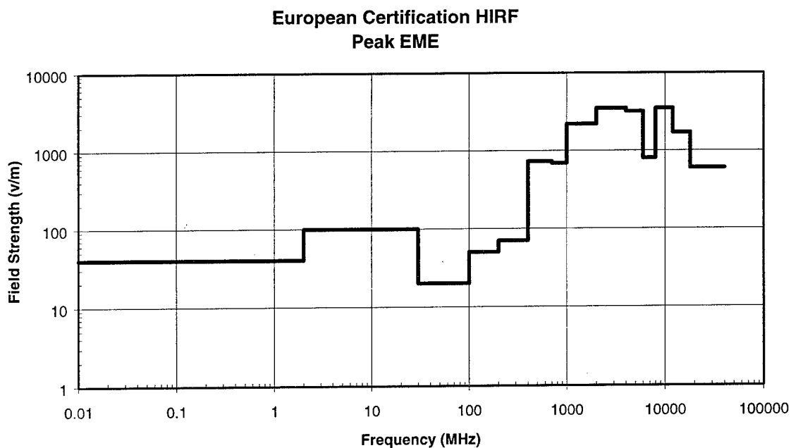
FIGURE 21 PEAK EUROPEAN CERTIFICATION ENVIRONMENT
