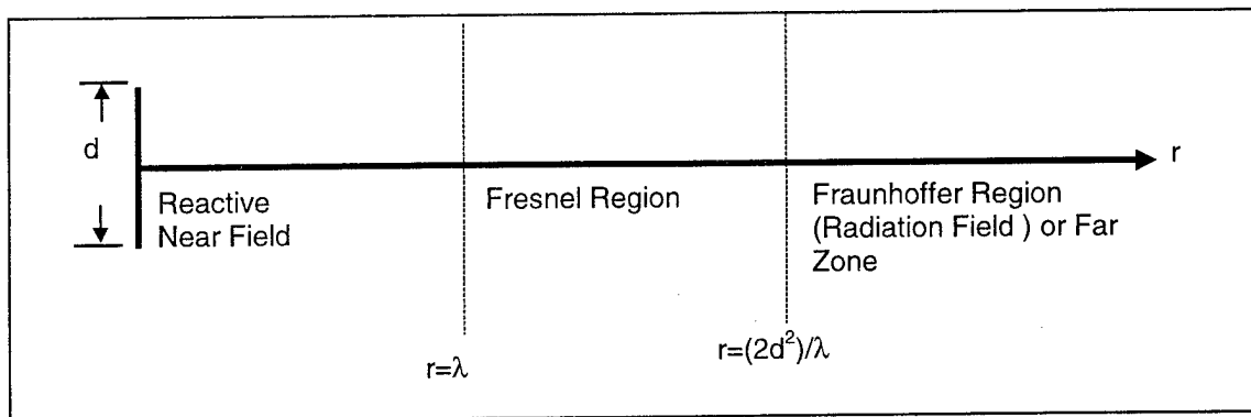
FIGURE 2 ANTENNA FIELD REGION
