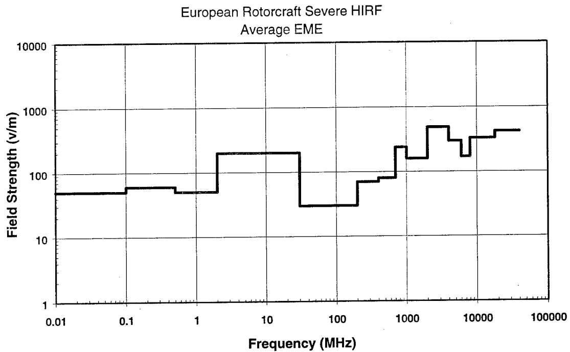
FIGURE 18 AVERAGE EUROPEAN ROTORCRAFT SEVERE ENVIRONMENT
