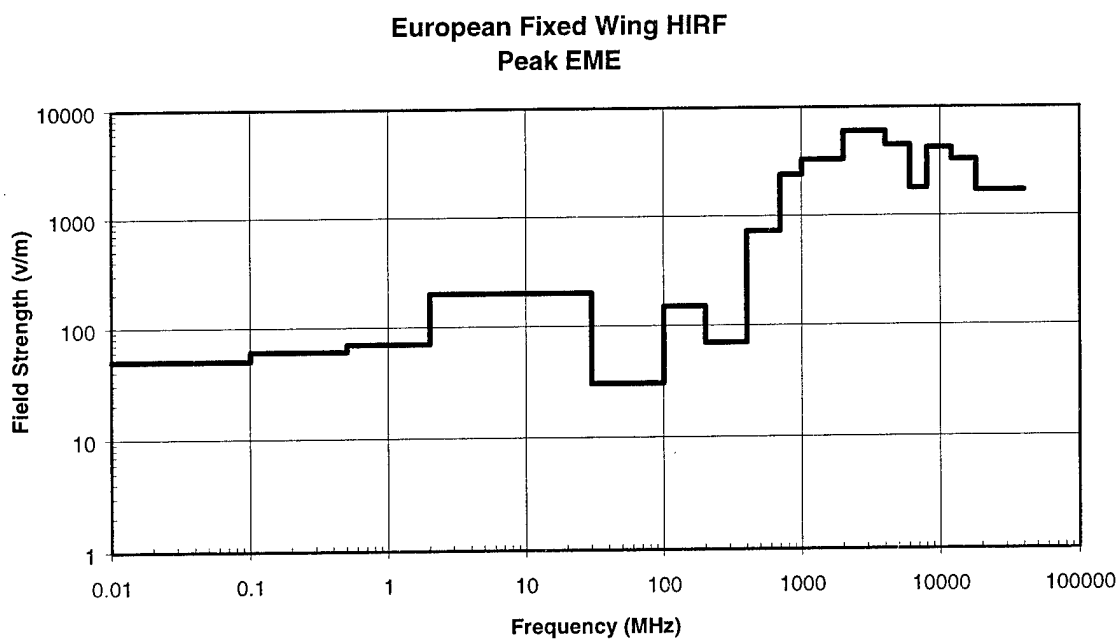
FIGURE 19 PEAK EUROPEAN FIXED WING SEVERE ENVIRONMENT
