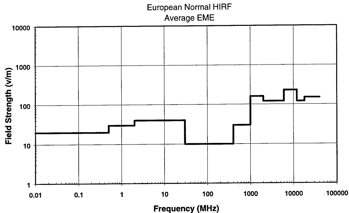
FIGURE 24 AVERAGE EUROPEAN NORMAL ENVIRONMENT
