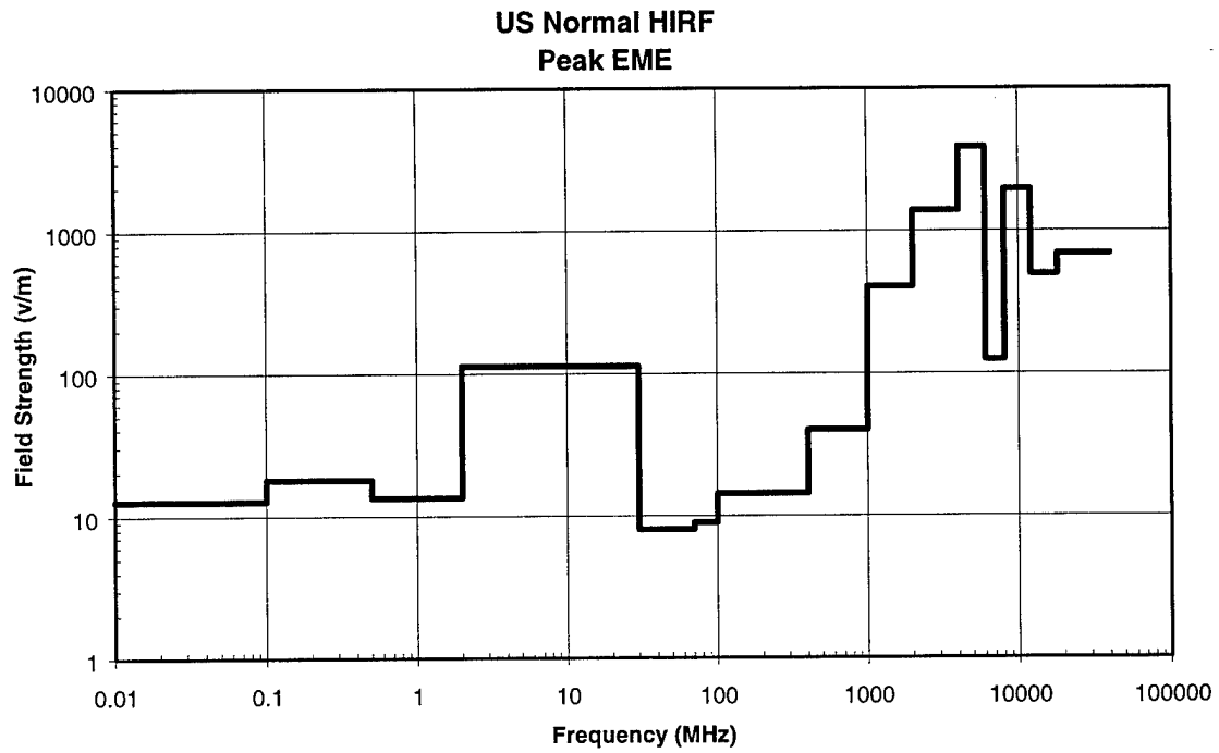
FIGURE 15 PEAK U.S. NORMAL ENVIRONMENT
