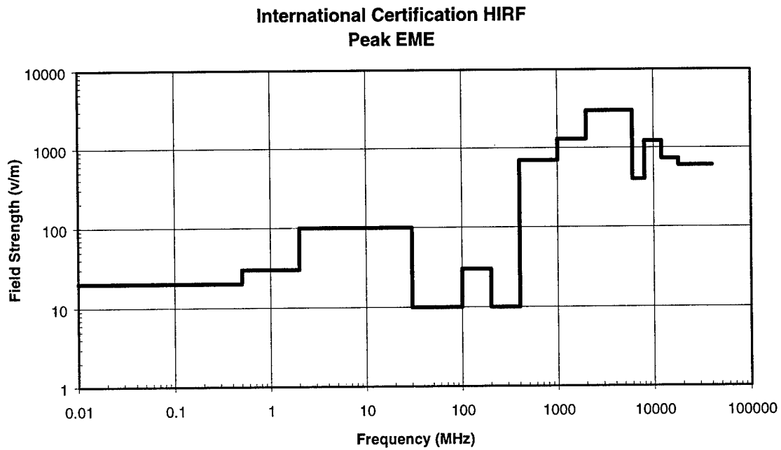
FIGURE 29 PEAK INTERNATIONAL CERTIFICATION ENVIRONMENT
