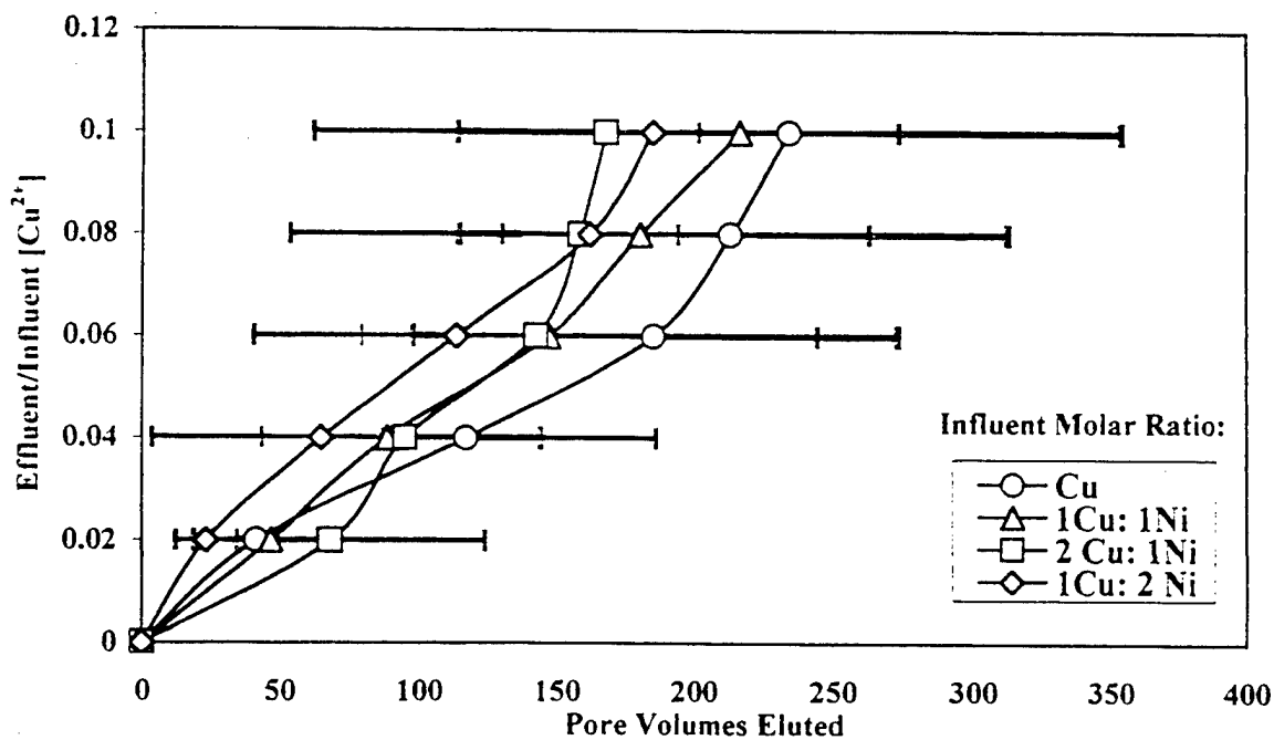
Figure 4-15. Copper breakthrough in a Cu 2+ and Ni 2+ bisolute system. Curves obtained with Carboxen-1011™ and a constant flow rate of 300 mL/min in the flow through experiments. Error bars represent a standard deviation about a triplicate mean.
