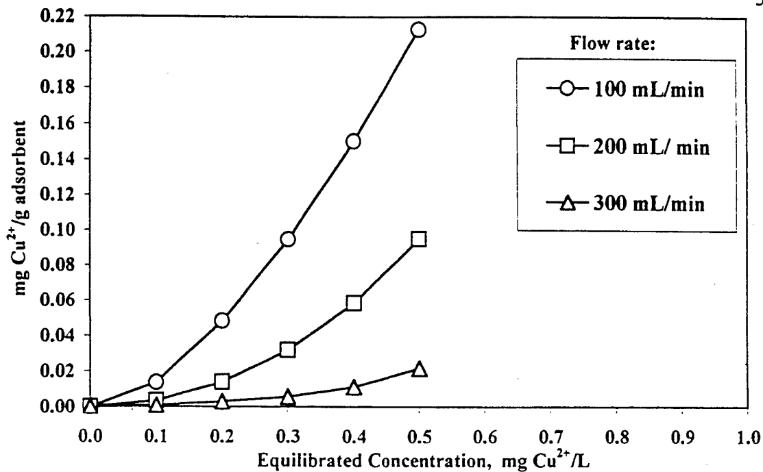
Figure 4-8. Adsorption isotherms obtained with Supelcarb™ as calculated by the Burgisser Model for a constant influent concentration of Cu 2+ of 5 mg Cu 2+ /L in the flow through experiments.
