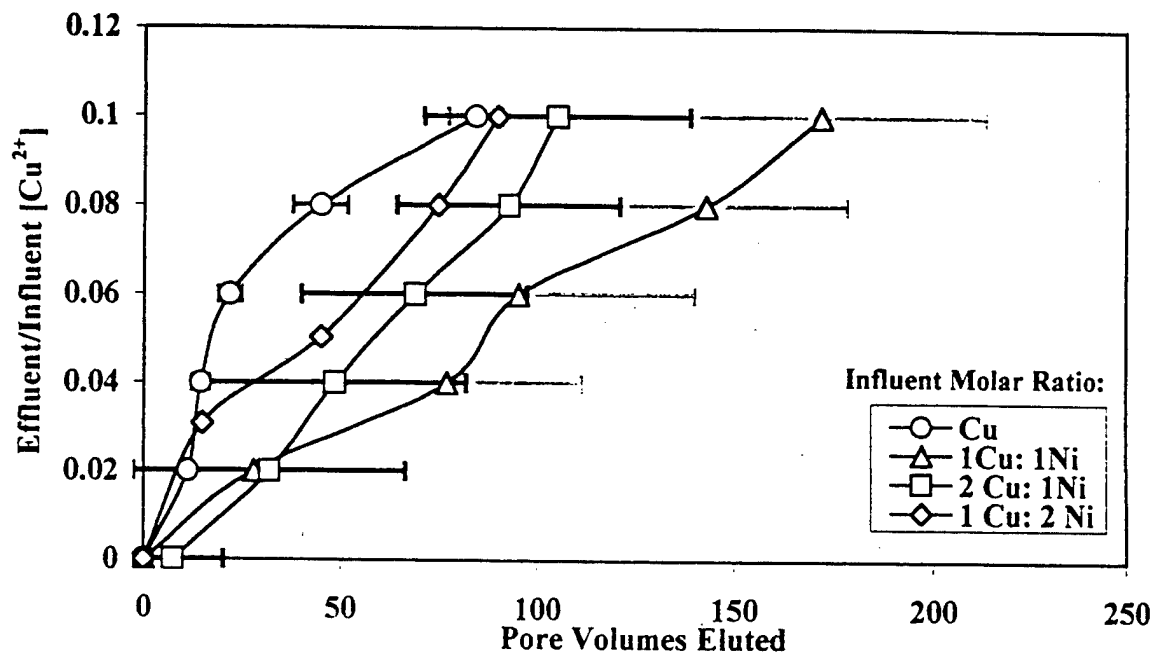
Figure 4-14. Copper breakthrough in a Cu 2+ and Ni 2+ bisolute system. Curves obtained with Supelcarb™ and a constant flow rate of 300 mL/min in the flow through experiments. Error bars represent a standard deviation about a triplicate mean.
