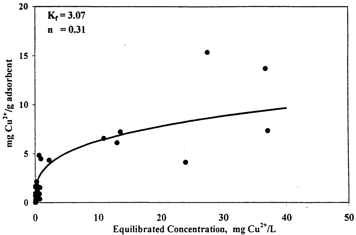
Figure 4-1. Copper adsorption isotherm obtained with Supelcarb™ in the batch experiments.
