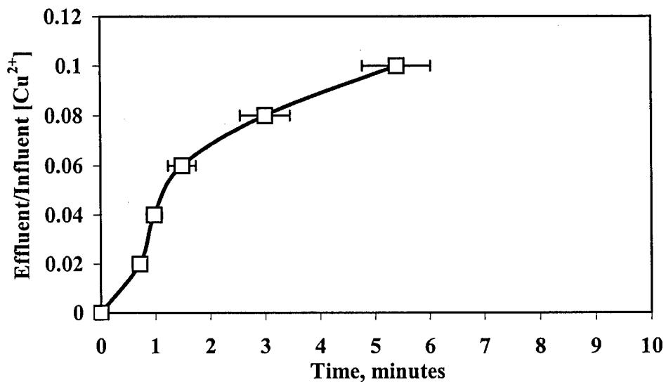
Figure 3-6. Representative average time to breakthrough curve. The graph shows reduction of the triplicate data set of Supelcarb TM at an influent concentration of 5 mg Cu 2+ /L and constant flow rate of 300 mL/min to one average break through curve. Error bars represent the standard deviation about the mean time value.
