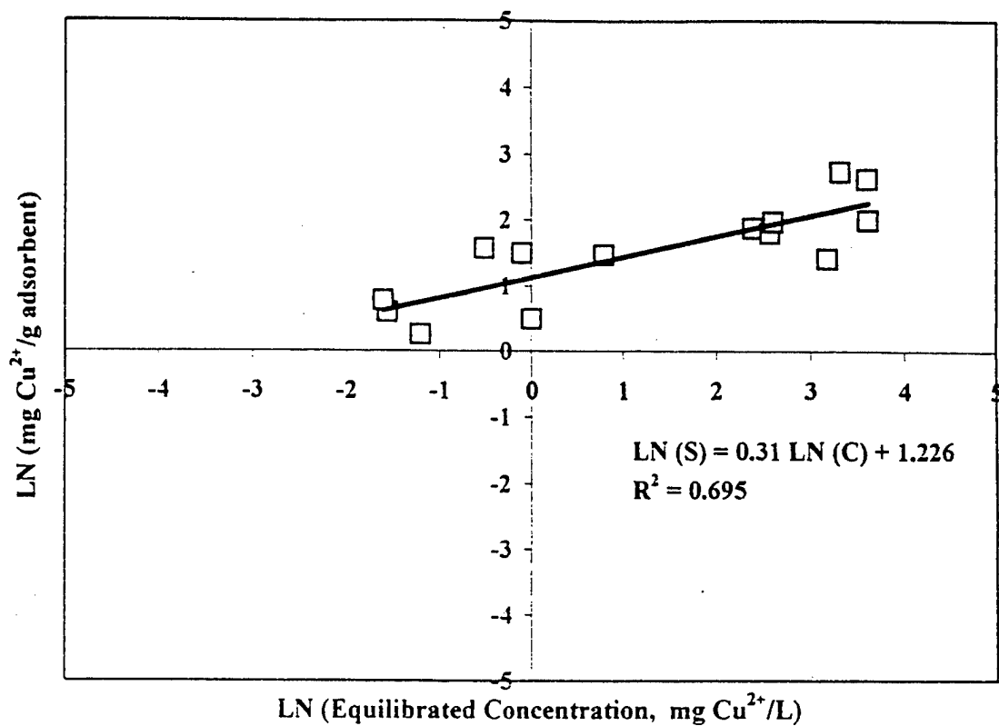
Figure 4-3. Freundlich adsorption isotherm obtained with Supelcarb TM in the batch experiments.
