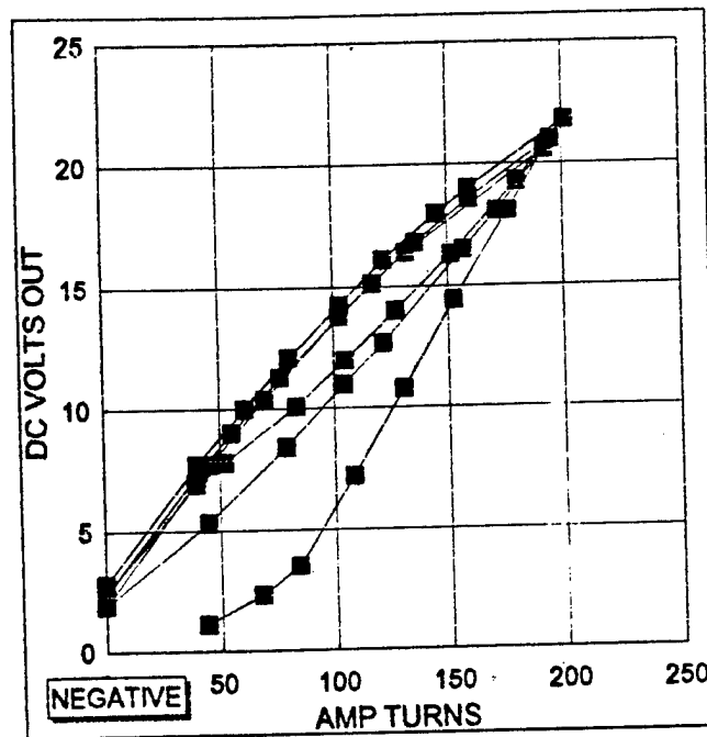
FIGURE 20 Typical Alternator Magnetization Curve Showing Hysteresis and Residual Magnetism (Truck Style Alternator, Field Coil 280 Turns)
