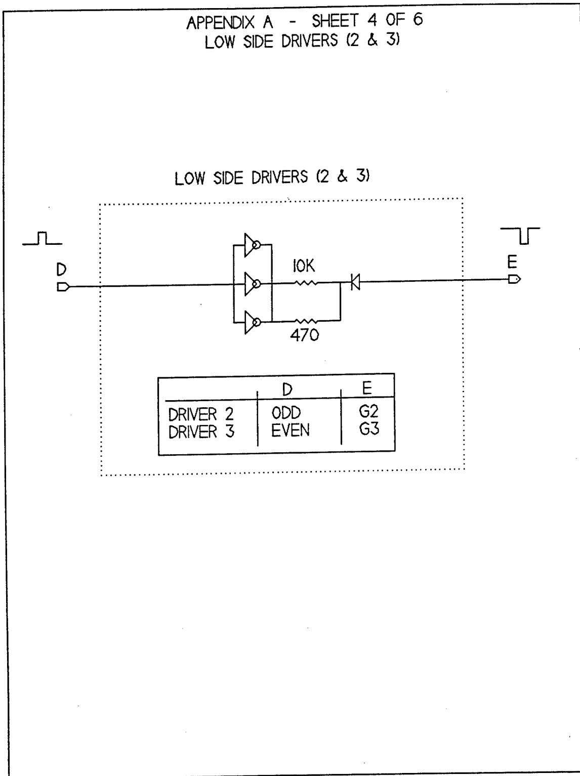
FIGURE A-4 Low Side Driver Circuit
