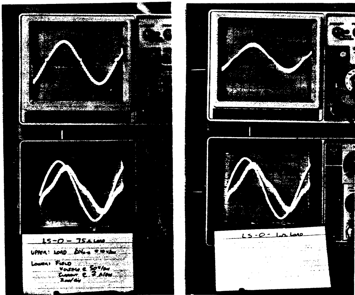
FIGURE 25 COMMUTATION
