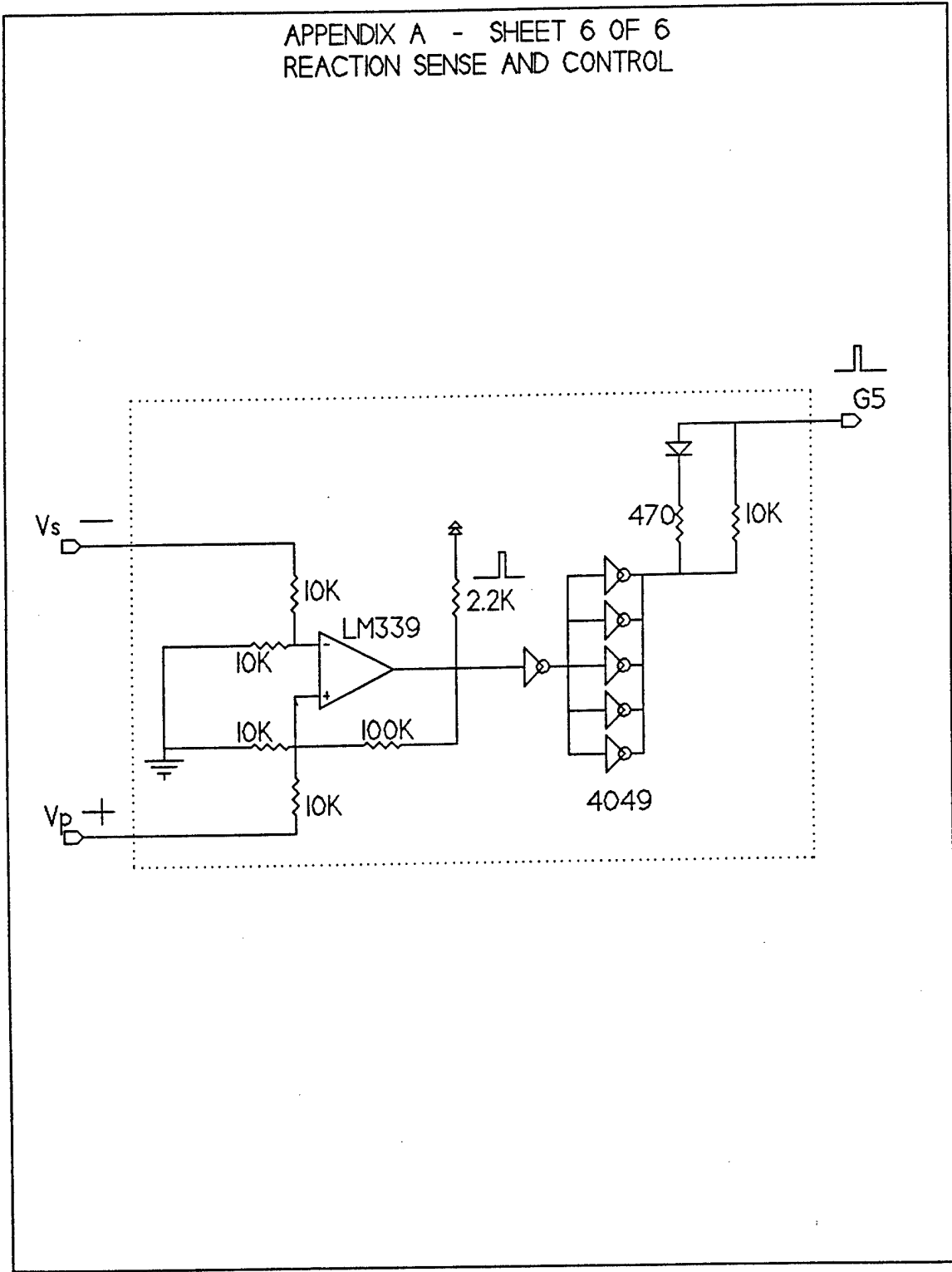
FIGURE A-6 Reaction Sense and Control Circuit
