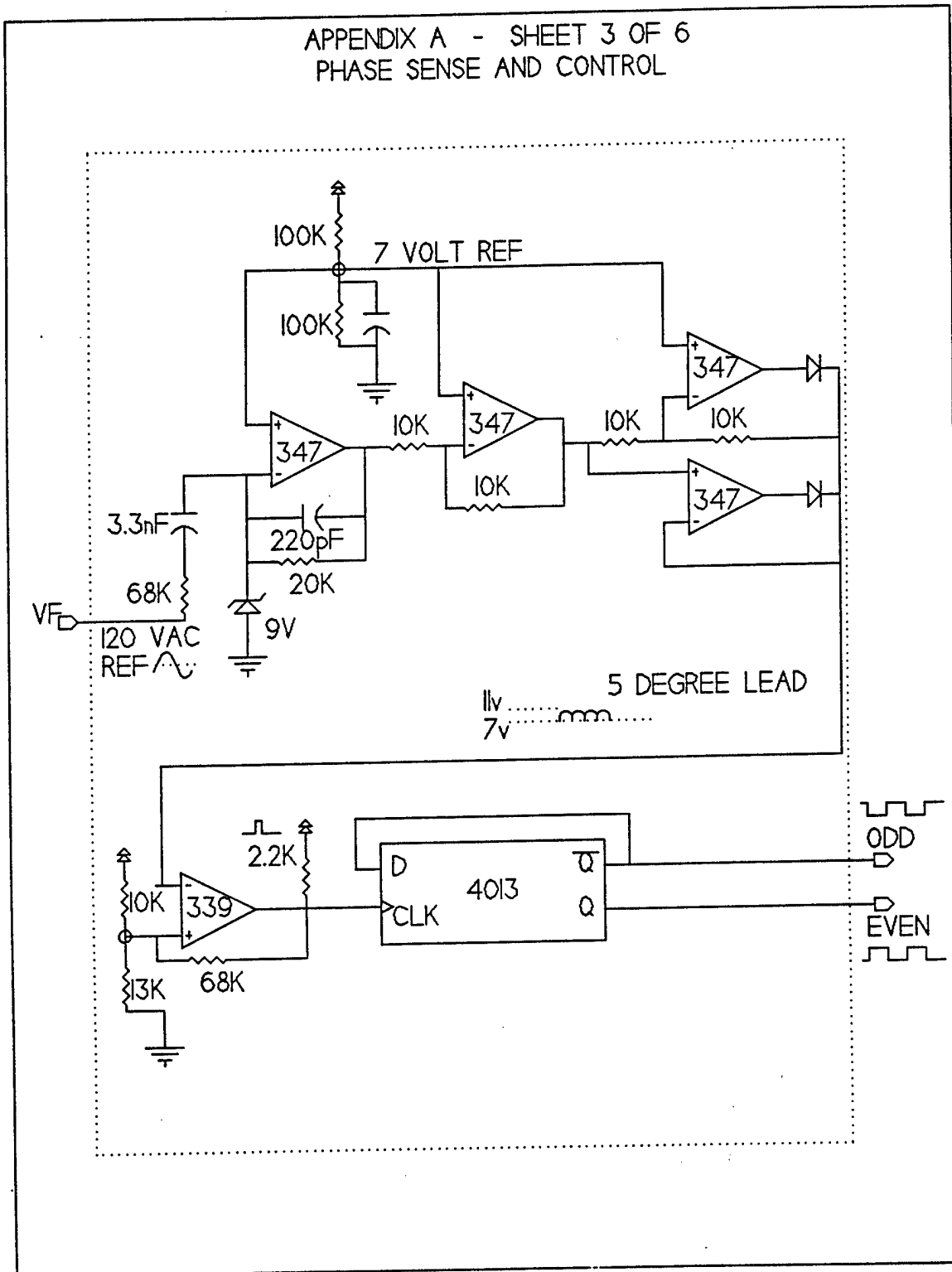
FIGURE A-3 Phase and Sense Control Circuit
