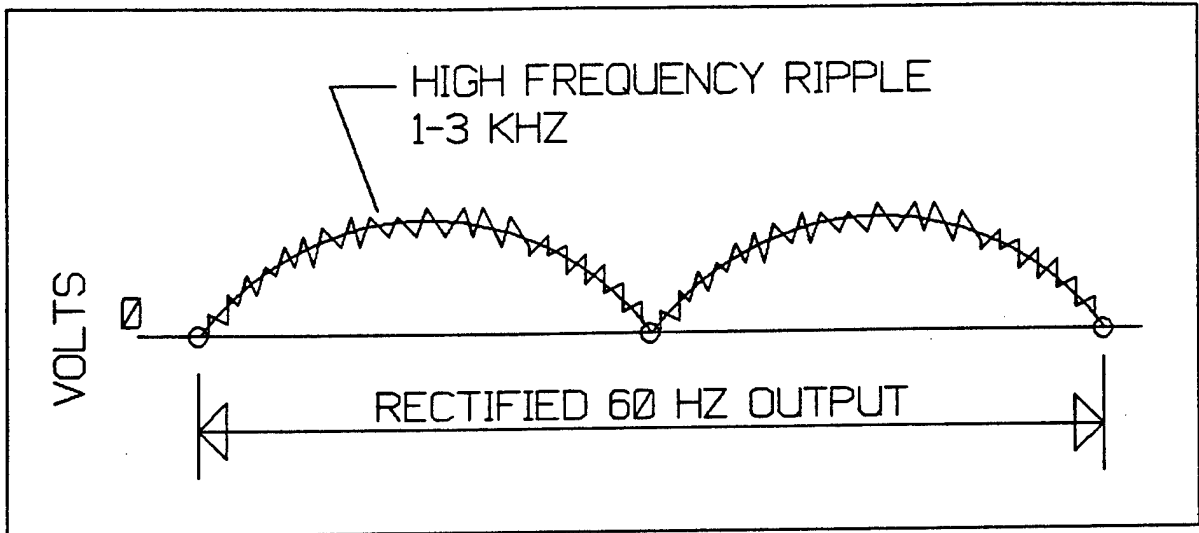
FIGURE 2 Modulated Output of High Frequency Alternator to Provide Rectified 60 Hz Waveform.
