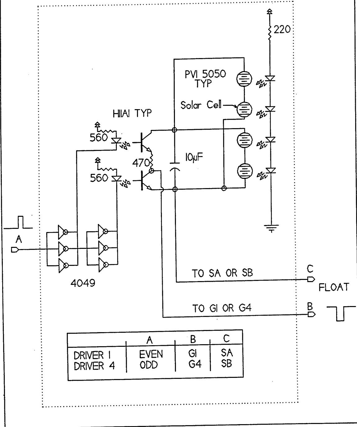
FIGURE A-5 High Side Driver Circuit
