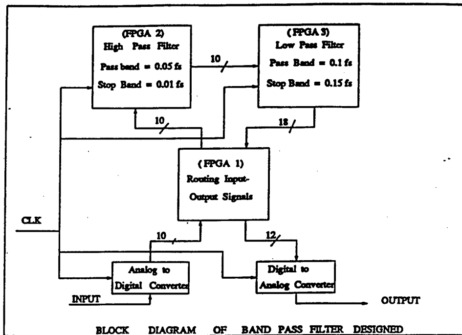
Figure 5.6 - The Block Diagram of Band Pass Filter
