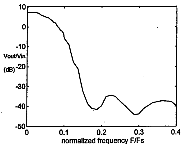
Figure 5.13 - Experimental Frequency Response (Fixed-Point Coefficients)
