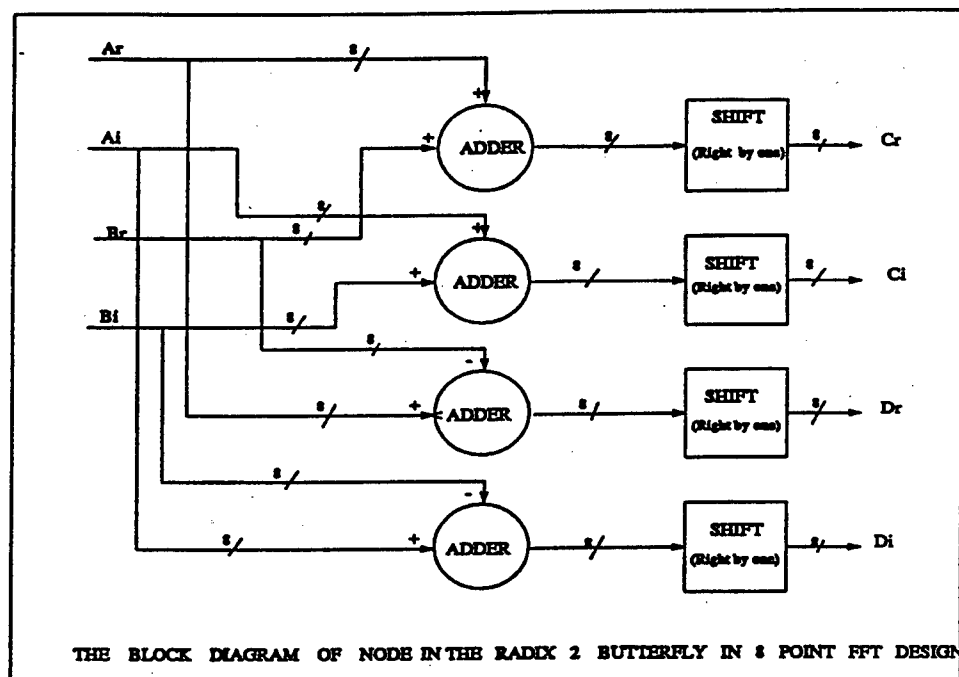
Figure 5.19 - The Block Diagram of Node element used in 8 point FFT
