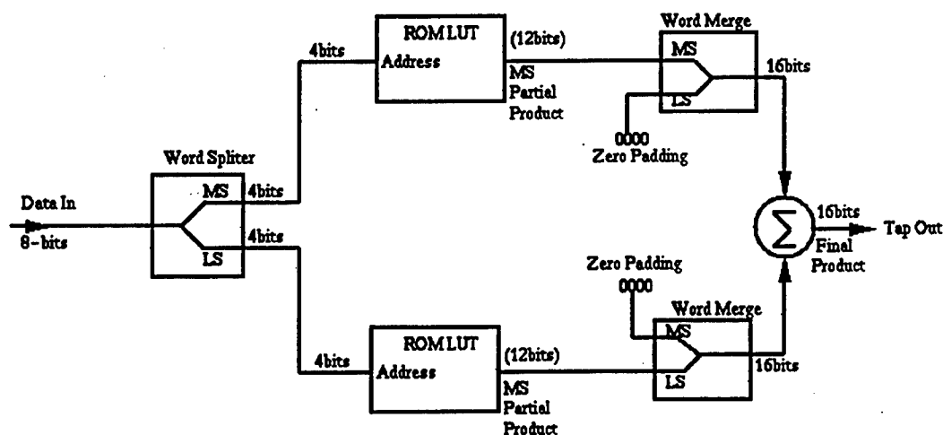
Figure 5.11 - Internal structure of LUT
