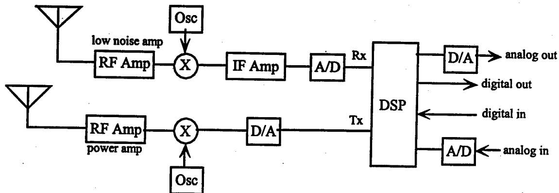
Figure 2.1 - Software Radio System
