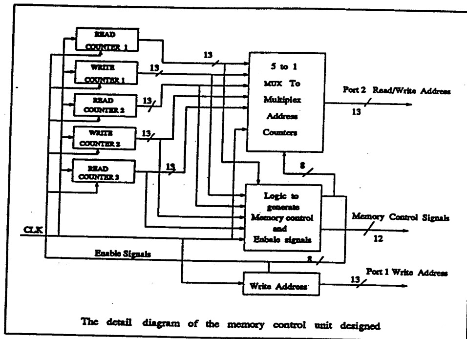
Figure 5.24 - Diagram of memory control logic unit
