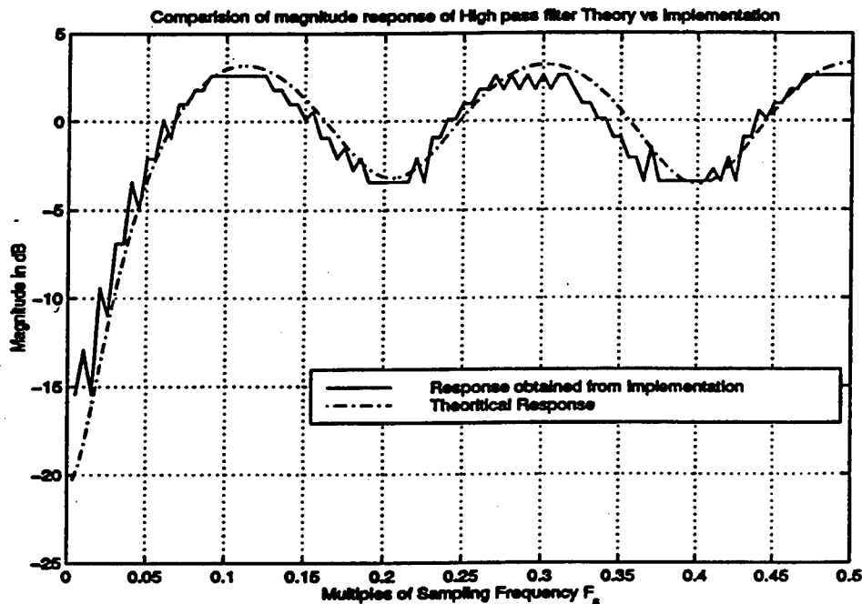
Figure 5.5 - Comparison of Magnitude Response of High Pass Filter
