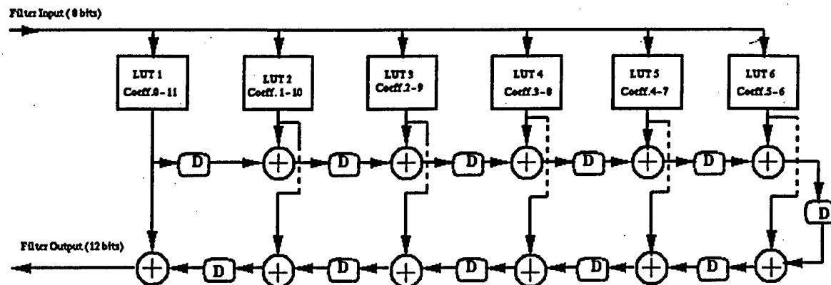
Figure 5.10 - Block diagram of the FIR Filter
