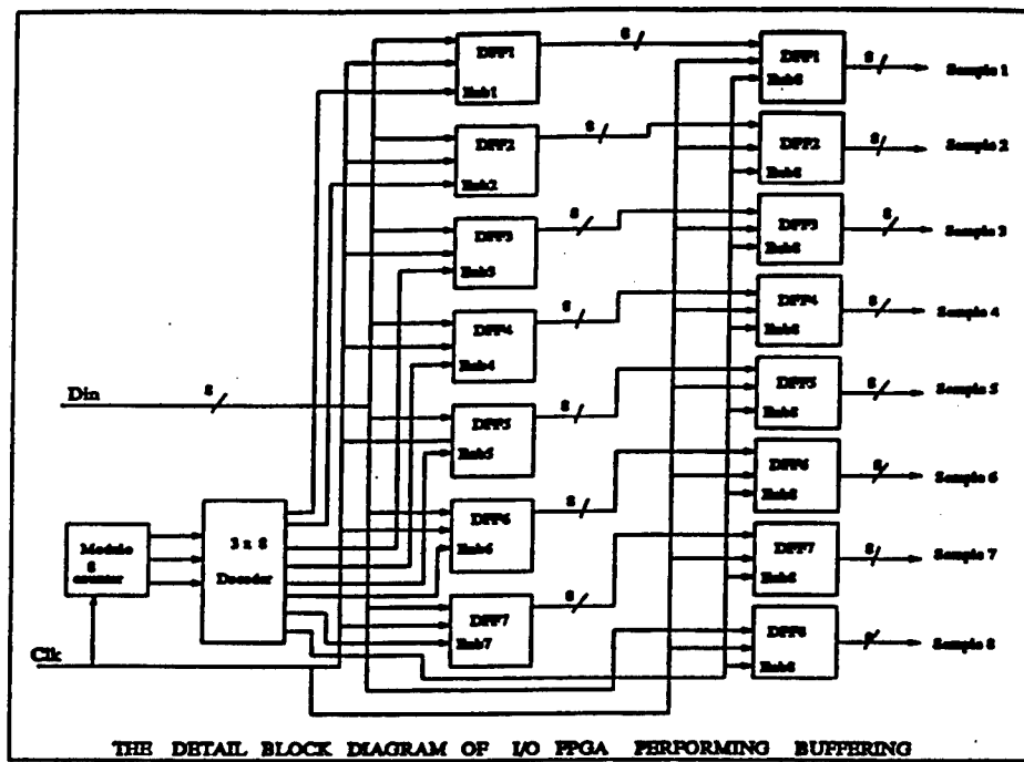
Figure 5.20 - The Block Diagram of Buffering Stage used in 8 point FFT
