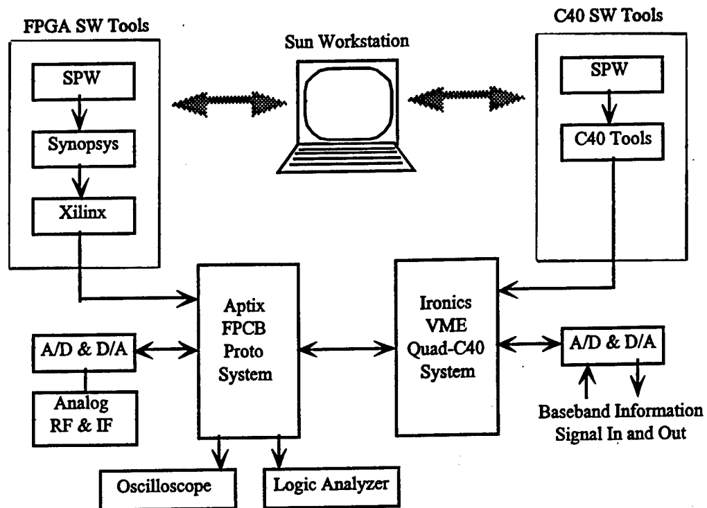
Figure 2-3: Rapid Prototyping Configuration
