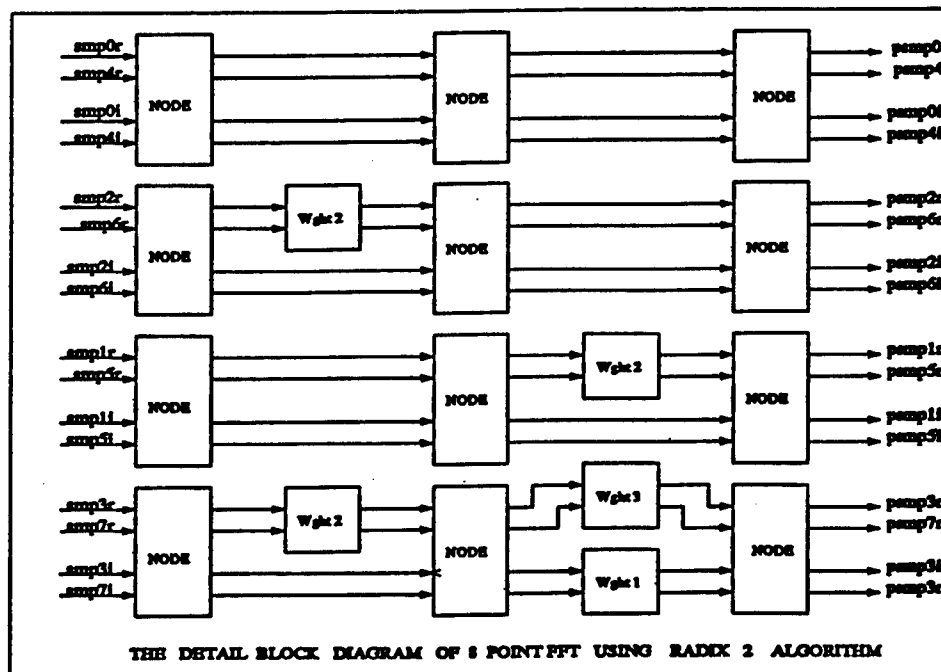
Figure 5.18 - The Detail Block Diagram of 8-point FFT using Radix 2 Algorithm
