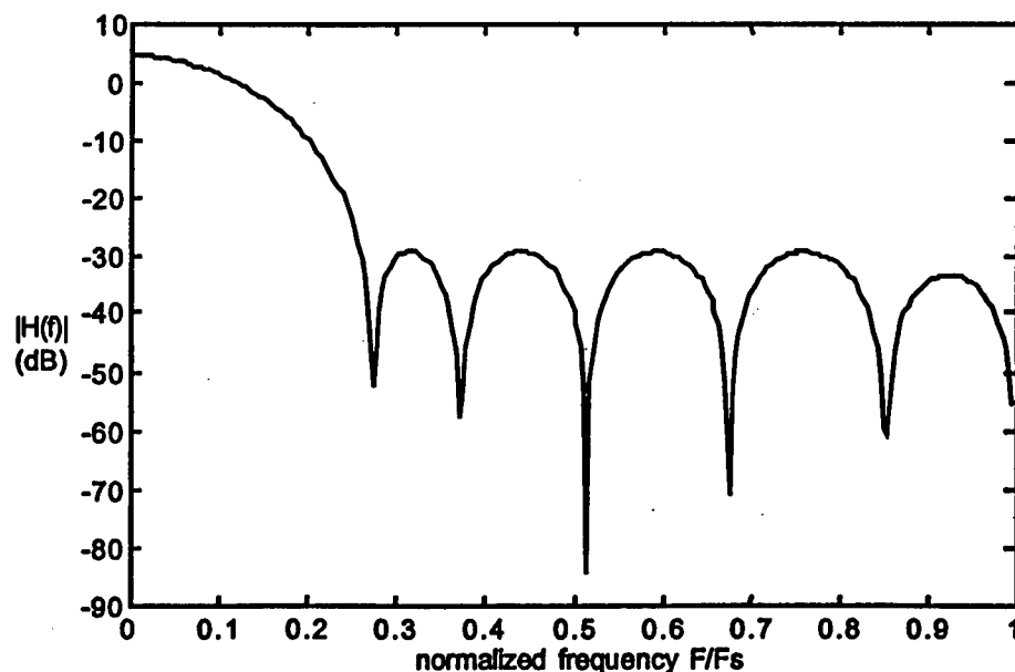
Figure 5.12 - Theoretical Frequency Response
