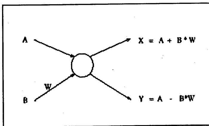
The Radix 2 Butterfly Element
