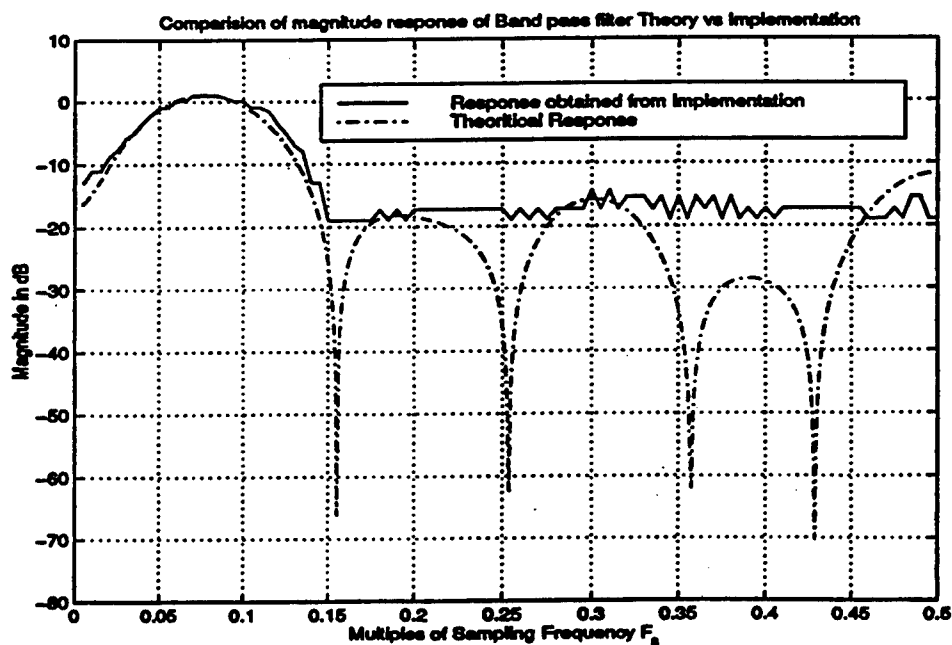
Figure 5.7 - Comparison of Magnitude Response of Band-Pass Filter
