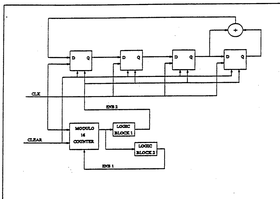
Figure 5.15 - Detail Block Diagram of PN Sequence Generator
