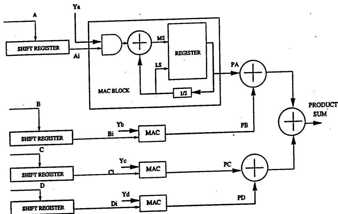
Figure 3.3 - Four-Product MAC Unit with Conventional Arithmetic
