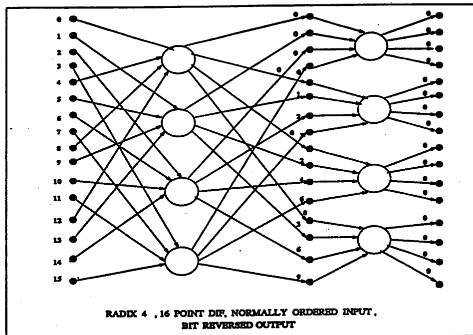
Figure 5.21 - Flow Diagram of 16 Point FFT
