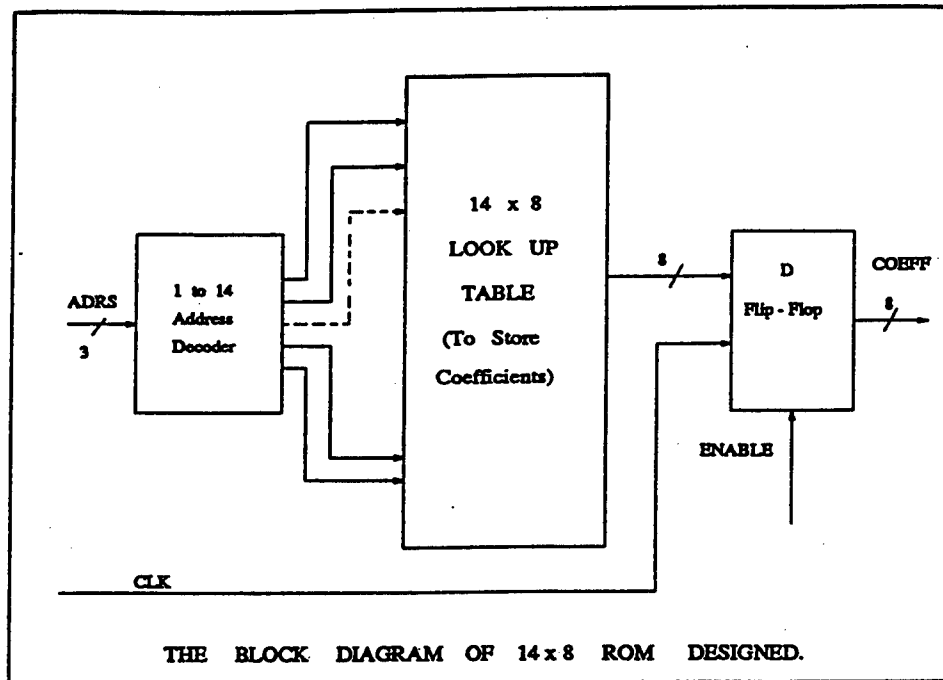
Figure 5.27 - The Block Diagram of Read Only Memory
