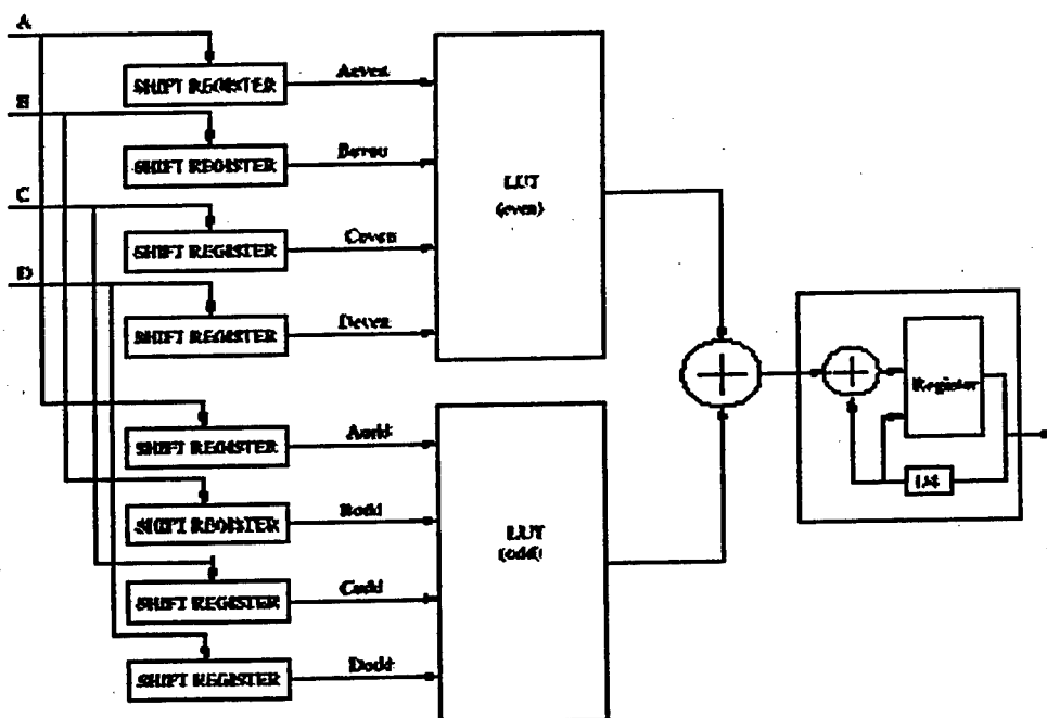
Figure 3.6 - 2-bit Parallel Distributed Arithmetic.
