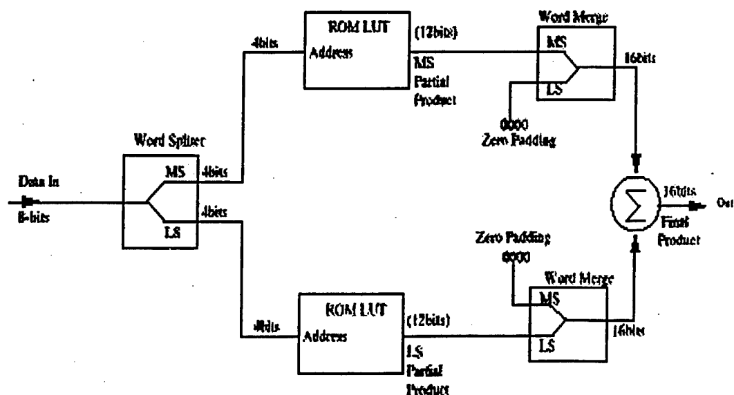
Figure 3.7 - Constant Coefficient Multiplier using LUT.
