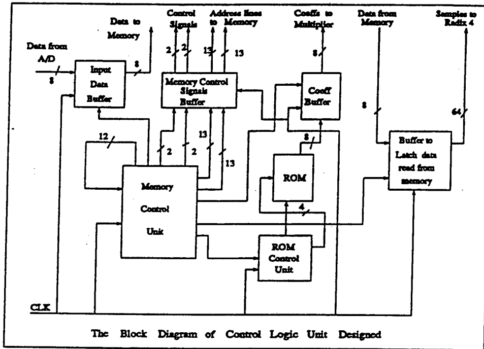
Figure 5.23 - Block diagram of Control Logic Unit
