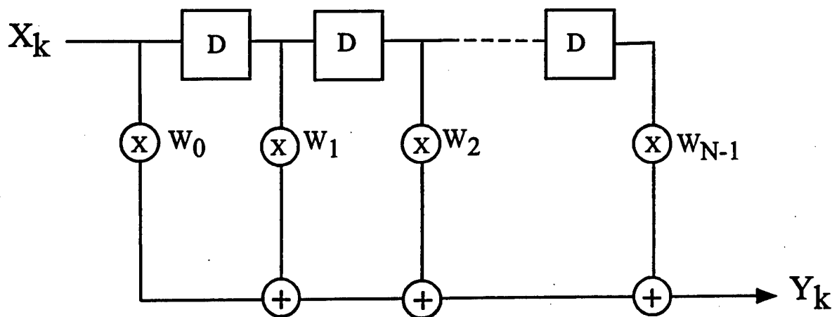
Figure 5.1 - Direct Form structure of an FIR filter
