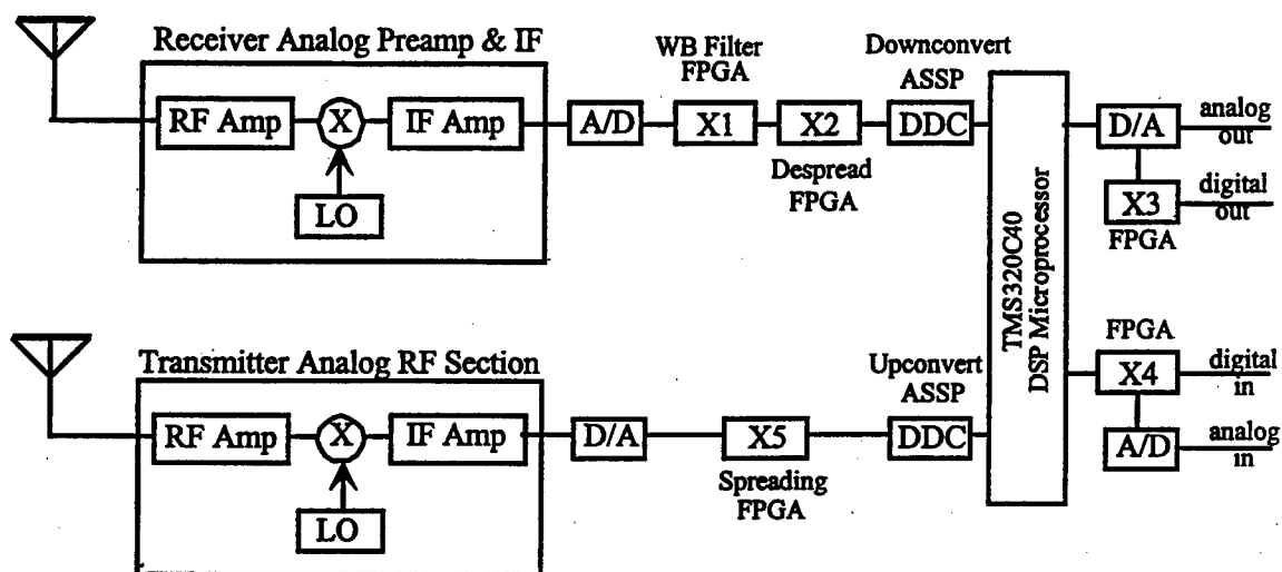
Figure 2-2: Tactical Radio Testbed
