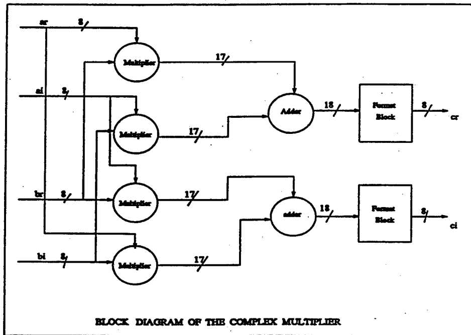
Figure 5.26 - The Block Diagram of Complex Multiplier
