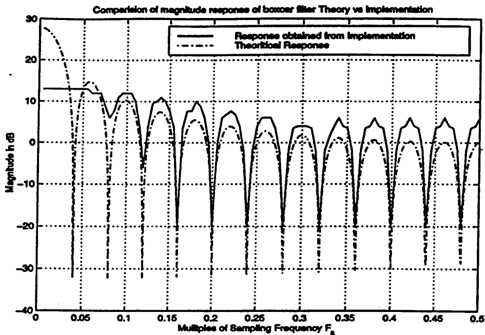
Figure 5.9 - Comparison of Magnitude response of Box Car Filter
