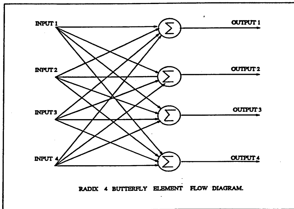
Figure 5.25 - The Flow Diagram of Radix 4 Butterfly Element
