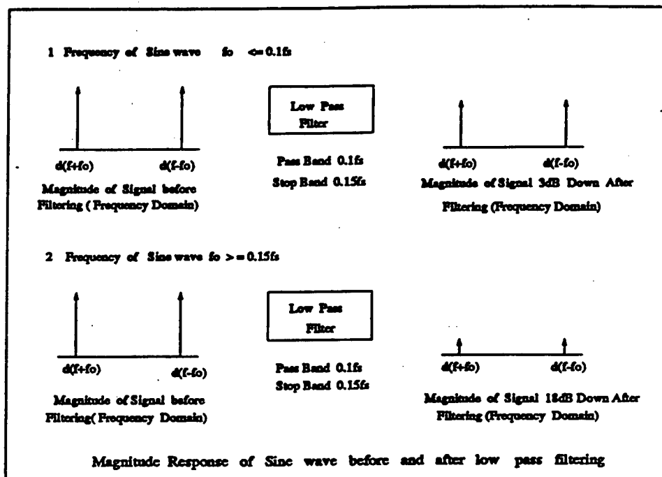
Figure 5.3: Theoretical Results: Low Pass Filtering
