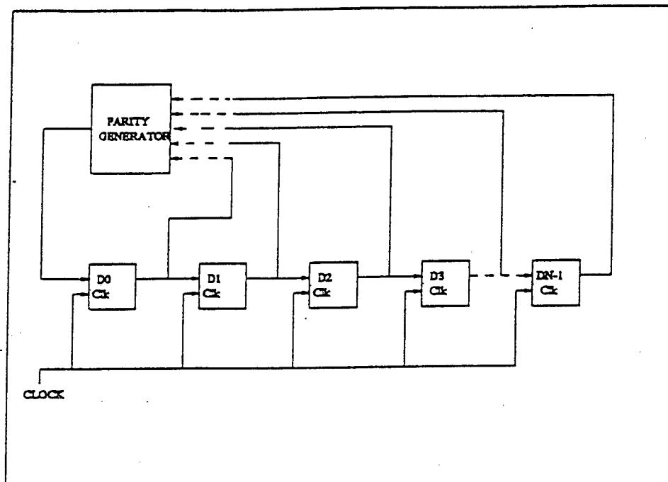
Figure 5.14 - Block Diagram of PN Sequence Generator
