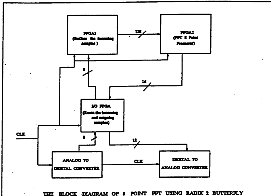
Figure 5.17 - The Block Diagram of Eight point FFT using Radix 2 Algorithm
