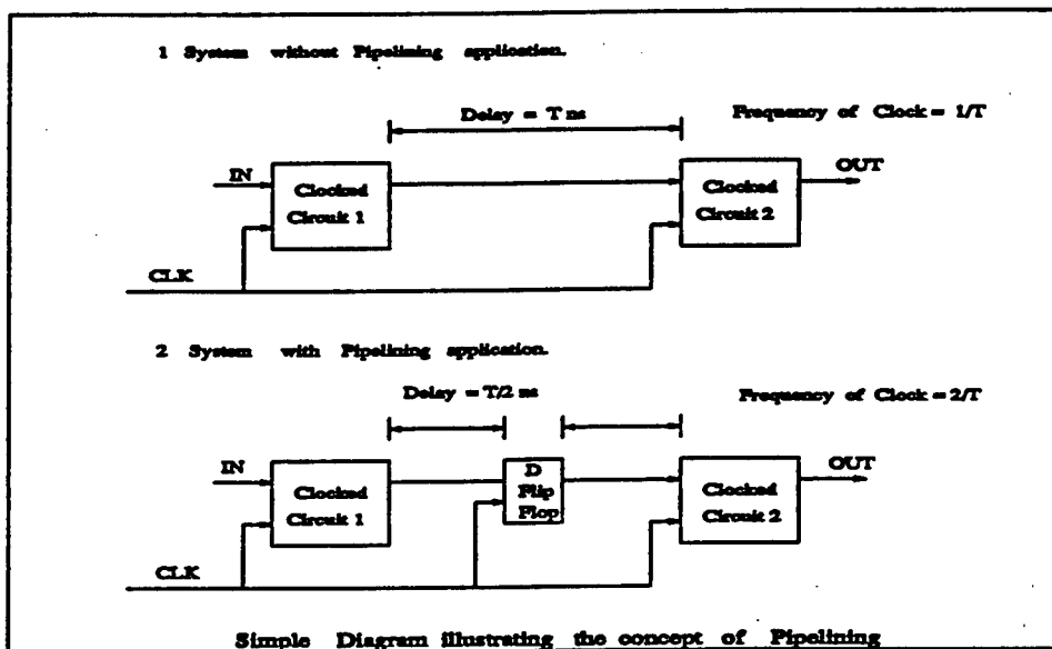
Figure 3.8 - The Pipelining Concept
