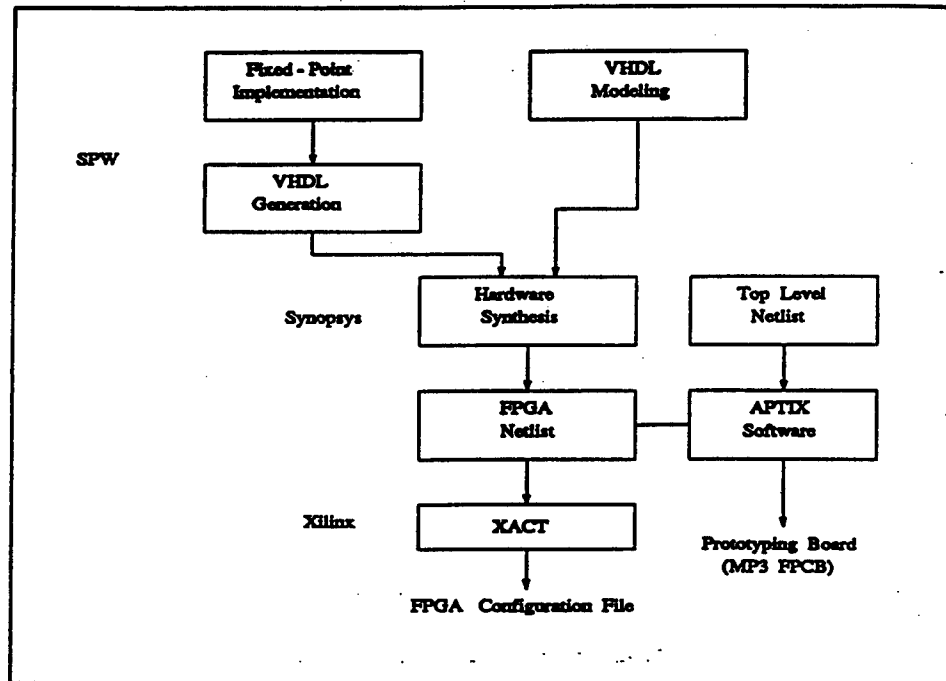
Figure 4.1 - Block Diagram of Rapid Prototyping Flow
