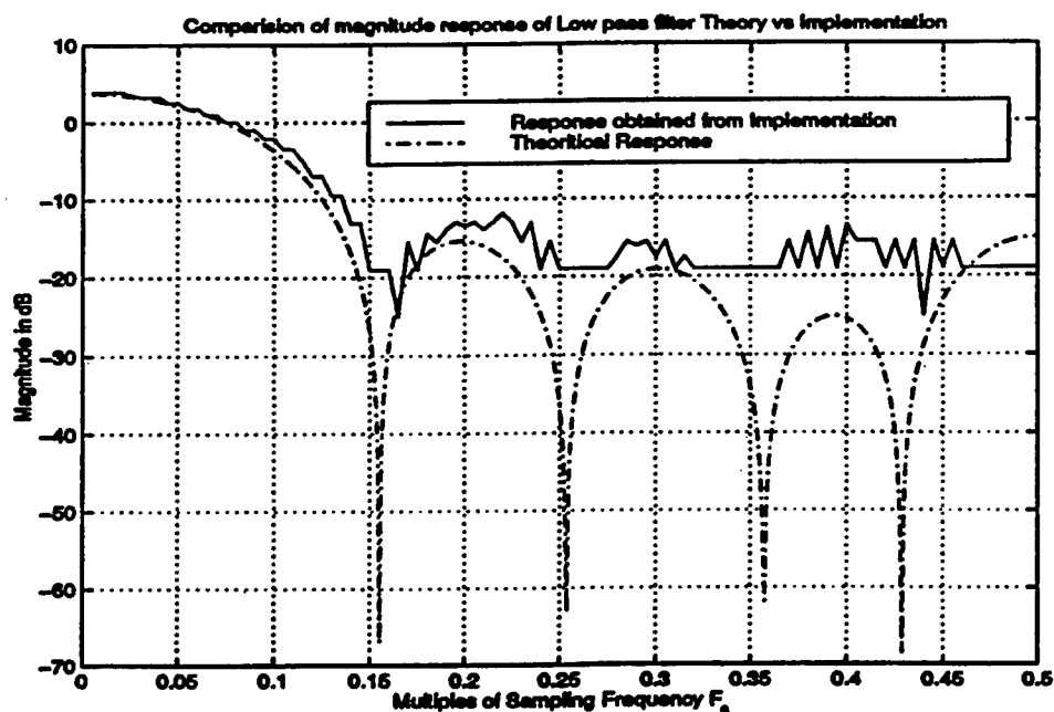
Figure 5.4: Comparison of Magnitude Response of Low Pass Filter
