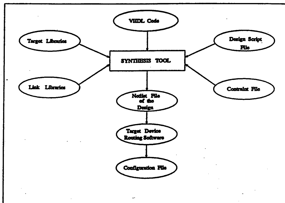
Figure 4.3 - Block Diagram of Synthesis Procedure
