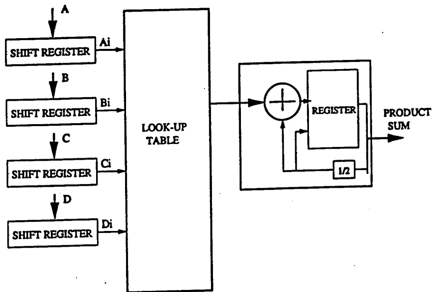
Figure 3.5 - A LUT Replaces the AND Gates & Adders in SDA
