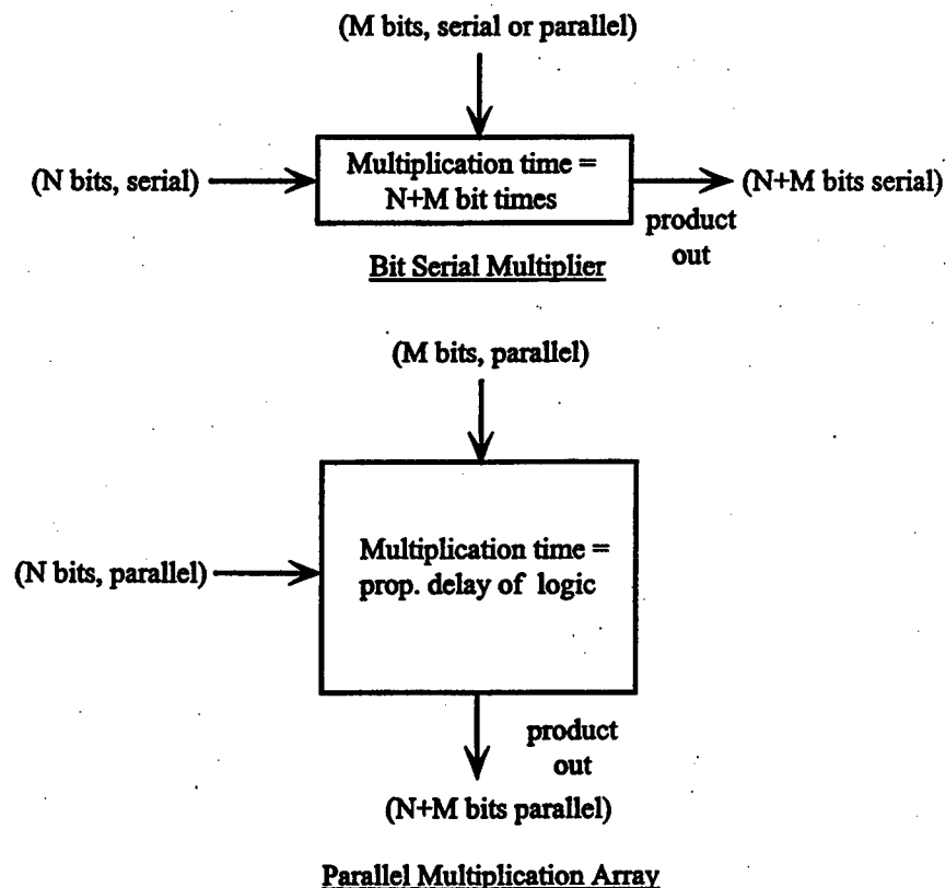
Figure 3.2 - Block Diagram of Basic Multiplier Alternatives
