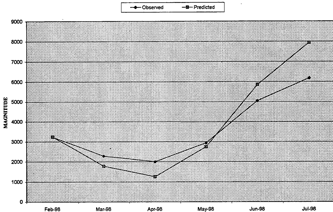
ARIMA 213 Process Back Forecasting Results
