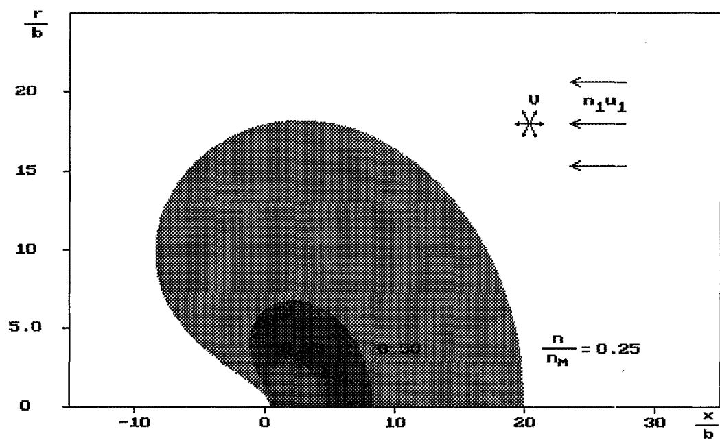
Fig.3 The lines of equal plasma concentration in the simmetry plane of the resulting plasma formations for spherically symmetrical gas expansion.
