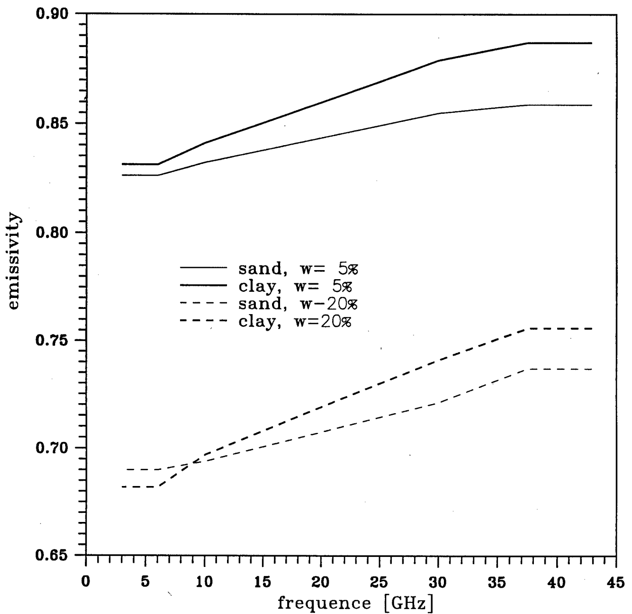
Fig.2.3.Spectral dependence of bare smooth land emissivity at different volumetric soil moisture w .
