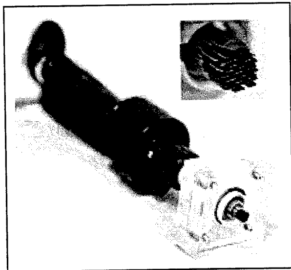
Figure 1. Mechanical punch device. Our punch device consists of 28 parallel blades banded together. These blades are connected to a steel piston is housed within a plastic handle. A piece of plexiglass is located above and perpendicular to the blades, and is used to align the device so that each blade is equidistant from the bottom of the well. A plunger located at the top of the device is connected to the steel piston. When depressed, the blades contact the well surface. A consistent level of downward force is applied to the blades by activation of an electromagnet. Increased magnification of the blades is illustrated in the inset.
