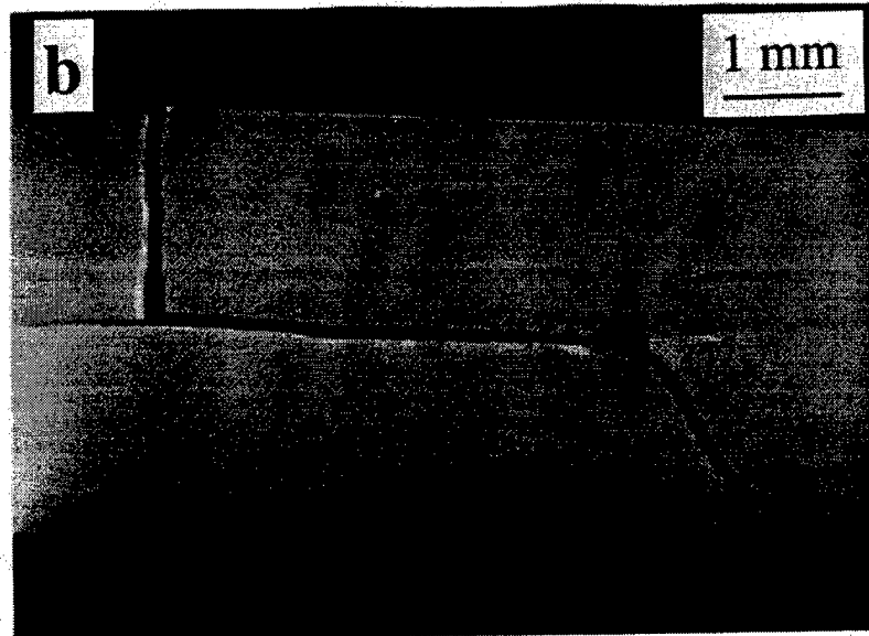
Figure 9: Optical micrographs for bifurcation phenomena: (a) short bifurcation before crack reinitiation, (0.5 of MZ; 100 \mu m thin layer thickness) and (b) extensive bifurcation (0.6 of MZ; 100 \mu m thin layer thickness).
