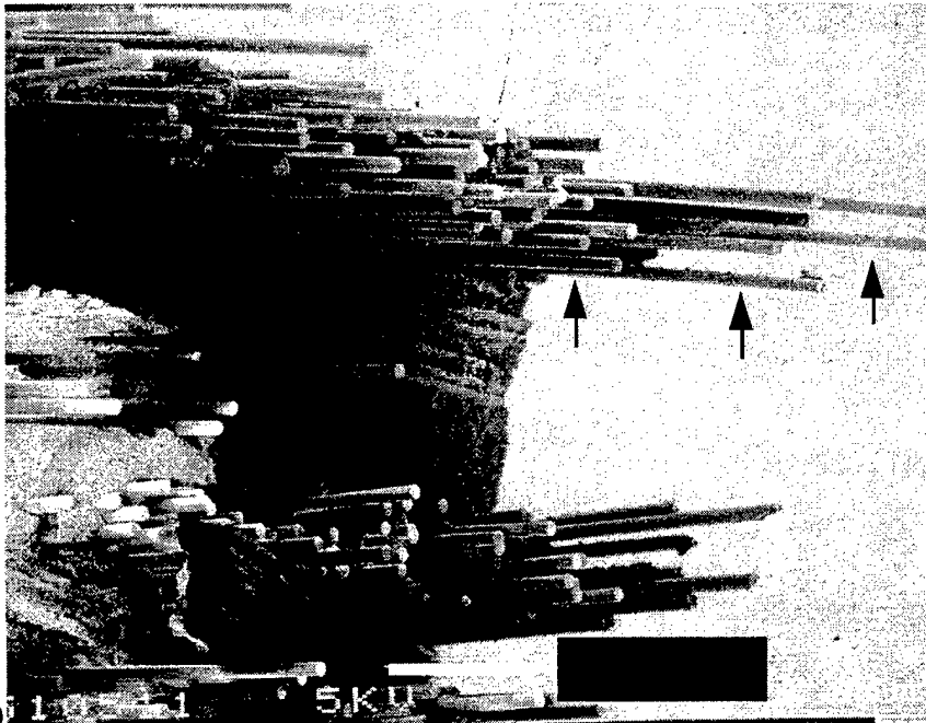
Figure 10. Fracture surface near the tensile surface of a 0/90° fiber orientation composite containing 70v% cubic ZrO_2 (8m% Y_2O_3 )/30v% mullite sintered at 1200°C for 5 hours in HCl. The composite was tested in the in-plane 3-point bending configuration. Large amounts of fiber pullout are evident with little coordinated fracture. (a) Low magnification showing general extent of fiber pullout, (b) Higher magnification, arrows show fibers that failed independently and pulled free with disintegration of the surrounding matrix.
