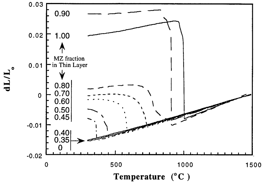
Figure 5: Dilatometry curves obtained during cooling for monolithics composed of different mixtures of TZ and MZ powers (5 MZ indicated in figure) and heated to 1500 °C.
