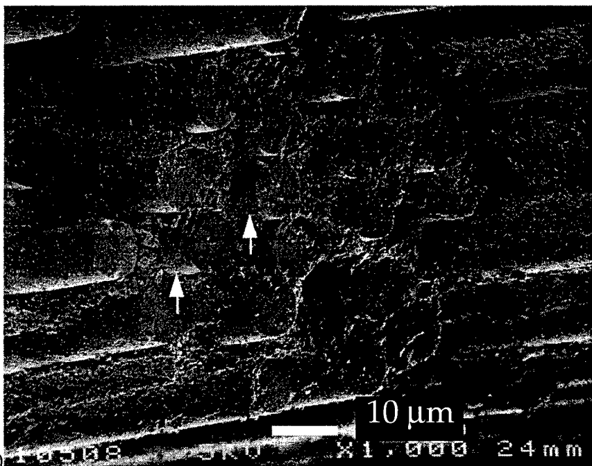
Figure 11. Fracture surface near the tensile surface of a \pm 45^\circ fiber orientation composite containing 70v% cubic ZrO_2 (8m% Y_2O_3 )/30v% mullite sintered at 1250^\circ C for 5 hours in HCl. The composite was tested in the in-plane 3-point bending configuration. Very little fiber pullout is evident for in-plane testing in this fiber orientation. (a) Arrows show where the crack propagated along fibers before cutting across part of the tow of fibers and then continued again along the fibers. (b) Arrows show that fracture of the fibers was not on a common plane but still independently failed fibers although with less disintegration of surrounding matrix.
