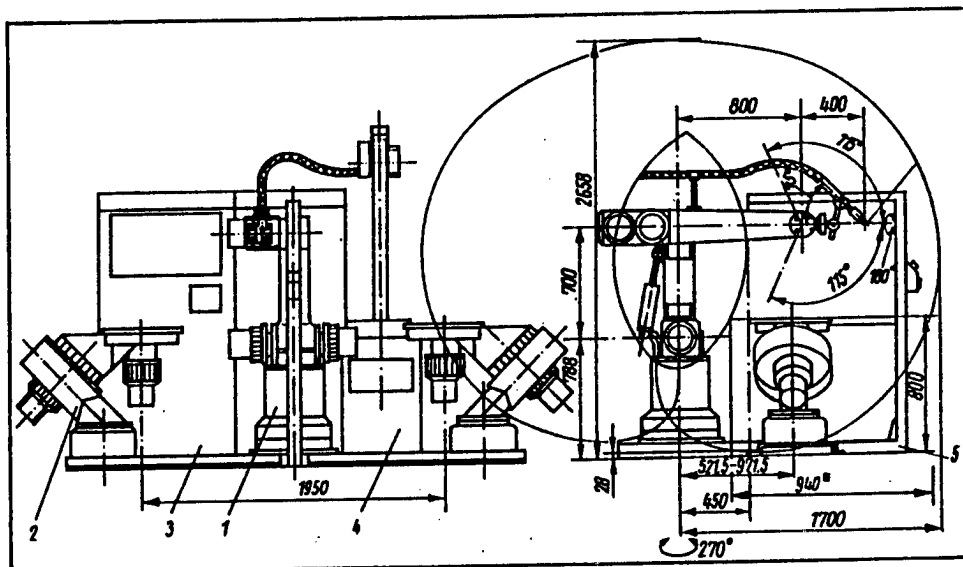
Figure 6. 0J-10 modular robot workstation. (* table surface)
