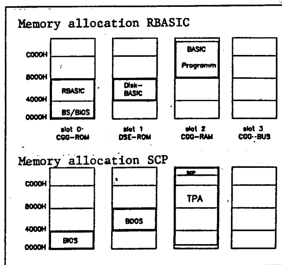
Figure 1. Memory allocations for the A 5105 for RBASIC and SCP.
