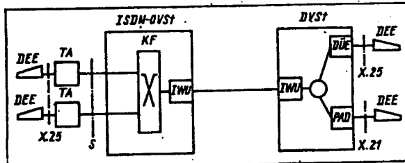
Figure 3. Minimal Integration of Data services in ISDN Local Exchanges Based on CCITT X.31
