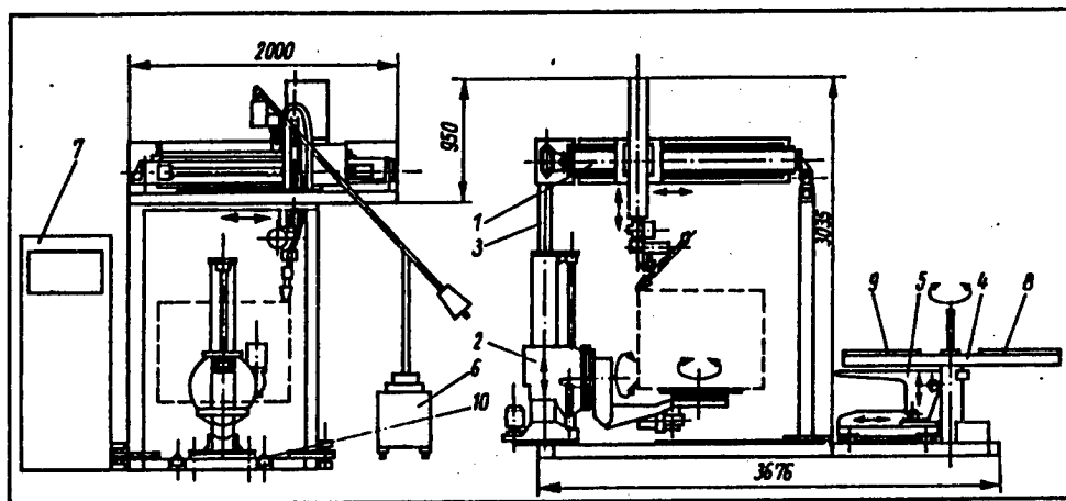
Figure 3. 7RL2 automated welding workstation
