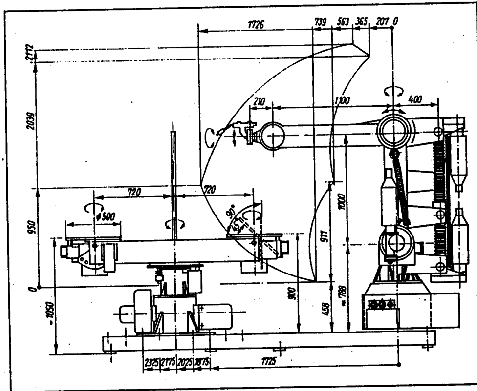
Figure 1. Welding workstation with PR 32 E robot
