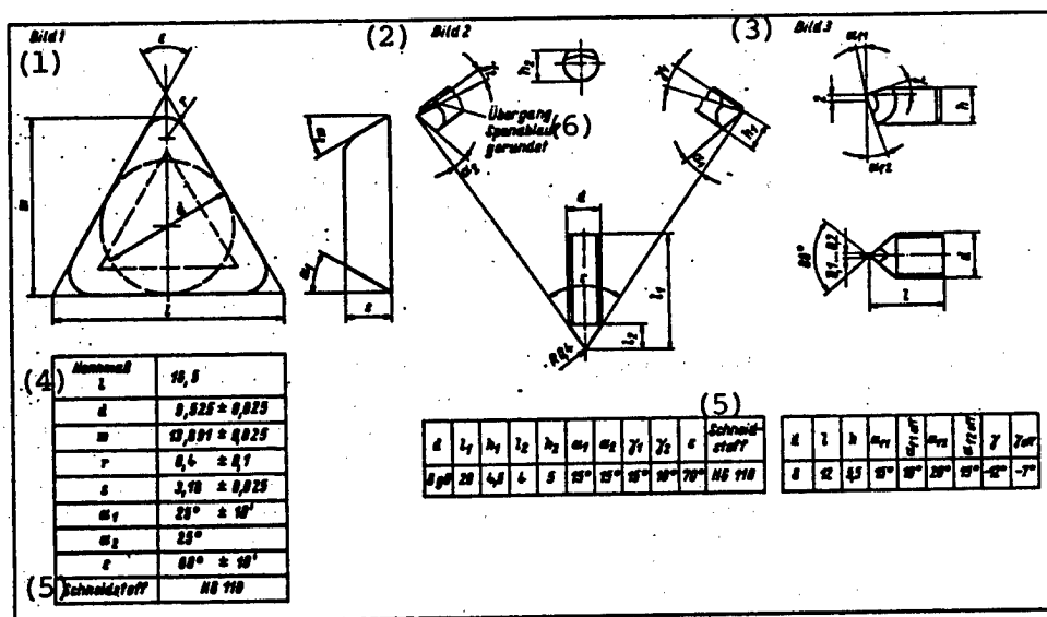
Figures 1-3. Figure 1: Cutting-edge Geometry of the Reversible Carbide Tip for the Turning of Aluminum ("a" less than 2 mm); Figure 2: Cutting Edge Geometry of Carbide-alloy Boring-bar Inserts for the Turning of Aluminum ("a" less than 1.5 mm); Figure 3: Cutting-edge Geometry of the Carbonado Insert PB 0501 for the Inside Turning of Aluminum
