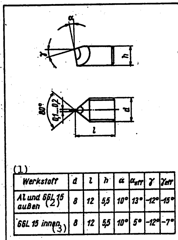
Figure 4. Cutting-edge Geometry of the Carbonado and Composite Insert Key:—1. Machined material—2. Al and GGL 15 outside—3. GGL 15 inside
