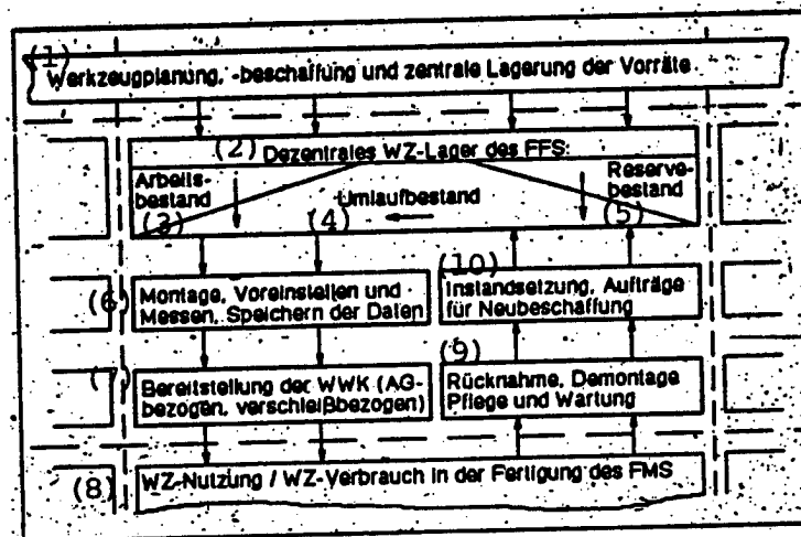
Figure 3. Store and Operational Areas of TTC Ready for FMS's.
