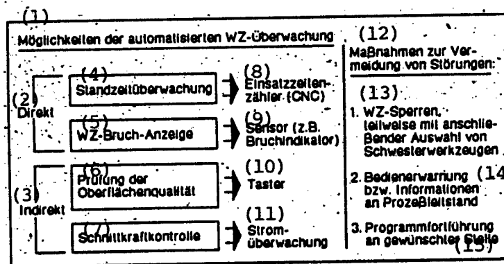
Figure 1. Technical Solutions for the Automated Monitoring of the Serviceability of TTC's.
