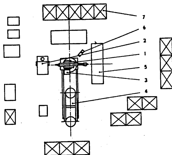
Figure 4. RTP for arc welding at the BSS National Enterprise at Brandys nad Labem:
