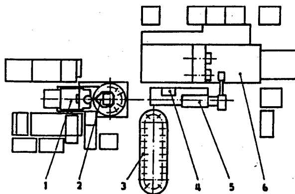
Figure 3. RTK for the production of gear wheels—Model AUCOR-16:
