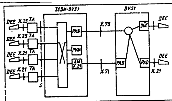
Figure 5. Integration Possibilities for Data Link Terminals Based on X.21 and X.25 in ISDN Local Exchanges
