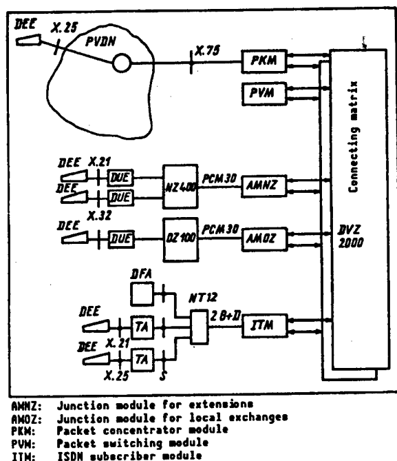
Figure 10. Possibilities for Data Communication in Digital Islands DVZ 2000, OZ 100, NZ 400.
