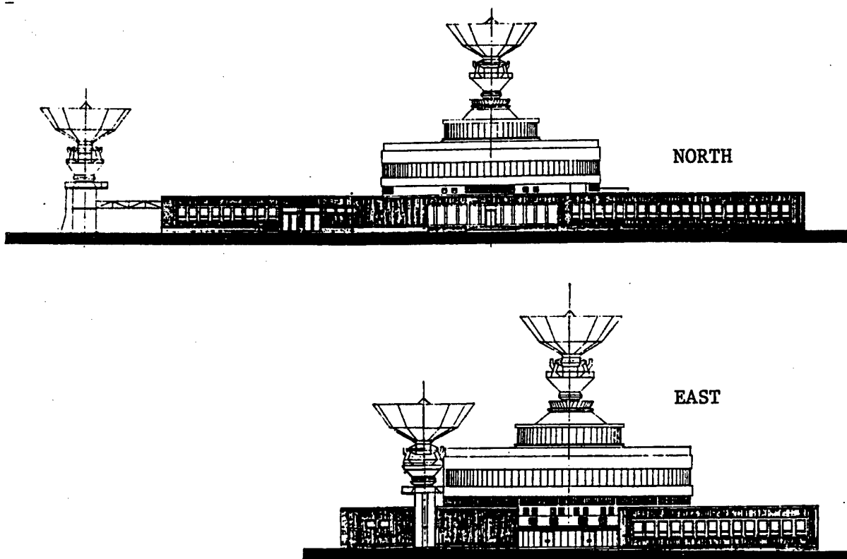
Figure 2. Ground station after completion of second stage of expansion—view from the north and the east.
