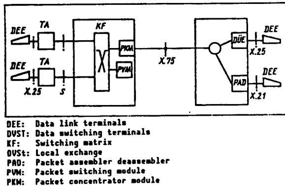
Figure 4. Maximal Integration of Data Services in ISDN Local Exchanges based on CCITT X.31
