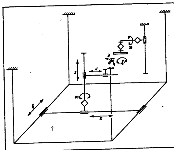
Figure 4. Kinematic view of the 7RL2 robot workstation
