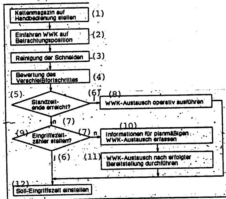
Figure 2. Flow Chart for the Inspection Process
