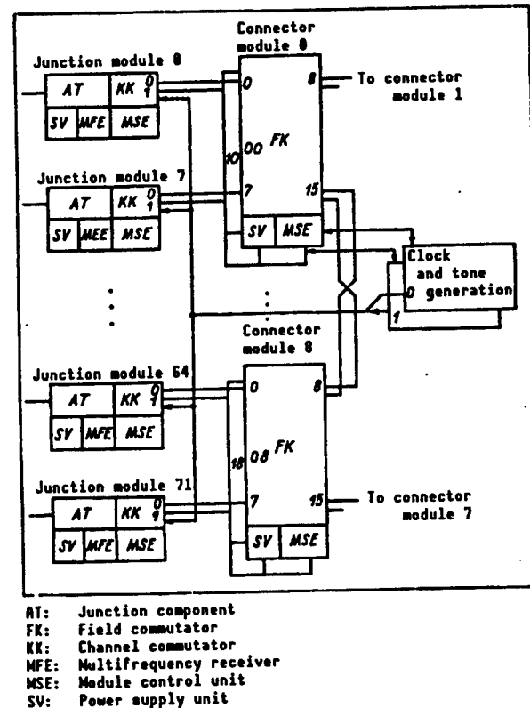
Figure 1. Basic Structure of a Central Exchange for the DVZ 2000 System
