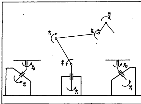
Figure 8. 0J-10 industrial robot
