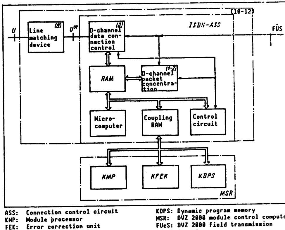
Figure 7. Basic Structure of an ISDN Subscriber Module.
