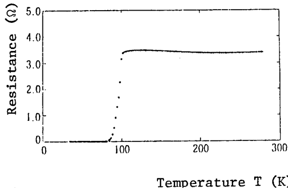
Figure 1. Dependence of Electric Resistance of Y-Ba-Cu-O Thick Film Sample Produced by Spray Pyrolysis Method on Temperature
