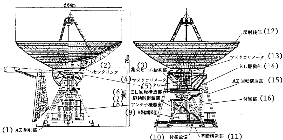
Figure 1. Construction of Deep-Space Exploration Antenna
