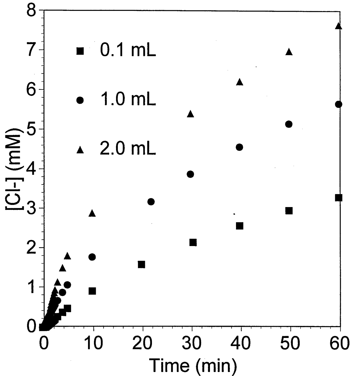
Figure I-2 Chloride production for various amounts of R-11 in 110 mL of Ar-saturated, 0.5 g/L TiO 2 , 0.30 M formate/formic acid buffer, and 7.0 × 10 -5 M(hv)/min.
