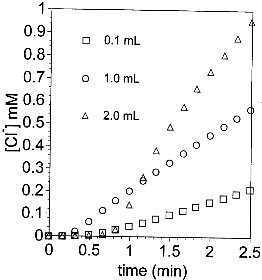
Figure I-3 Chloride production at short times for various amounts of R-11 in 110 mL of Ar-saturated, 0.5 g/L TiO_2 , 0.30 M formate/formic acid buffer, and 7.0 \times 10^{-5} \text{ M}(\text{h}\nu)/\text{min} .
