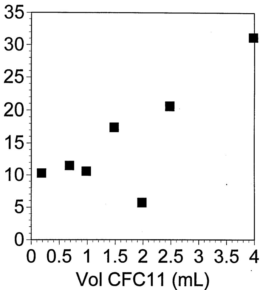
Figure I-10 Photonic efficiencies for the fast step of various amounts of R-11 in 110 mL of air-saturated, 0.5 g/L TiO 2 , 0.30 M formate/formic acid buffer, and 1.8 x 10 -5 M/min
