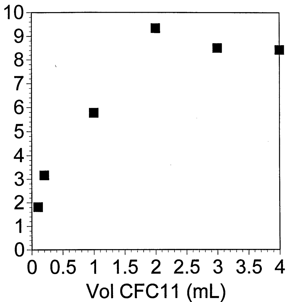
Figure I-4 Photonic efficiencies for the fast step of various amounts of R-11 in 110 mL of Ar-saturated, 0.5 g/L \text{TiO}_2 , 0.30 M formate/formic acid buffer, and 7.0 \times 10^{-5} M(\text{h}\nu)/\text{min}
