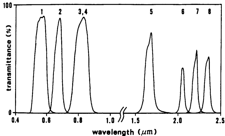
Figure 3. Transmittance curves of the filters installed.
