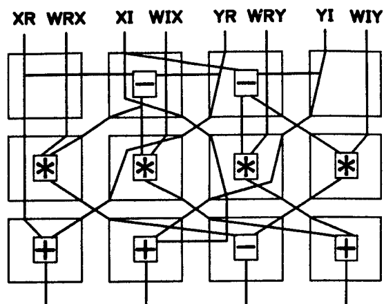
Figure 2-3. Radix-2 Butterfly
