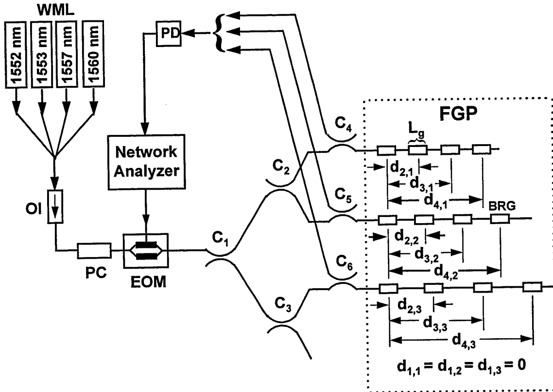
FIGURE 2: EXPERIMENTAL SETUP FOR THE DISCRETE BEAMFORMING SYSTEM.
