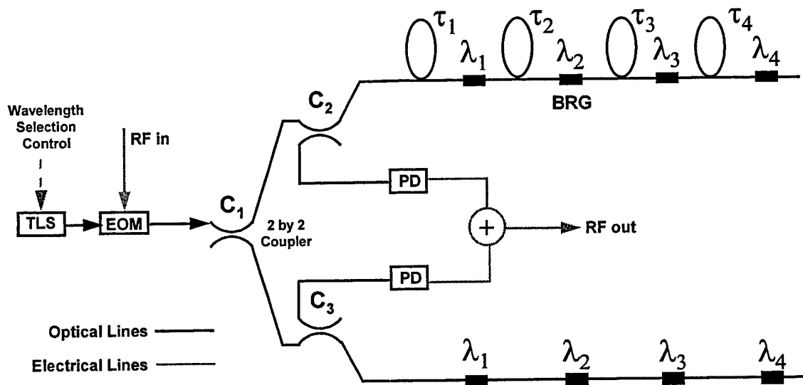
FIGURE 5: TRANSVERSAL NOTCH FILTER
