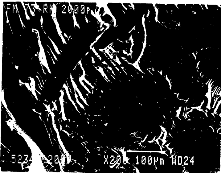
Fig. 3.5: SEM photographs of the surface failure morphology of SLS joints after 10 days in humidity chamber. Adhesive FM73, primer A187. Laser energy 180mj/p*cm 2 , 2000pulses).
