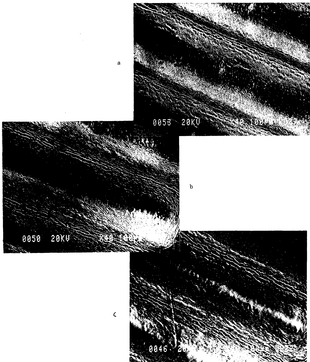
Fig. 3.12 : SEM photograph of Al surface: a)after irradiation with 2.7 \text{ J/p} \cdot \text{cm}^2 , 10 pulses, b)after after irradiation with 2.7 \text{ J/p} \cdot \text{cm}^2 , 50 pulses, c) after after irradiation with 2.7 \text{ J/p} \cdot \text{cm}^2 , 100 pulses.
