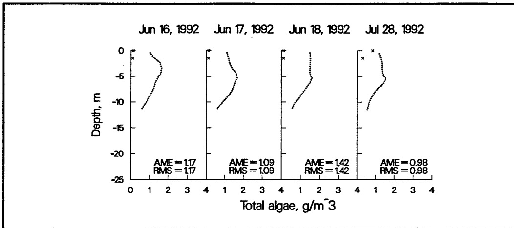
Figure 32. 1992 computed versus observed algae at station 3
