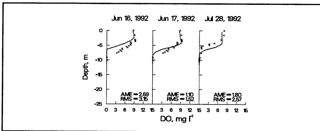
Figure 29. 1992 computed versus observed DO at station 35
