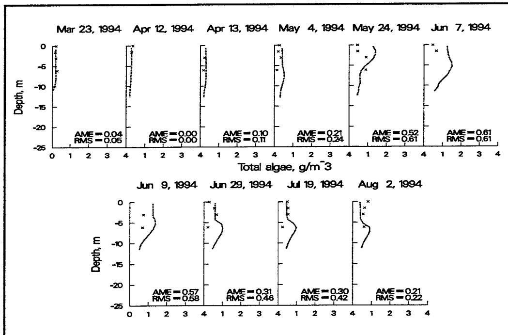
Figure 22. 1994 computed versus observed algae at station 3
