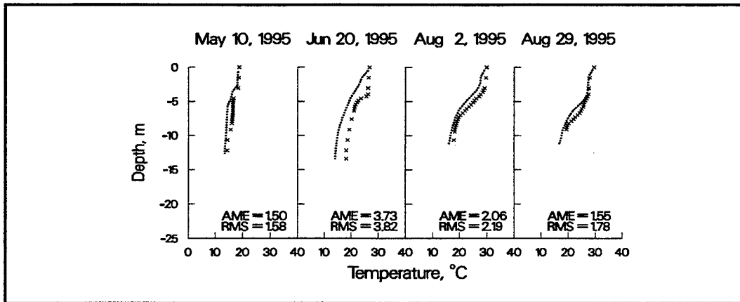
Figure 36. 1995 computed versus observed temperature at station 3
