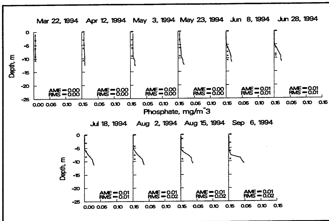
Figure 13. 1994 computed versus observed phosphorus at station 3
