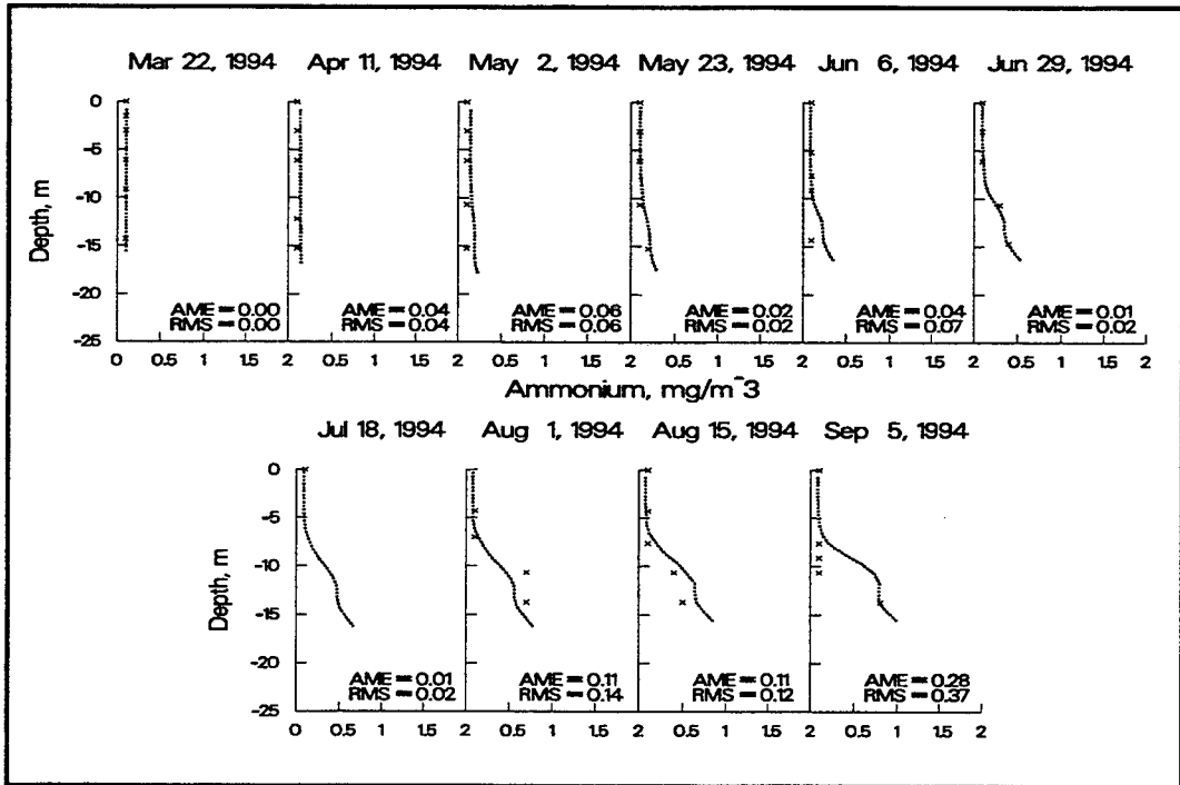
Figure 14. 1994 computed versus observed ammonium at station 1
