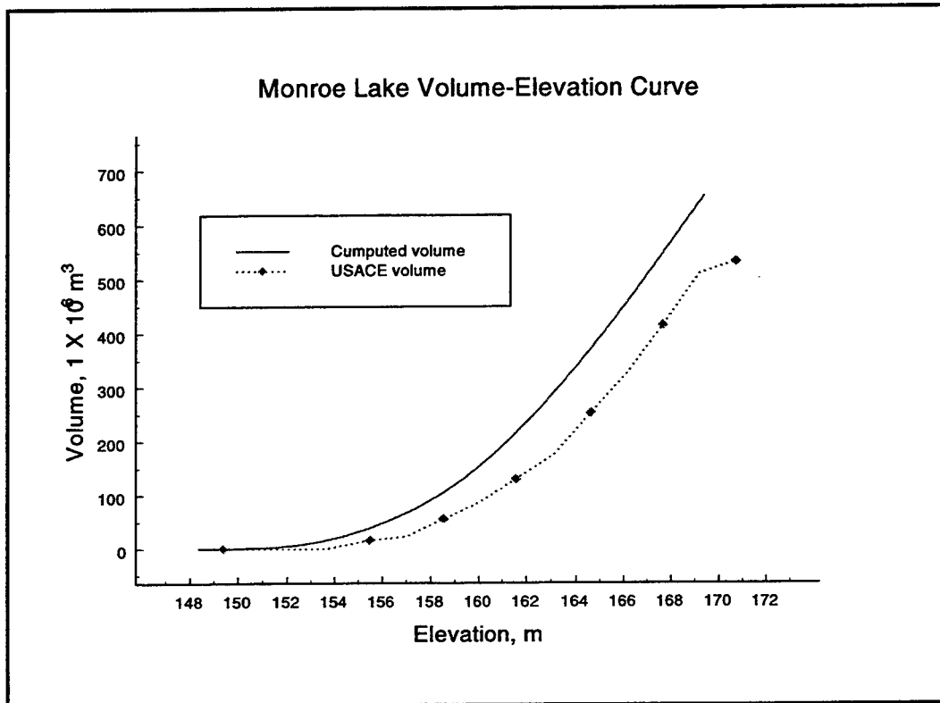
Figure 3. 1994 Lake Monroe volume-elevation curve
