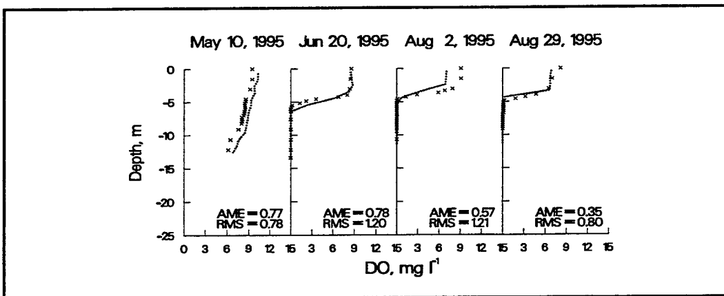
Figure 39. 1995 computed versus observed DO at station 3
