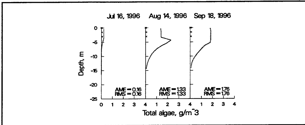
Figure 51. 1996 computed versus observed algae at station 35
