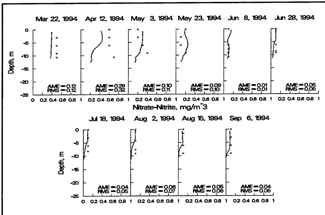
Figure 19. 1994 computed versus observed nitrate-nitrite at station 3
