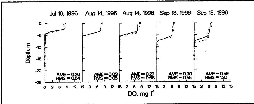
Figure 47. 1996 computed versus observed DO at station 1
