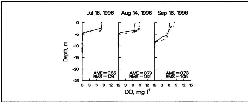
Figure 49. 1996 computed versus observed DO at station 3
