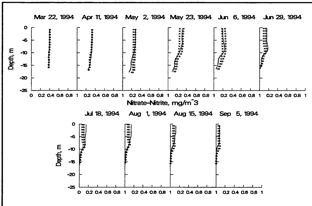
Figure 70. Nitrate-nitrite results for base run (....), scenario 5 (xxx) and scenario 6 (ooo)
