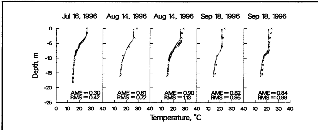
Figure 44. 1996 computed versus observed temperature at station 35
