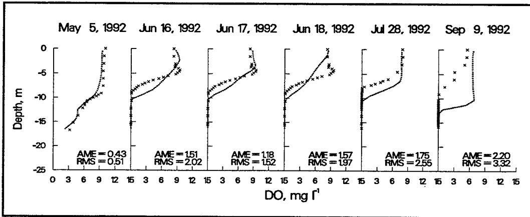
Figure 27. 1992 computed versus observed DO at station 3
