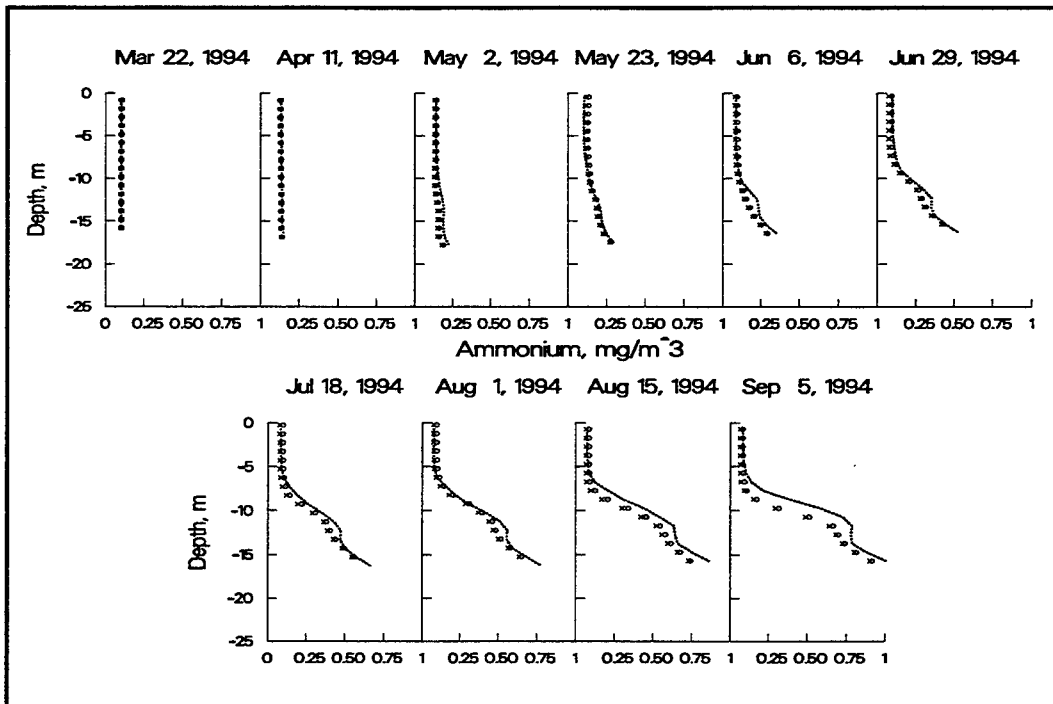
Figure 69. Ammonium results for base run (....), scenario 5 (xxx) and scenario 6 (ooo)
