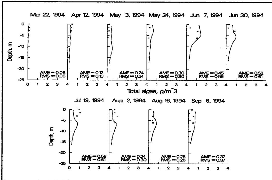
Figure 20. 1994 computed versus observed algae at station 1
