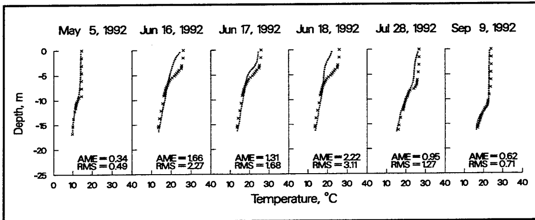
Figure 24. 1992 computed versus observed temperatures at station 1
