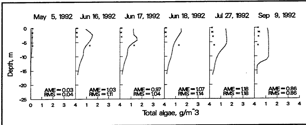
Figure 30. 1992 computed versus observed algae at station 1
