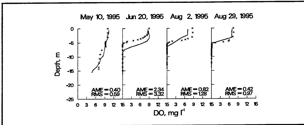
Figure 38. 1995 computed versus observed DO at station 35
