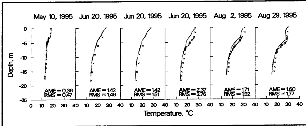
Figure 34. 1995 computed versus observed temperature at station 1
