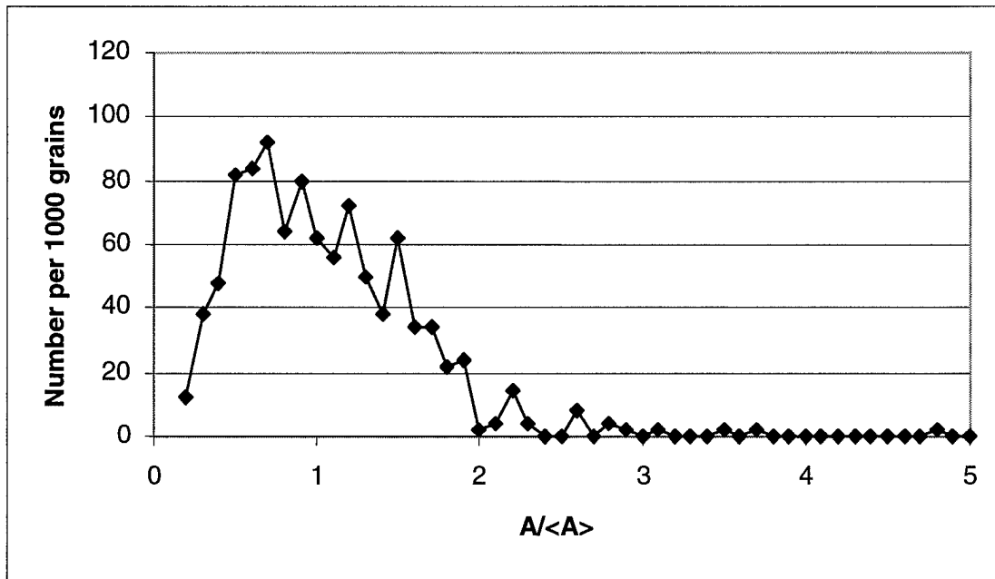
Figure 3-7. Normalized Grain Area Distribution of 500 Grains.
