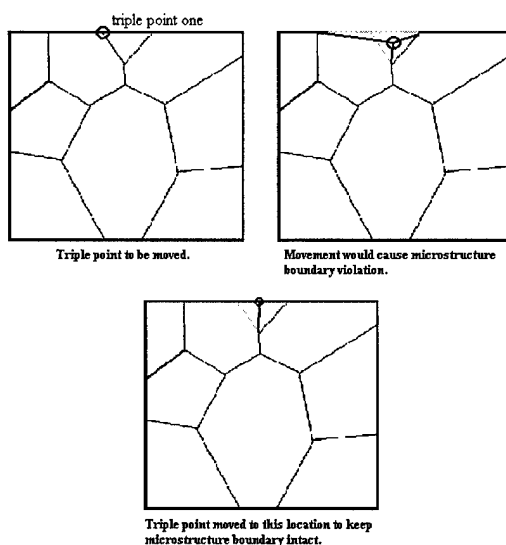
Figure 2-24. Example of Correcting a Triple Point that Lies on the Microstructure Boundary for the Three-sided Grain Removal Process.
