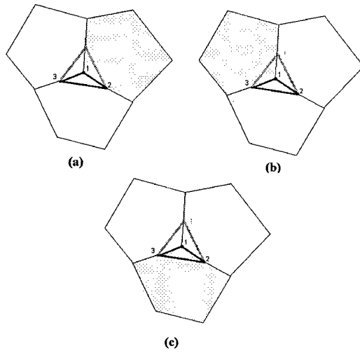
Figure 2-25. Triple Point Cases for Three-sided Grain Removal.
