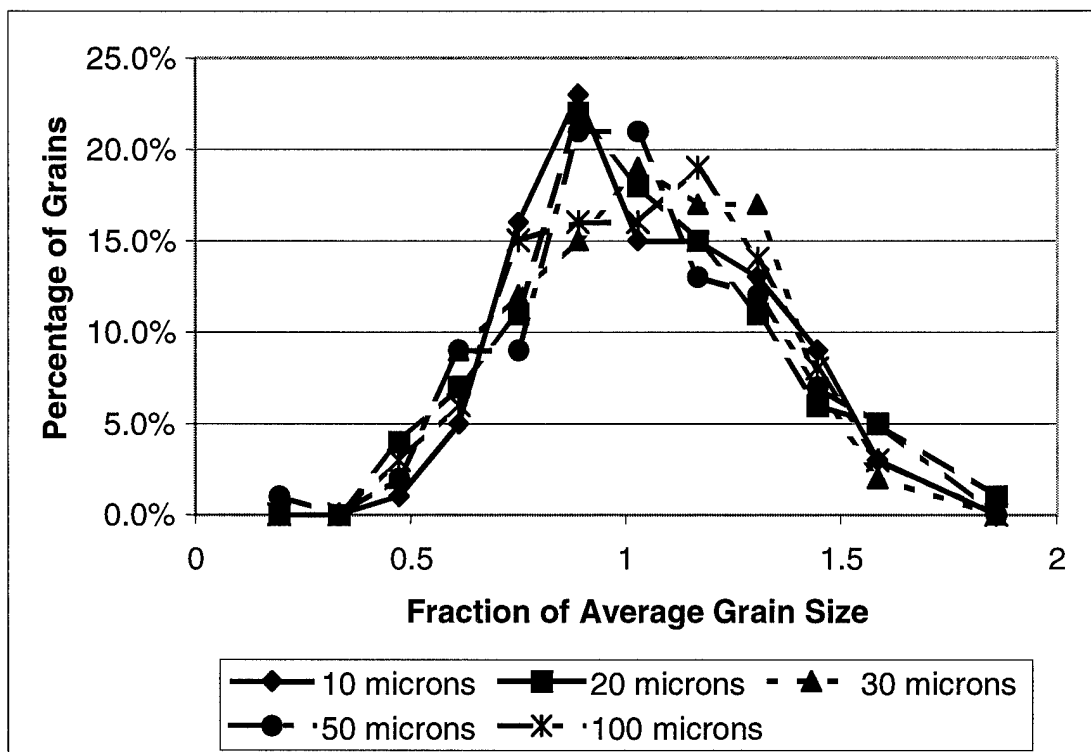
Figure 3-4. Grain Size Distributions for Different Average Grain Sizes.
