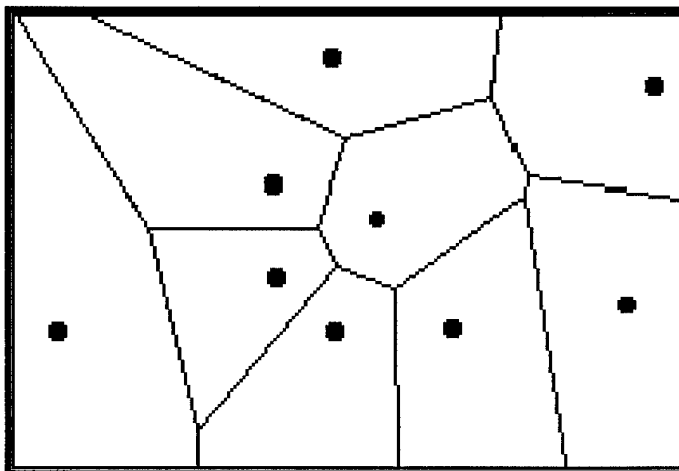
Figure 2-1. Voronoi Diagram.
