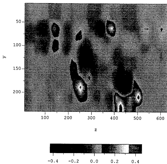
Figure 3-31: \omega_x , \alpha = 30^\circ , x/c = 0.3 , Leeward Side Vortex
