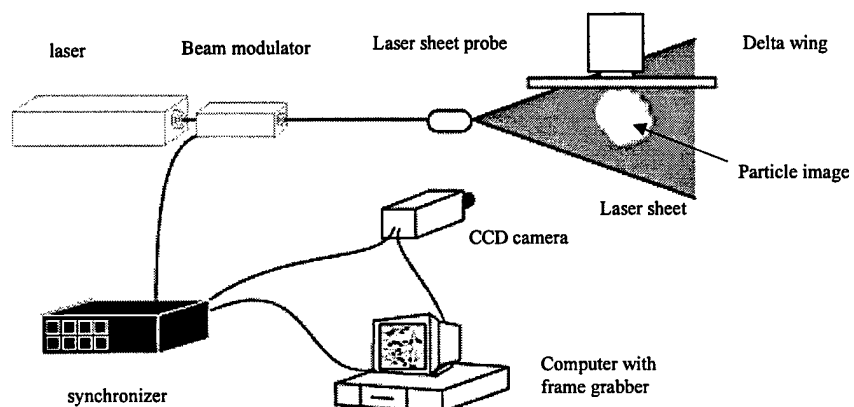
Figure 2-5: Particle Image Velocimetry Set-up
