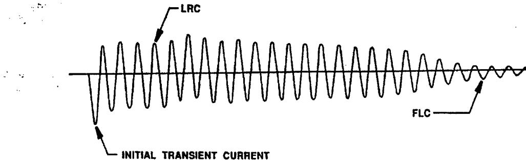
Fig 4.1. One Phase Trace of Motor Starting Current [Heberlein 1989]
