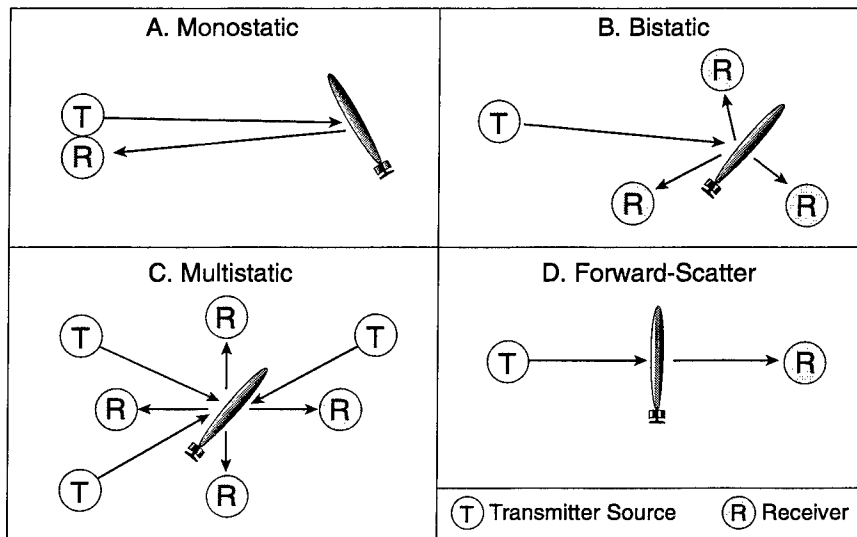
FIGURE 1.2 Basic transmitter and receiver configurations for four different active acoustic concepts: (A) monostatic, (B) bistatic, (C) multistatic, and (D) forward scatter.
