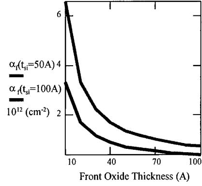
Figure 9. Calculated dependence of \alpha_f on t_{si} and t_{ox} . t_{box} = 5000 \text{ Å} .
