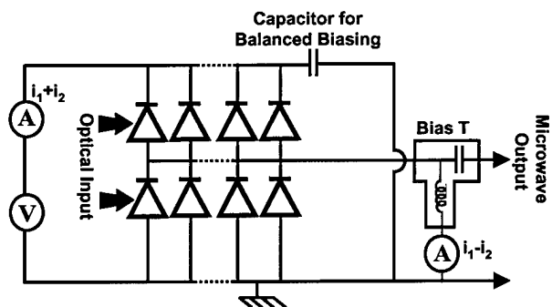
Figure 8. The biasing circuit for balanced detection.
