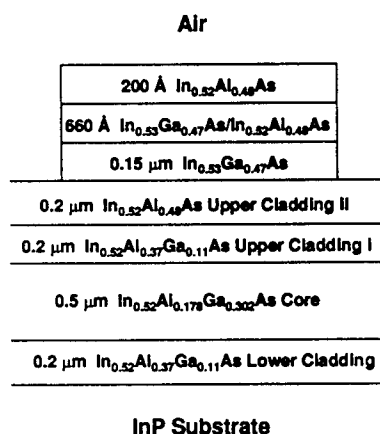
Figure 3. Cross section of VMDP wafer after mesa etching
