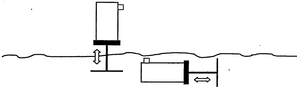
Figure 5.4. Typical actuator placement for vertical and shear wave excitation.
