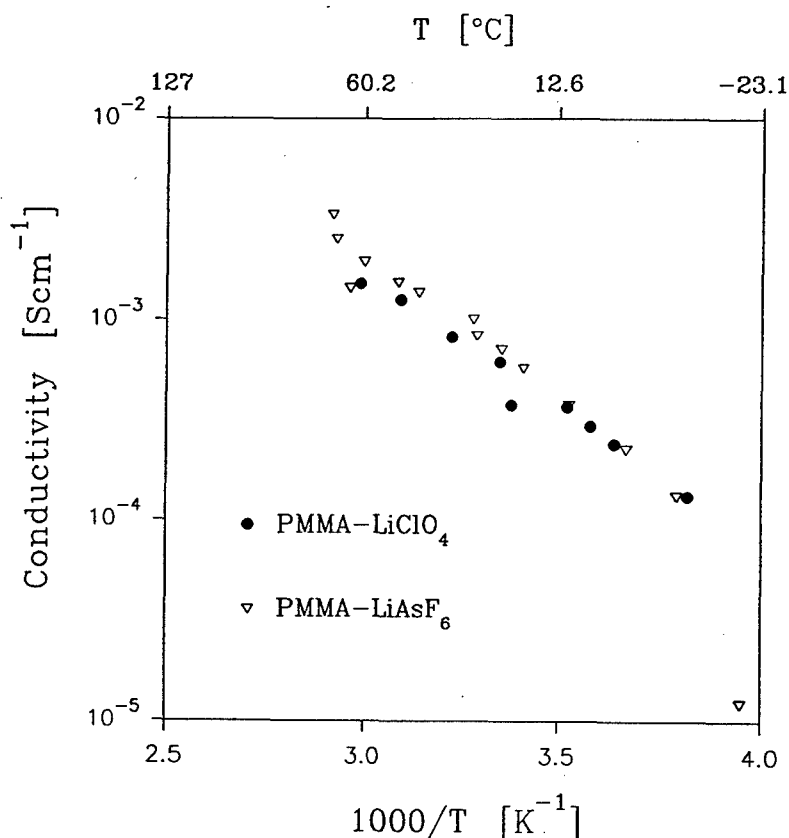
Figure1- Arrhenius plot of the PMMA-PC/EC- \text{LiClO}_4 (sample S-1) and of the PMMA-PC/EC- \text{LiAsF}_6 (sample S-2) electrolytes.
