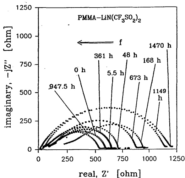
Figure 3- Time evolution of the impedance of a Li/PMMA-PC/EC LiN(CF 3 SO 2 ) 2 (sample S-3)Li cell stored continuously under open circuit conditions at room temperature. The number of progressive hours of storage is indicated in the figure.
