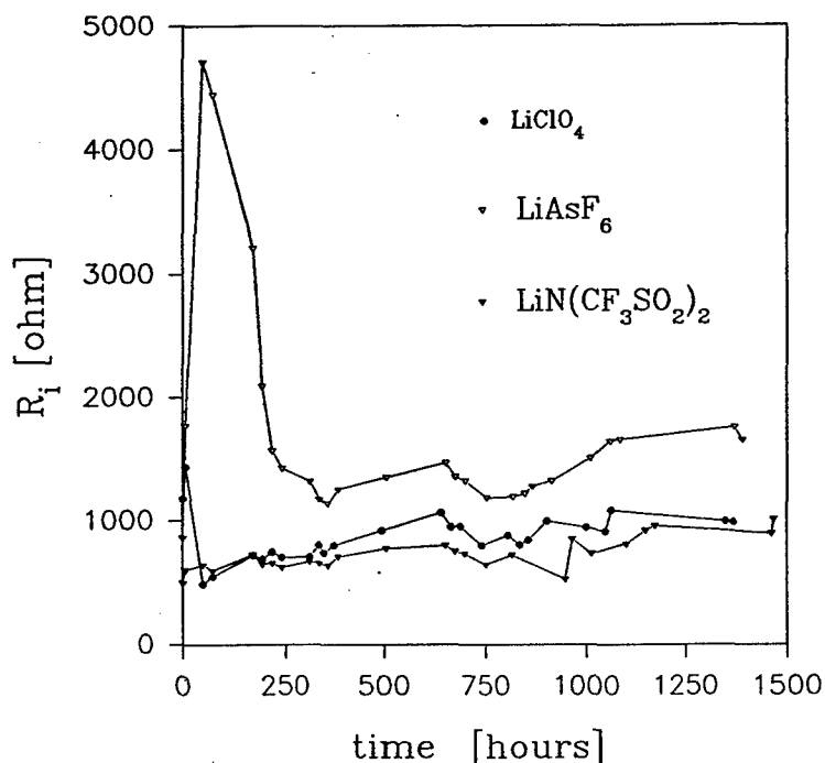
Figure 4 - Time evolution at 25 °C of the interfacial resistance R_i of the lithium electrode in the LiClO 4 , EC/PC-PMMA, (sample S-1) LiAsF 6 , EC/PC-PMMA (sample S-2) and LiN(CF 3 SO 2 ) 2 , EC/PC-PMMA (sample S-3) gel electrolytes under the conditions described in figures 1, 2, and 3, respectively.
