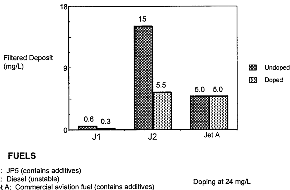
Figure 1. Effect of C 60 on the thermal stability of fuels determined by using a gravimetric JFTOT [4].
